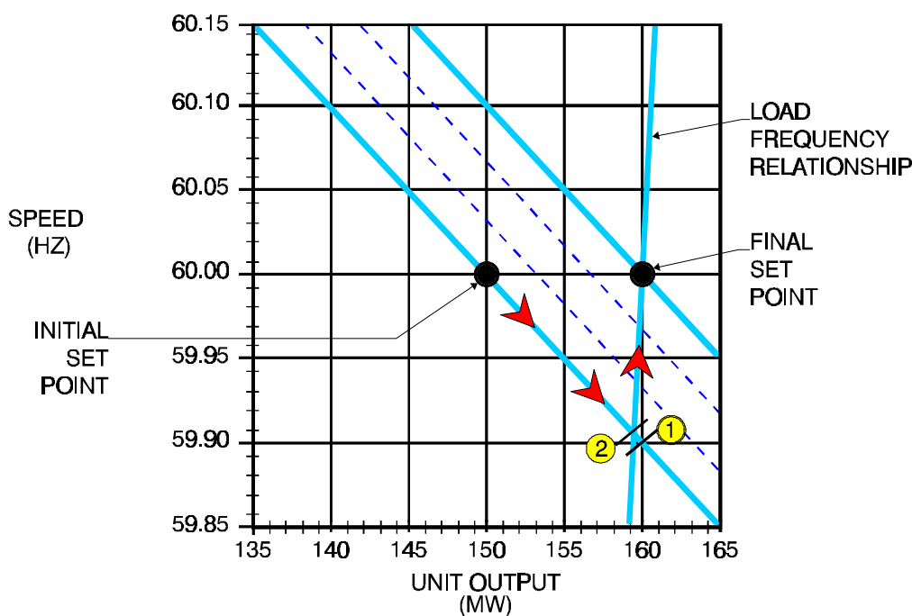
Figure 4-19 Load/Frequency Relationship & Droop Curves
