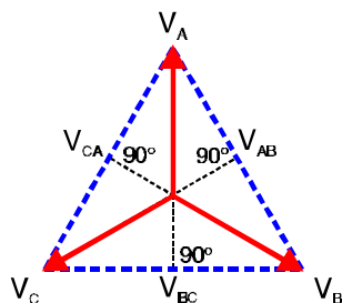
Figure 10-27 Phase in a PST
