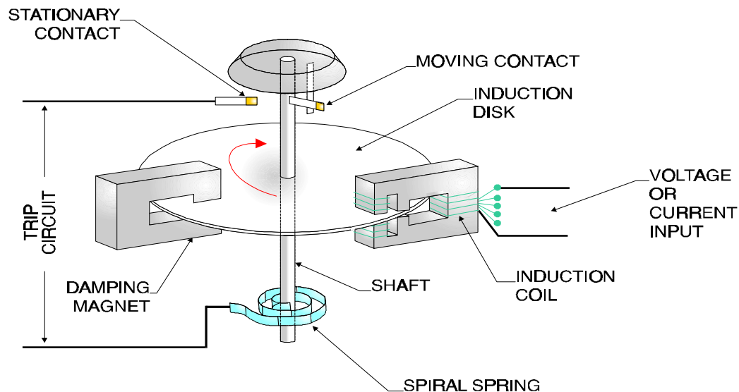
Figure 2-35 Induction Disc Relay Element
