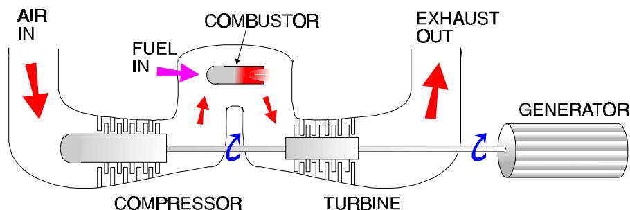
Figure 2-64 Basic Combustion Turbine
