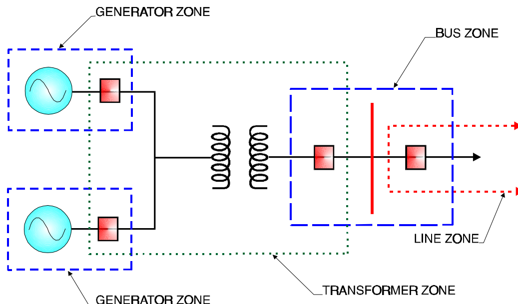
Figure 2-40 Zones of Protection
