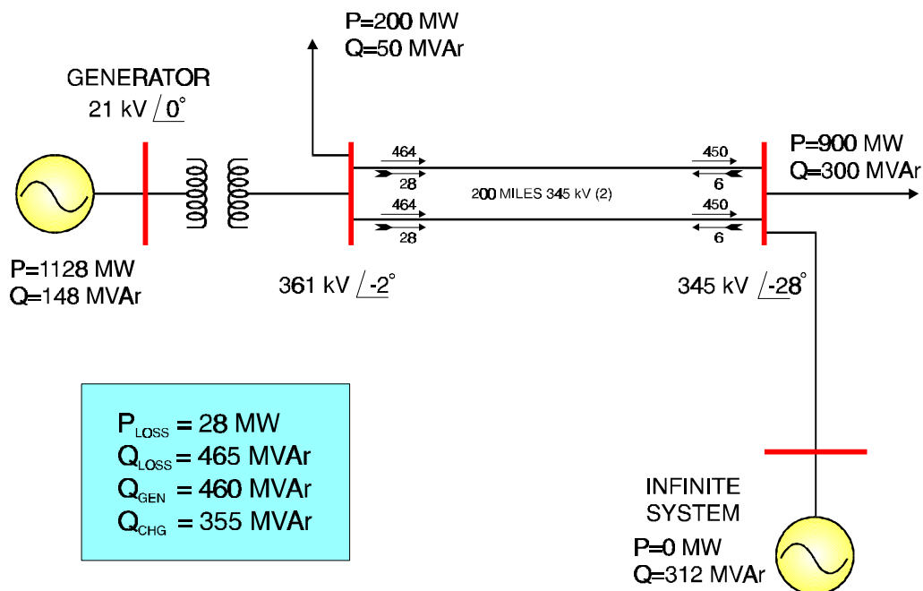
Figure 5-10 Reactive Power & Line Outages - Normal System
