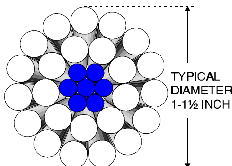
Figure 2-72 ACSR Conductor Cross Section
