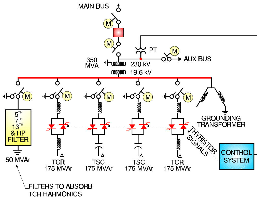
Figure 9-5 Static VAr Compensator
