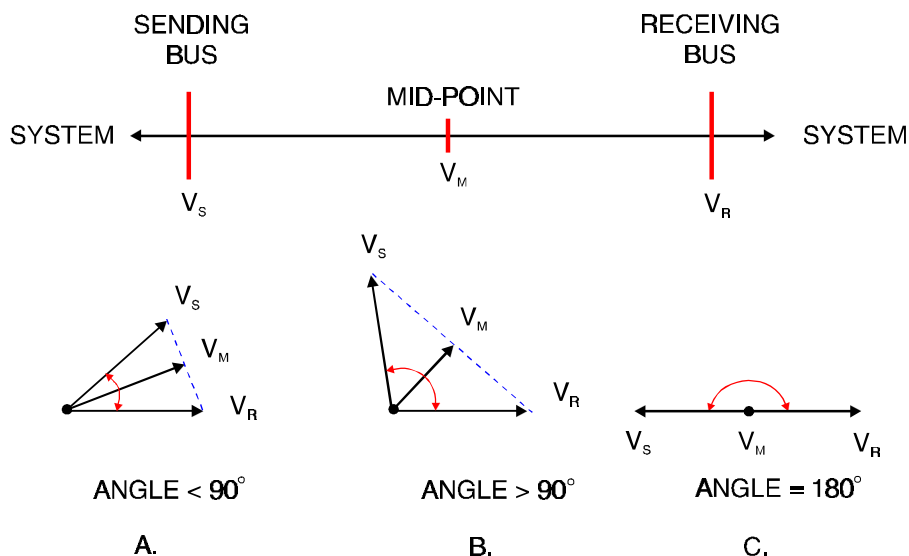
Figure 6-23 Voltage Collapse Due to a Loss of Synchronism
