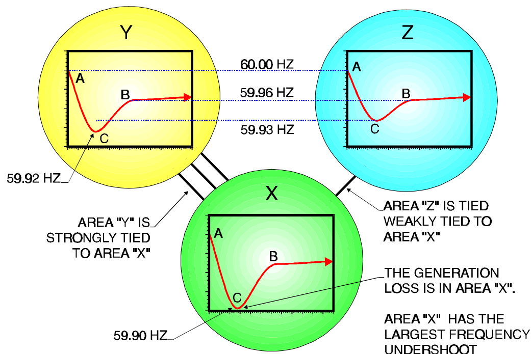
Figure 4-51 Illustration of Frequency Undershoots
