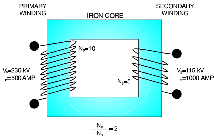
Figure 2-68 Transformer Turns Ratio
