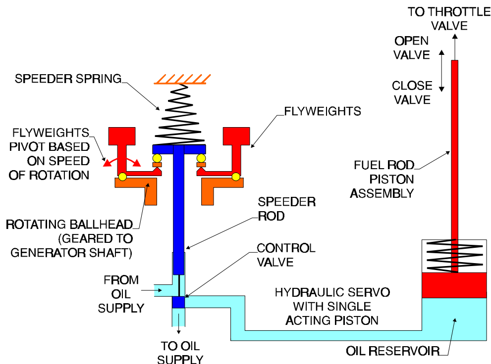
Figure 4-10 Basic Centrifugal Ballhead Governor
