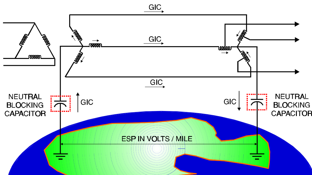
Figure 9-43 Using Neutral Blocking Capacitors
