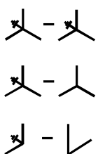
Figure 9-27 Preventing Distribution Ferroresonance
