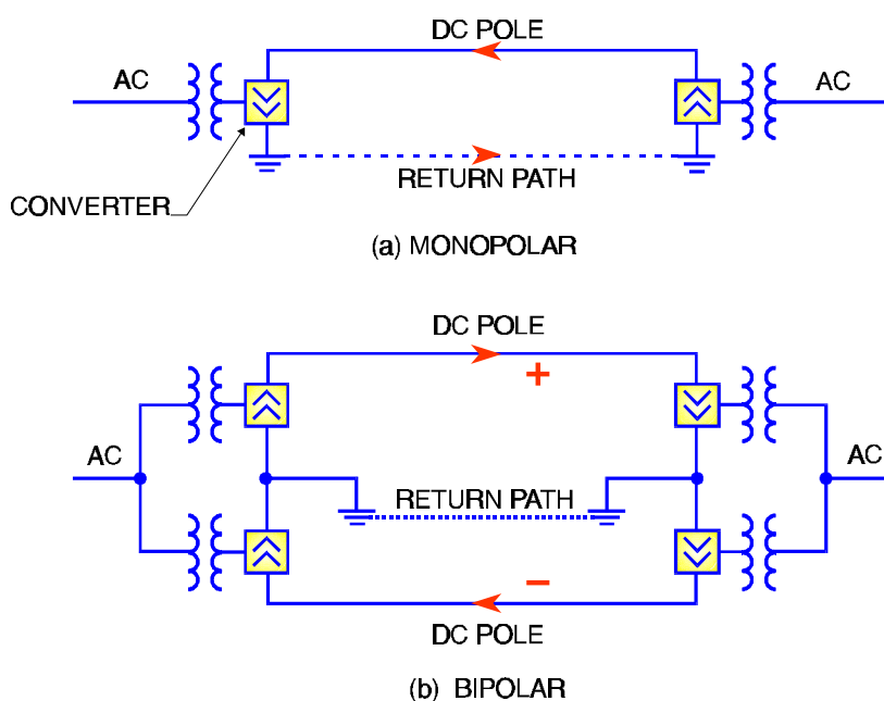
Figure 10-3 Types of HVDC Systems
