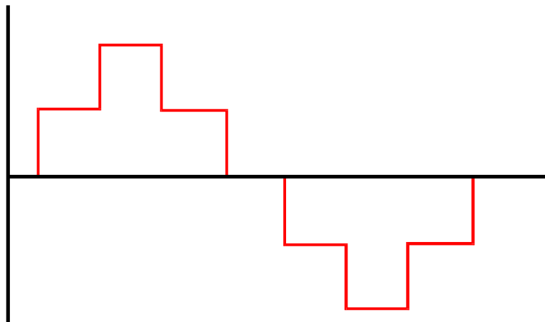
Figure 9-4 Sum of Fundamental, 5th, 7th, 11th, 13th, 17th, 19th, 23rd, & 25th
