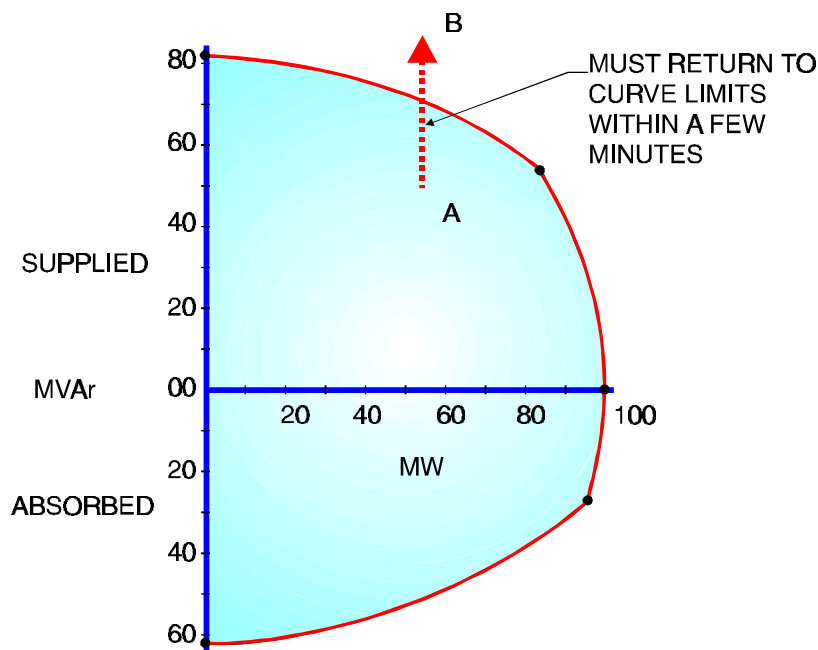
Figure 6-17 Temporary Reactive Power Boost
