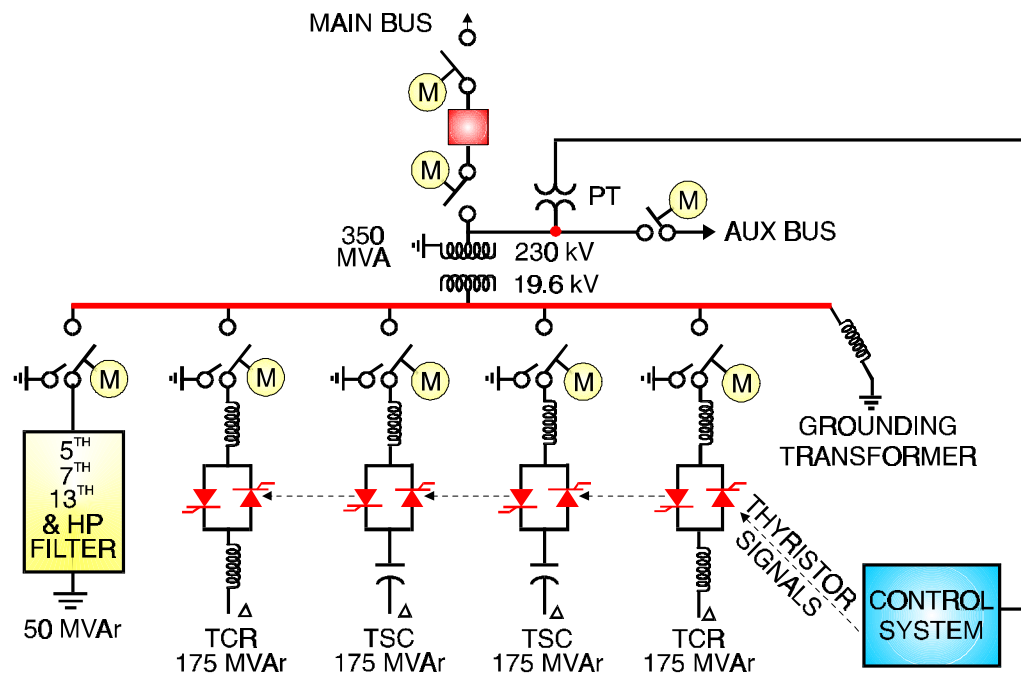
Figure 5-44 Static Var Compensator
