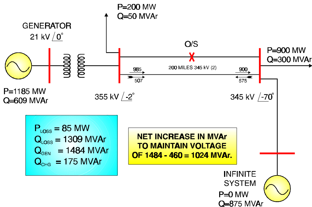
Figure 5-11 Reactive Power & Line Outages - Line Outage
