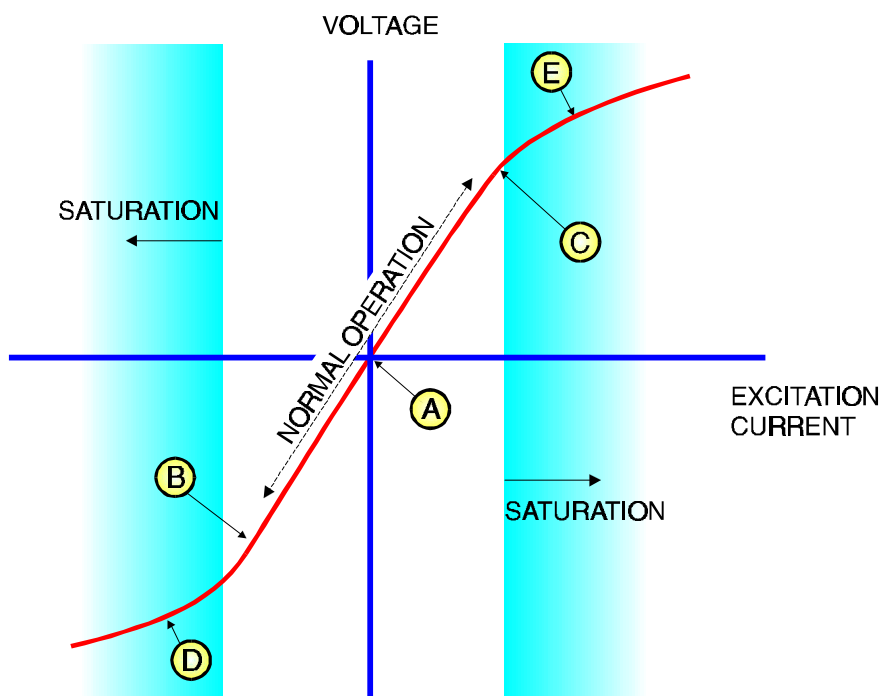
Figure 9-41 Transformer Saturation Curve
