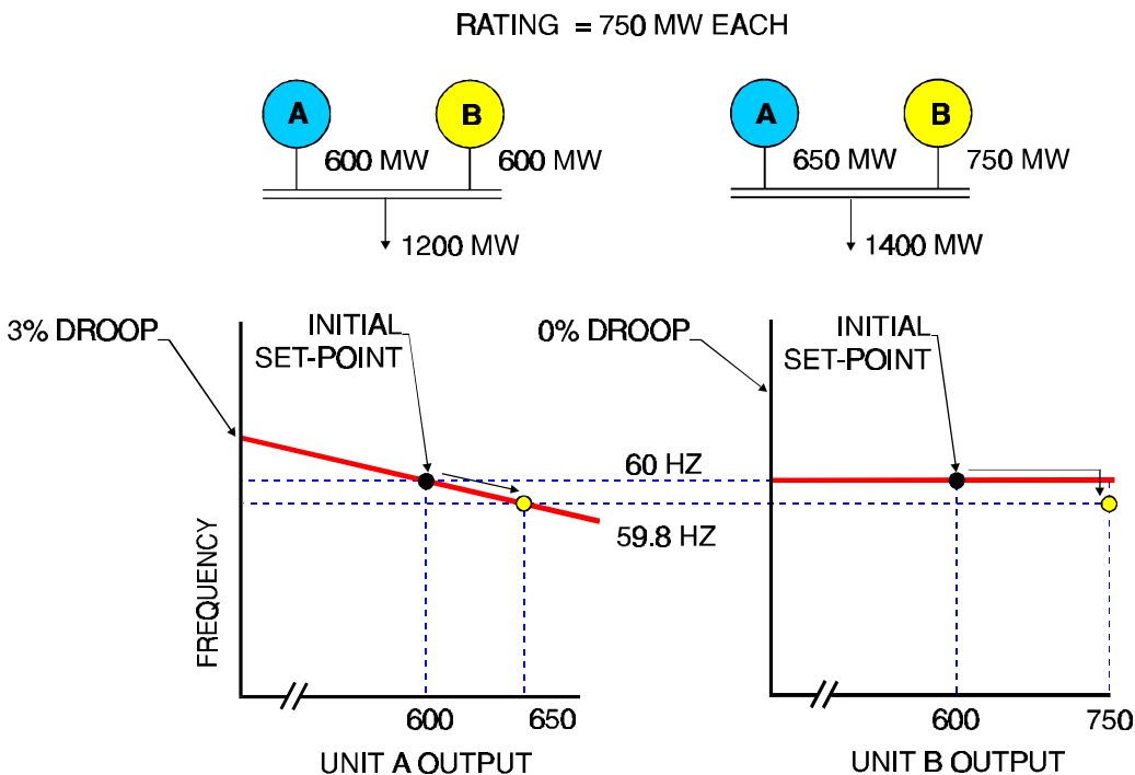
Figure 4-25 Load Sharing - Same Unit Ratings - One In Isochronous
