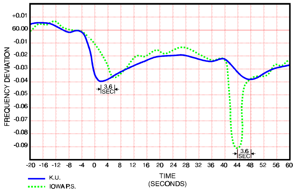
Figure 4-53 Speed of the Traveling Frequency Wave
