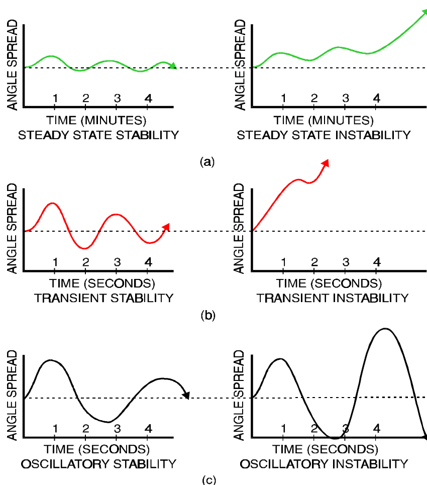
Figure 7-8 Types of Stability / Instability
