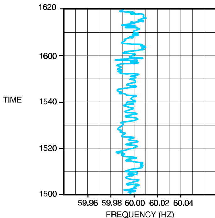
Figure 4-5 Normal Frequency Deviations
