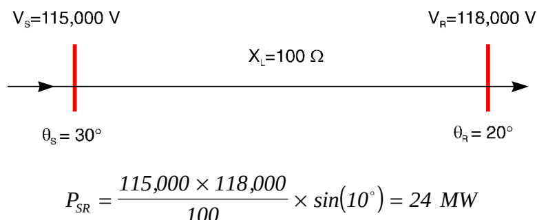
Figure 3-14 Use of the Active Power Transfer Equation
