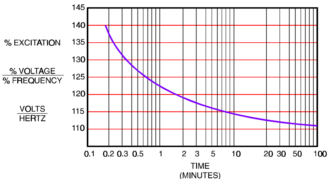
Figure 5-29 Transformer Over-Excitation
