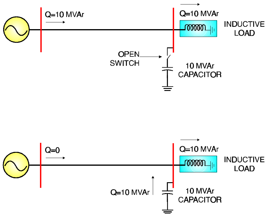
Figure 5-3 Use of a Capacitor
