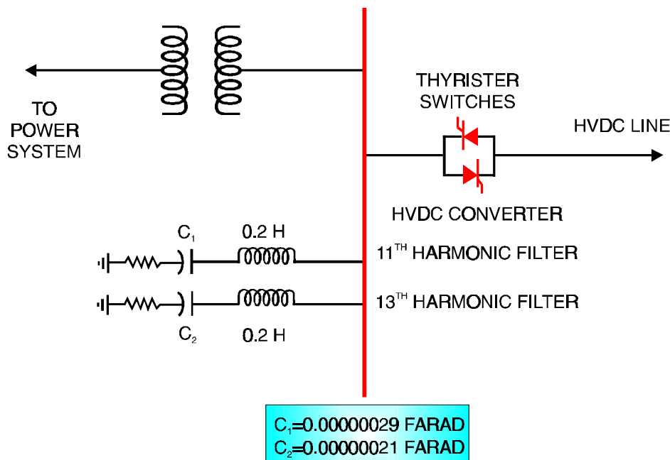
Figure 9-9 Sample Tuning of a Filter
