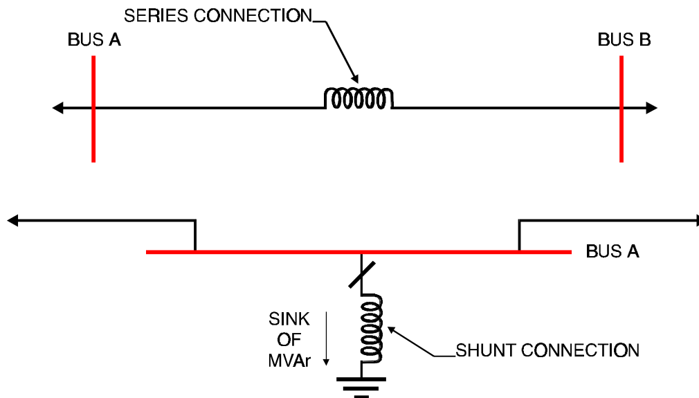
Figure 5-33 Shunt and Series Reactors
