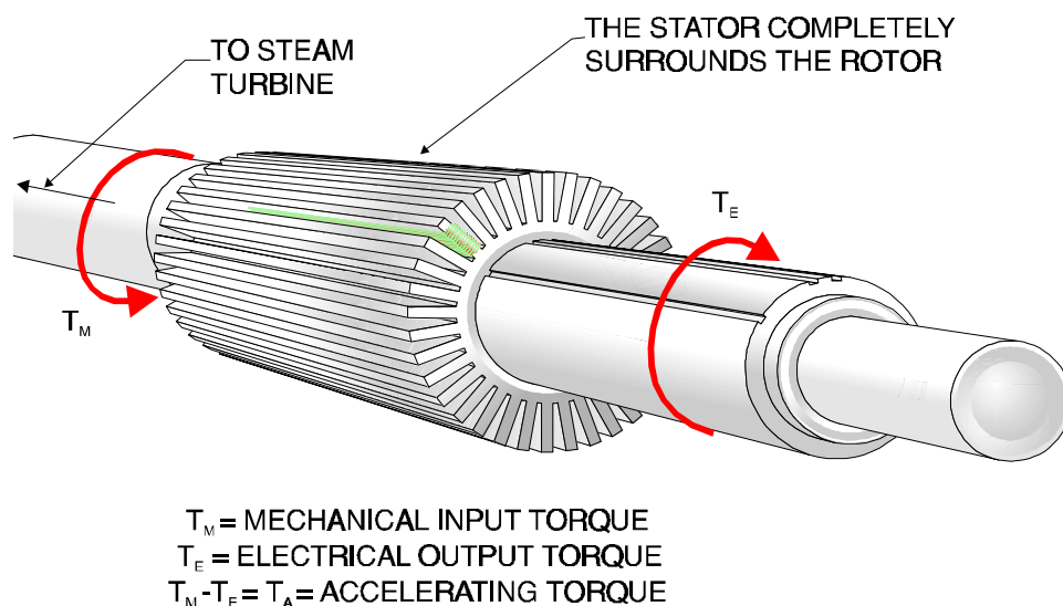
Figure 7-5 Rotor Torques
