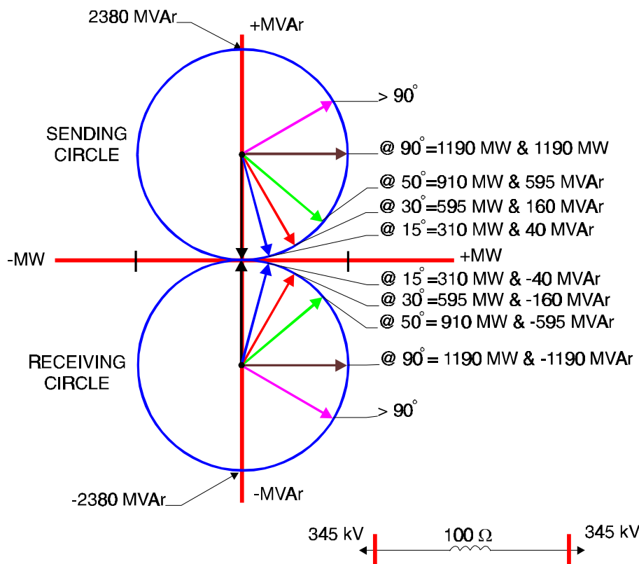
Figure 7-10 Power-Circle Diagram & Steady State Instability
