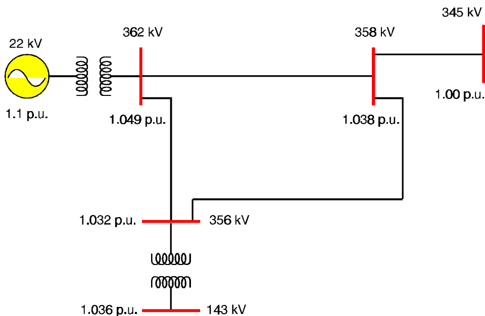
Figure 2-6 Per-Unit System
