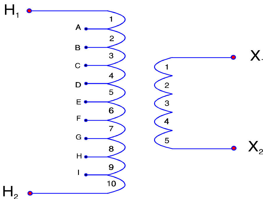
Figure 5-34 Illustration of a Tap Change
