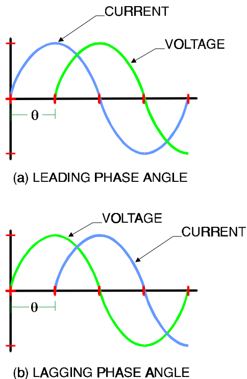
Figure 2-25 Phase Angles in AC Circuits
