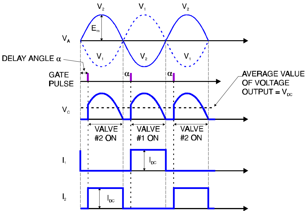
Figure 10-20 Two-Pulse Converter Operation with Gate Control
