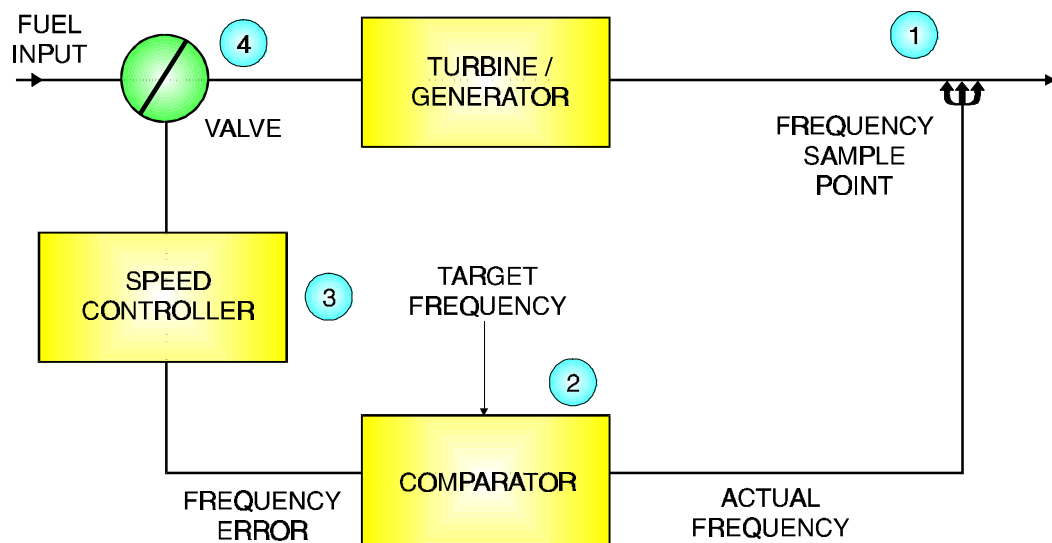
Figure 4-2 Simple Frequency Control System
