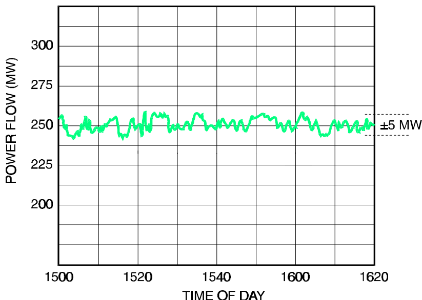
Figure 8-3 Three-Phase Power Flow on a Strip-Chart
