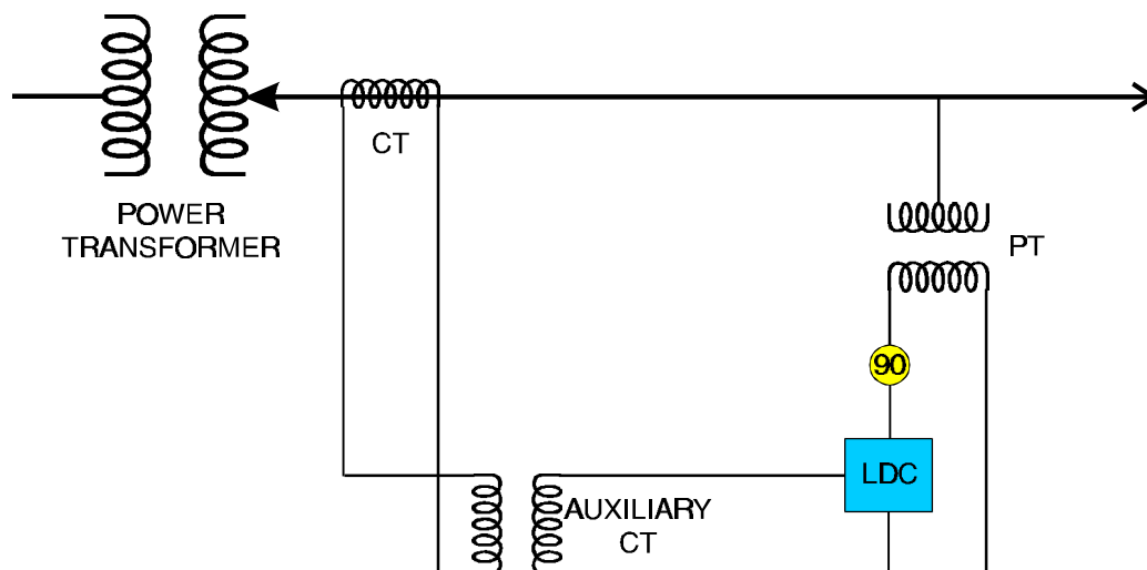
Figure 5-36 A ULTC Control Scheme
