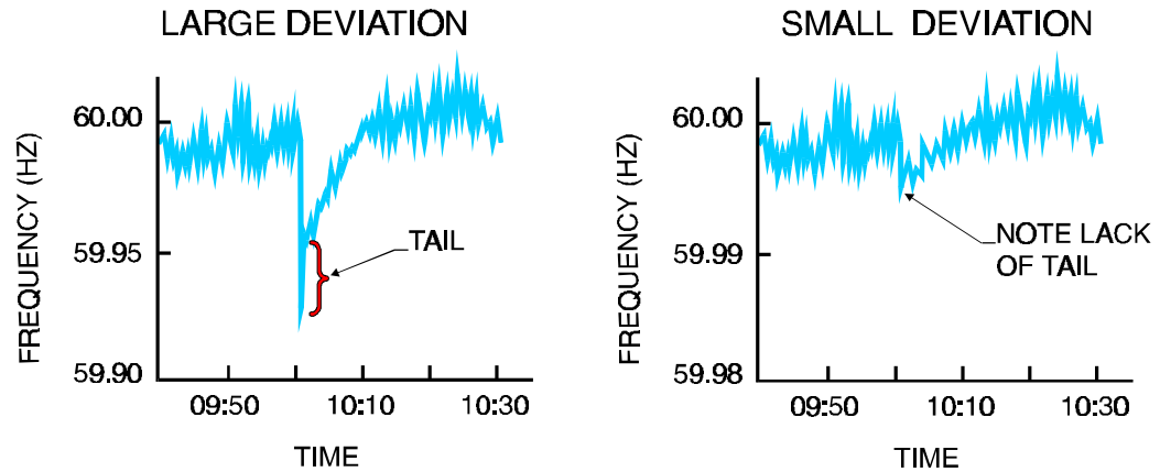
Figure 4-22 Comparison of Large & Small Frequency Deviations
