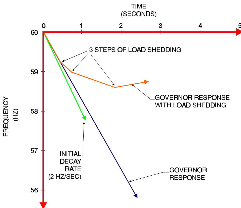
Figure 4-47 UF Load Shedding & Governor Response
