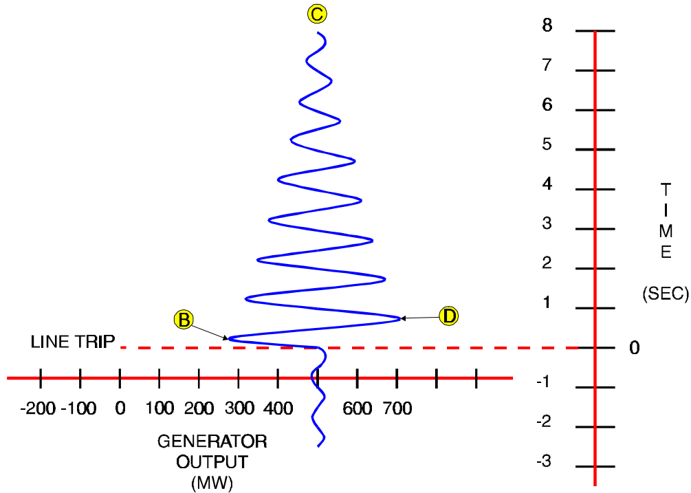
Figure 7-23 Strip Chart Illustration of Oscillatory Stability
