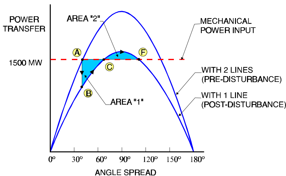
Figure 7-15 Power Angle Curve for Transient Instability
