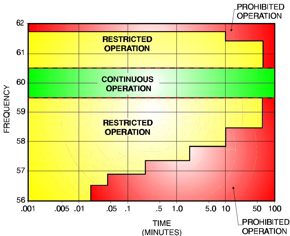
Figure 4-45 Steam Turbine Off-Frequency Limits
