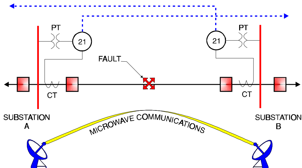
Figure 2-49 Simple Pilot Scheme
