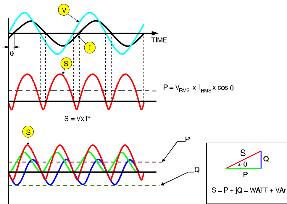
Figure 5-1 Active, Reactive and Complex Power
