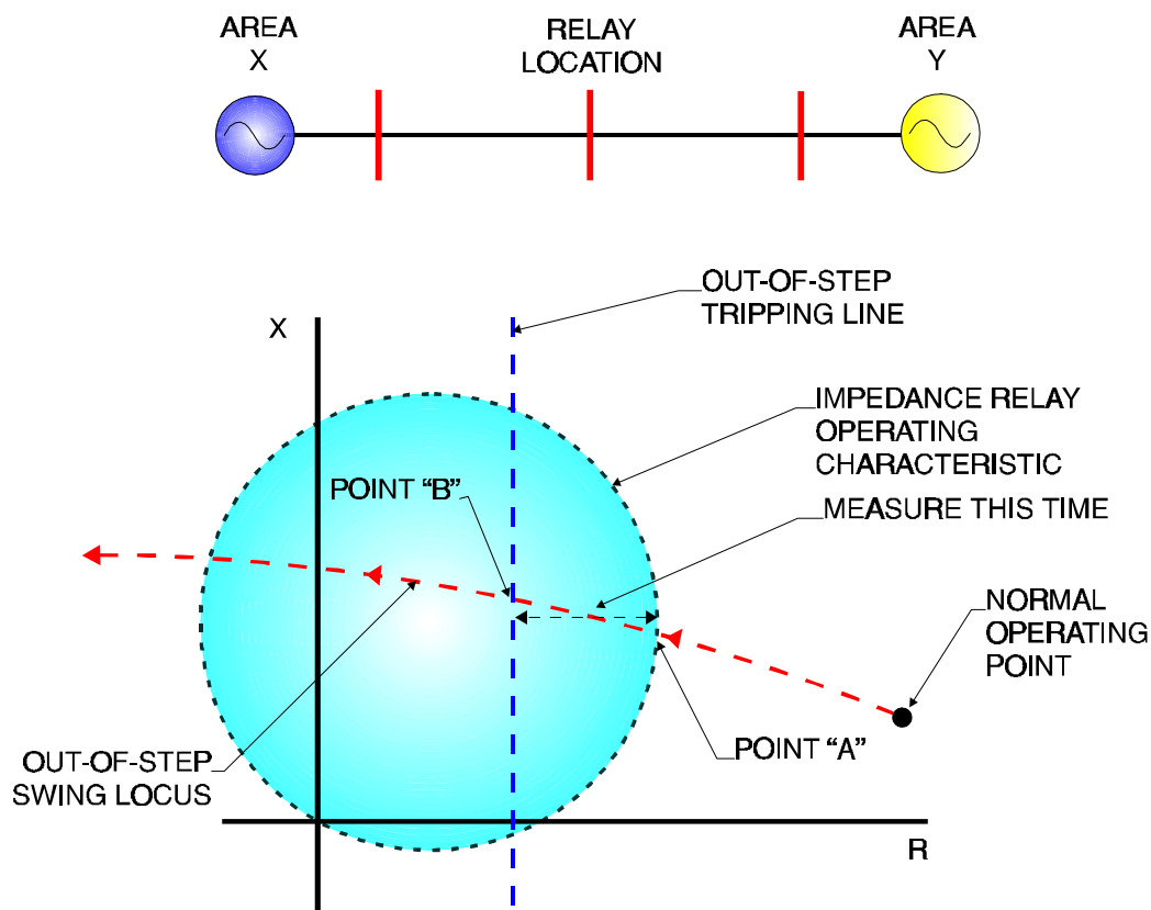
Figure 7-27 Out-of-Step Relay Characteristic
