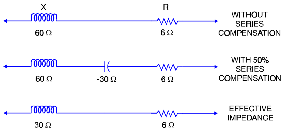
Figure 5-32 Series Compensation
