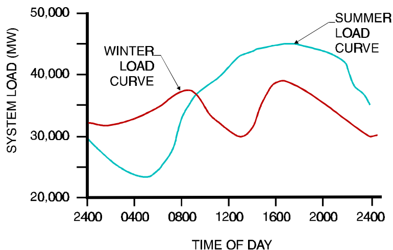
Figure 4-1 Summer and Winter Load Curves
