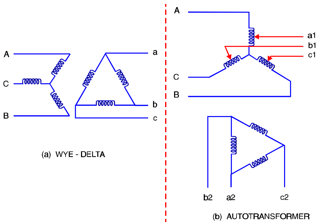
Figure 2-70 3F Transformer Connections
