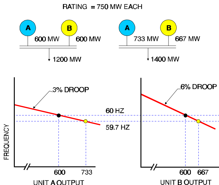
Figure 4-24 Load Sharing - Same Unit Ratings - Different Droop
