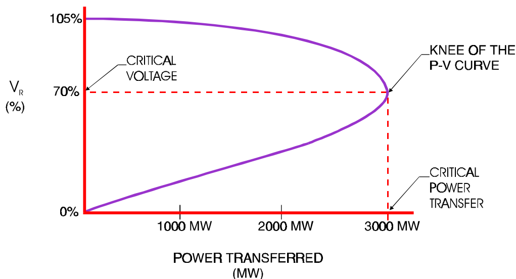
Figure 6-7 A Sample P-V Curve
