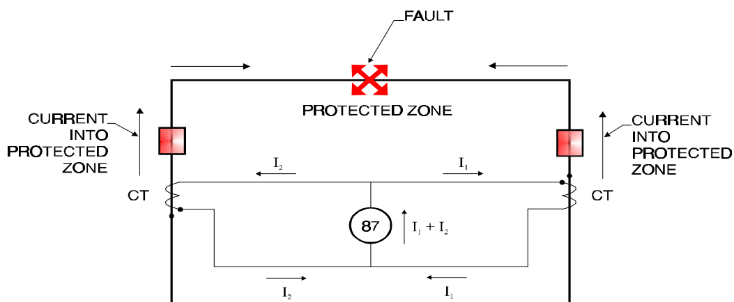
Figure 2-44 Fault Conditions for Differential Relay
