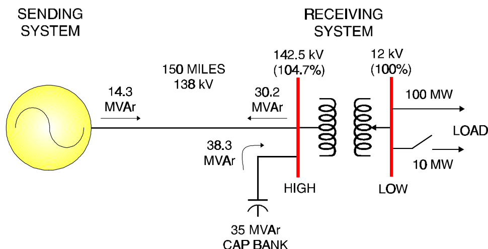
Figure 6-14 Conditions at Receiving Bus Prior to Adding 10 MW Load
