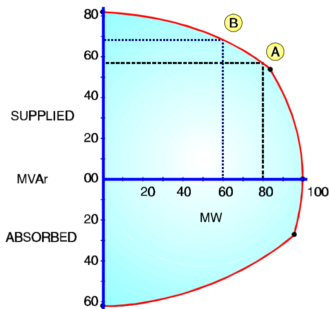
Figure 6-16 Adjusting the Generator Operating Point
