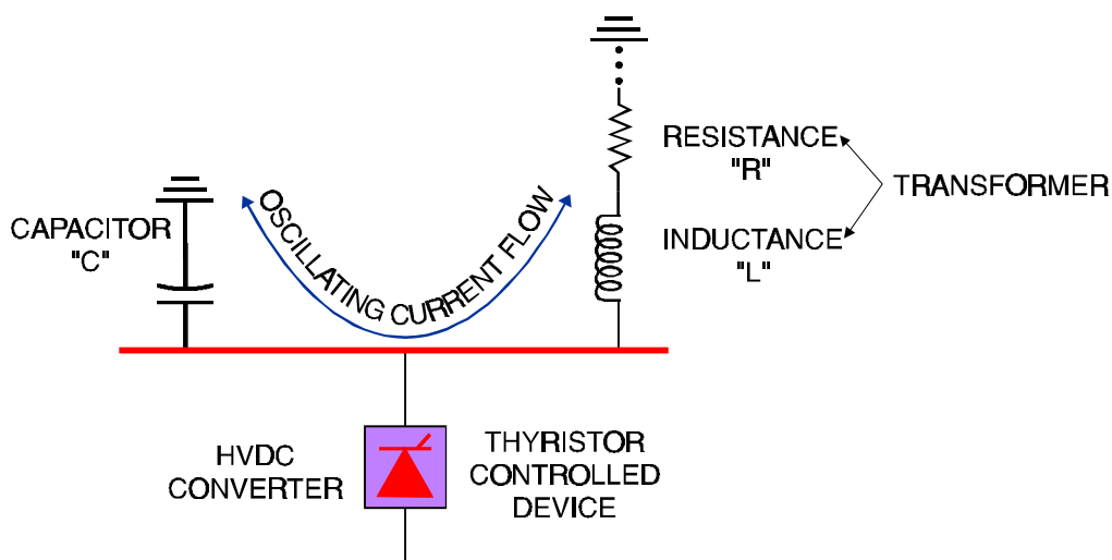
Figure 5-19 Harmonic Overvoltages
