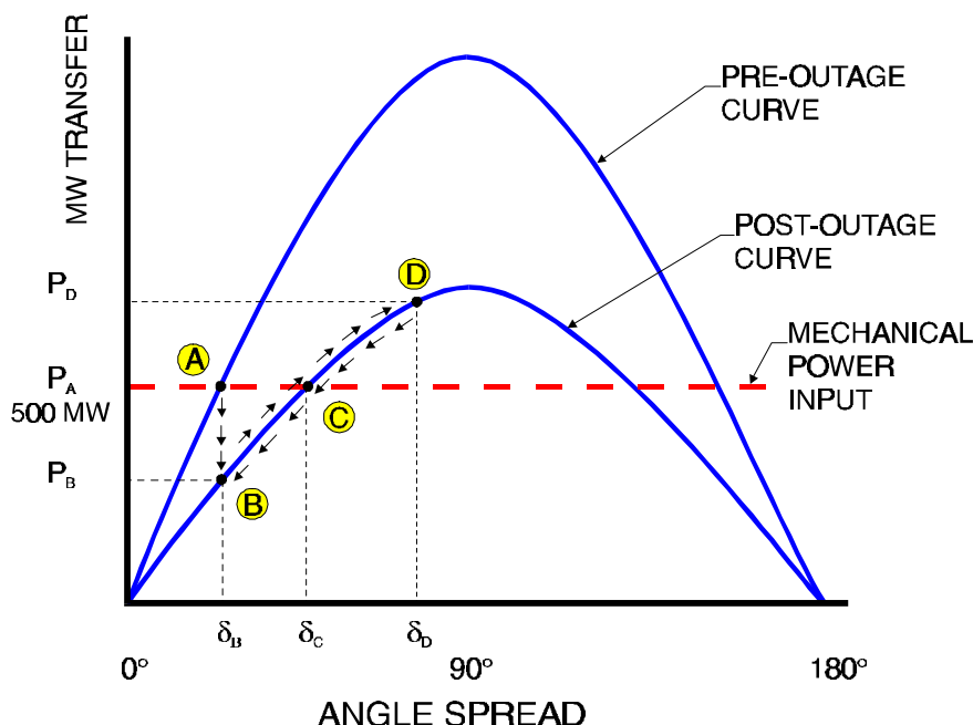
Figure 7-21 Power-Angle Curve for Oscillatory Stability
