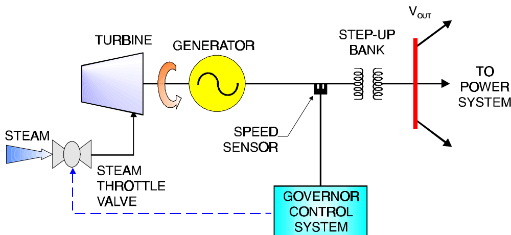
Figure 2-65 Model of Basic Governor Control System
