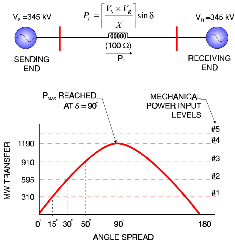
Figure 7-9 Steady State Instability
