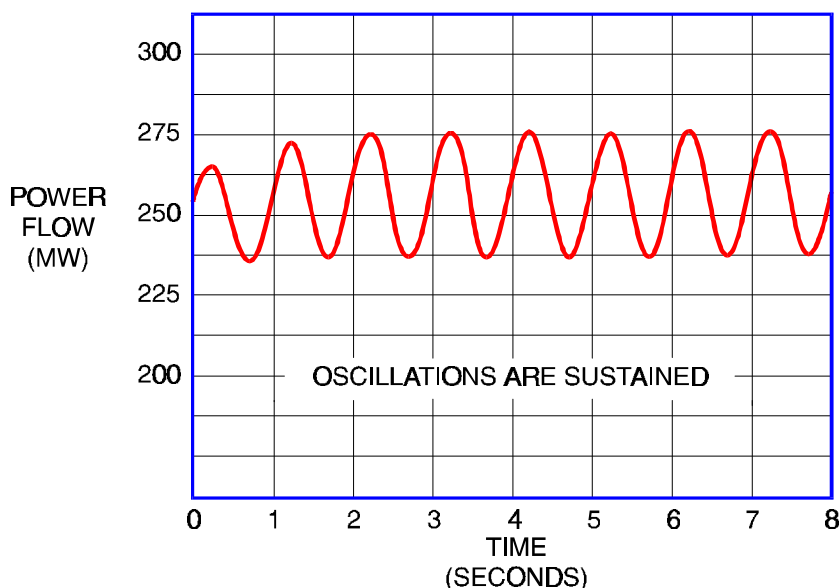
Figure 8-6 Sustained (Undamped) Power Oscillations
