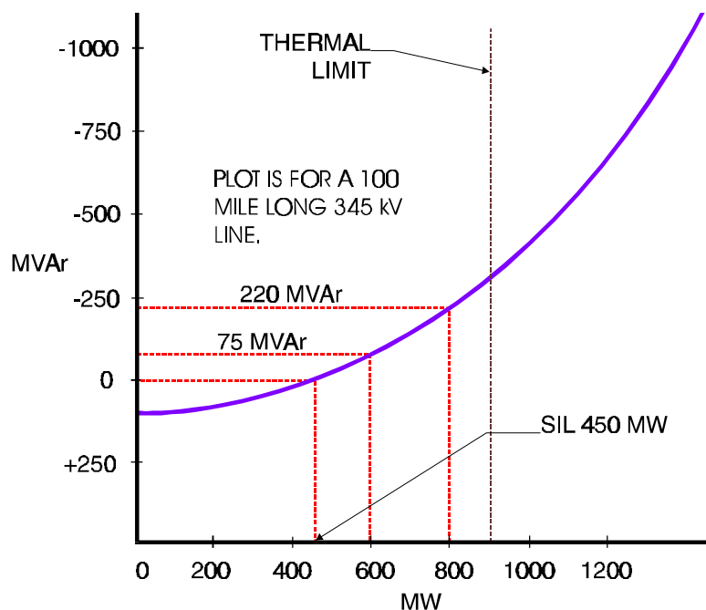
Figure 5-7 MW Required Versus MVar Transferred
