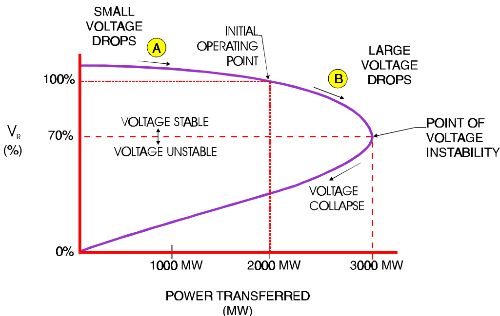
Figure 6-8 P-V Curve Illustration of Voltage Collapse
