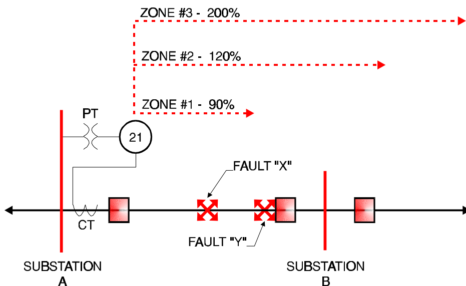
Figure 2-48 Distance Relay Scheme
