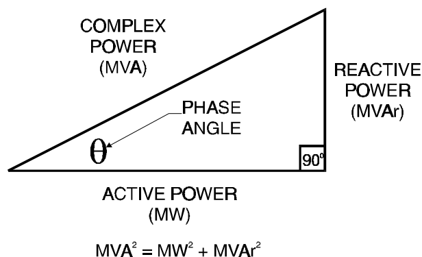
Figure 2-26 The Power Triangle
