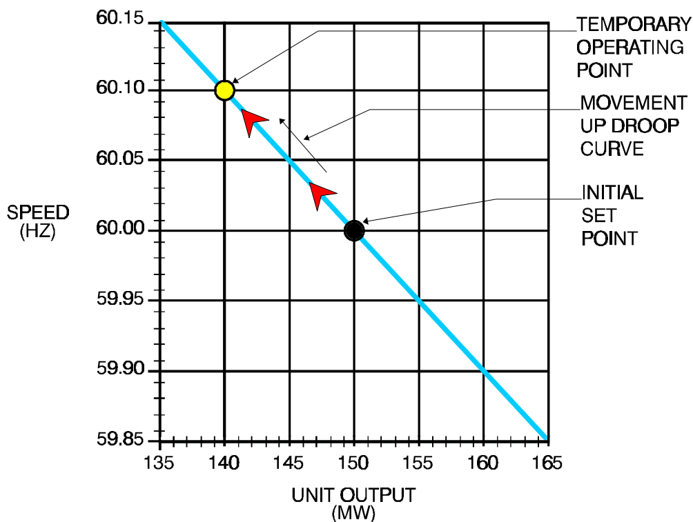
Figure 4-15 300 MW Unit with 5% Droop - Frequency Rise
