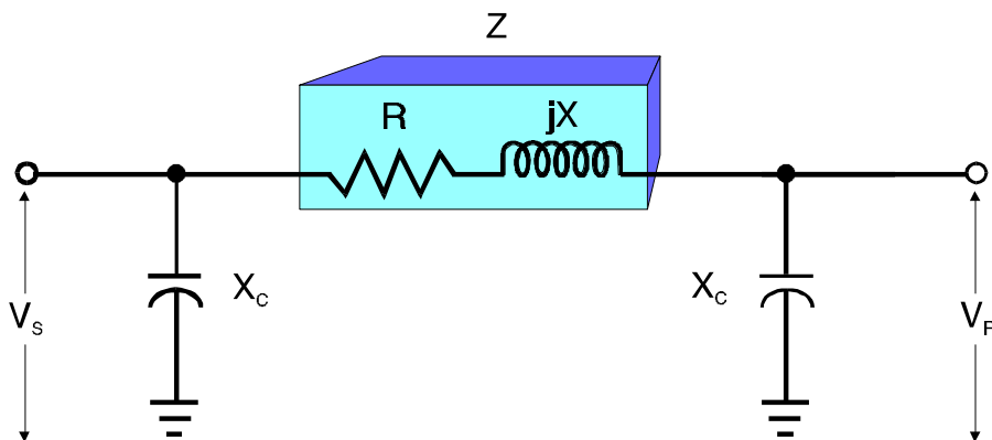
Figure 2-75 Transmission Line Impedance Model
