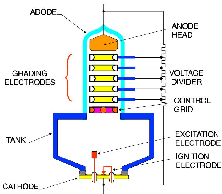
Figure 10-5 Mercury Arc Valve (MAV)
