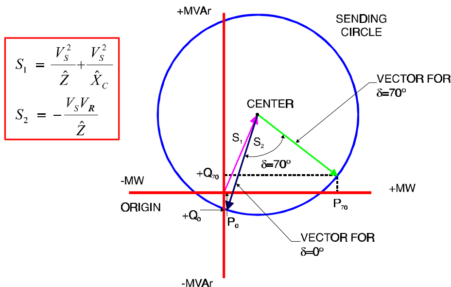
Figure 3-18 Sending End Power-Circle Diagram
