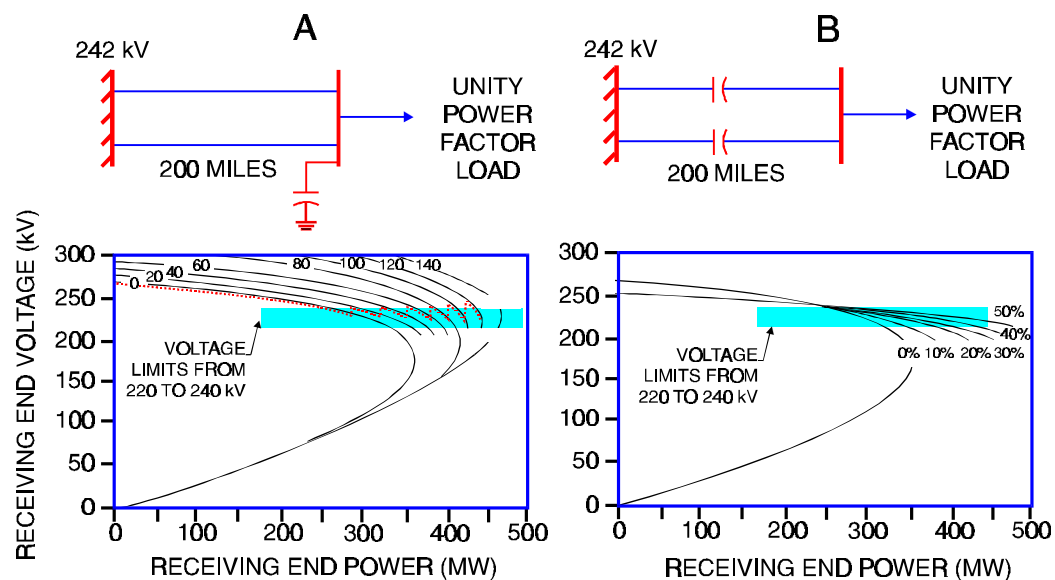
Figure 6-10 Shunt Versus Series Compensation
