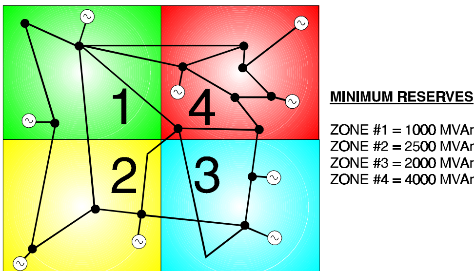
Figure 6-28 Voltage Control Zones
