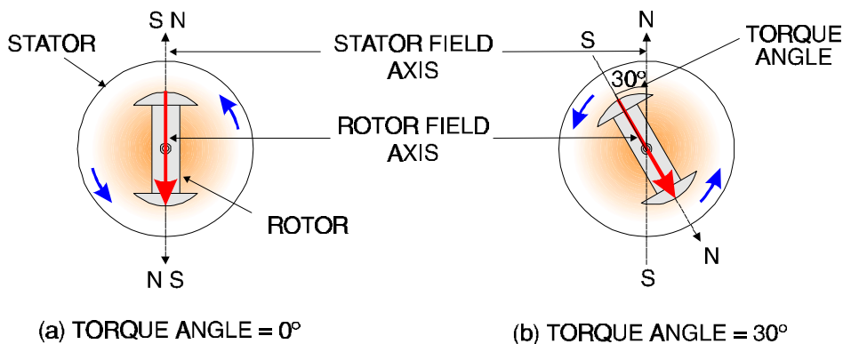
Figure 3-7 Generator Torque Angle
