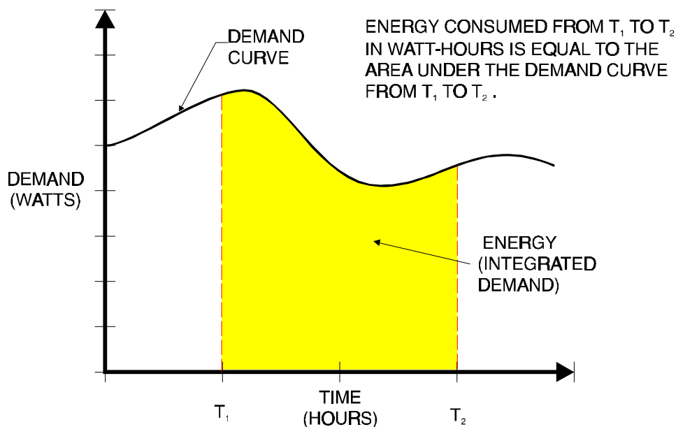
Figure 2-15 Integrated Demand
