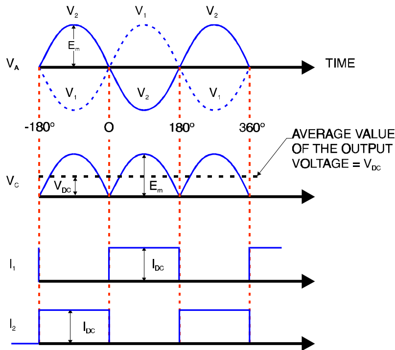
Figure 10-8 Waveforms for 1F Converter
