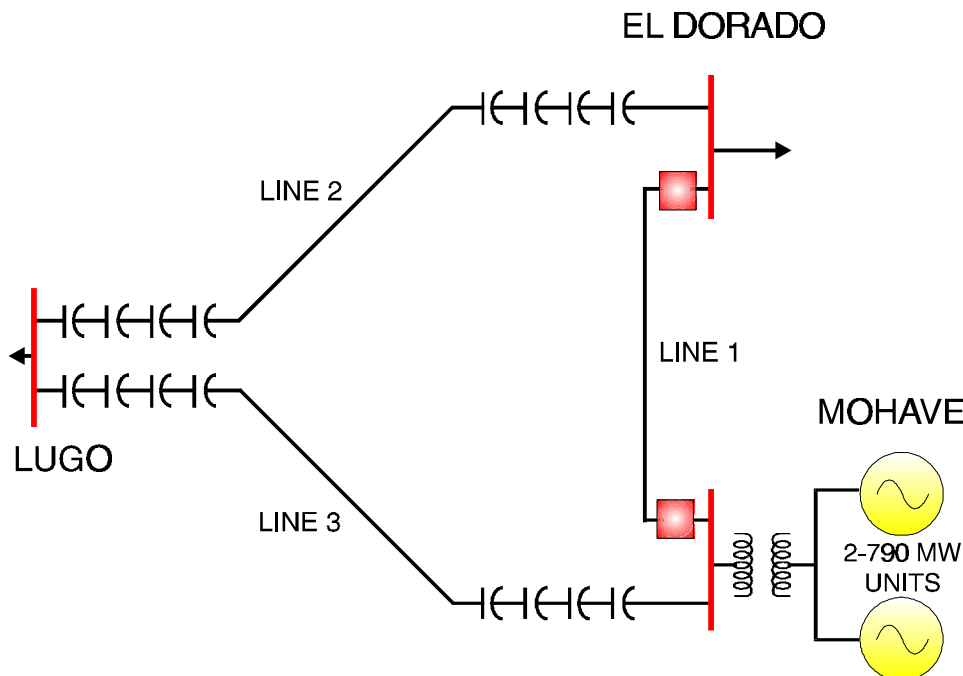
Figure 9-21 Mohave SSR Case Study
