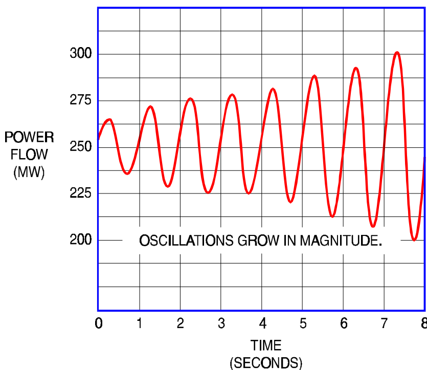
Figure 1-4 Power Oscillations
