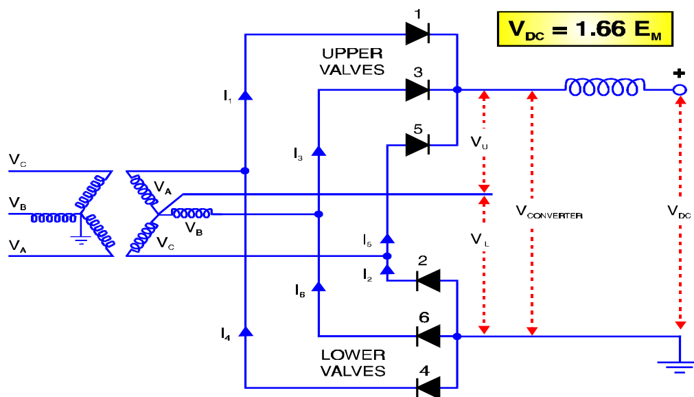
Figure 10-11 Three-Phase Two-Way Converter
