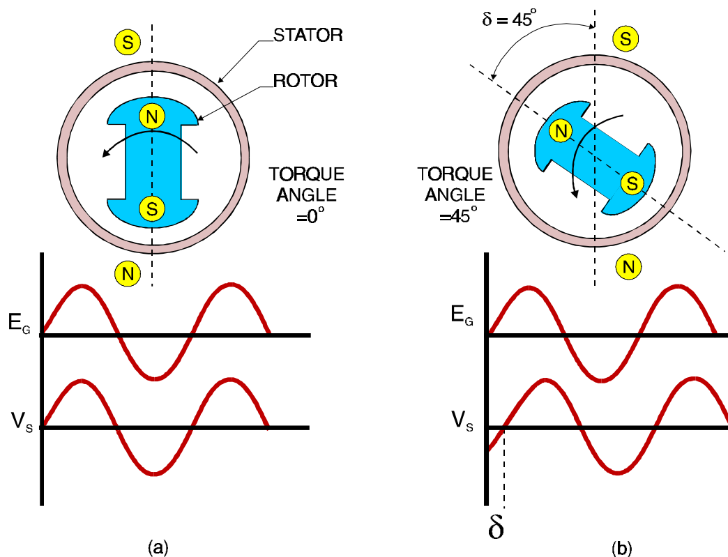
Figure 2-58 Torque Angle & Voltage
