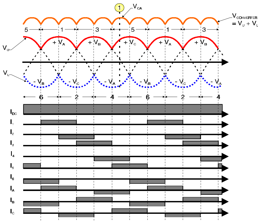
Figure 10-12 Waveforms for 3F Two-Way Converter
