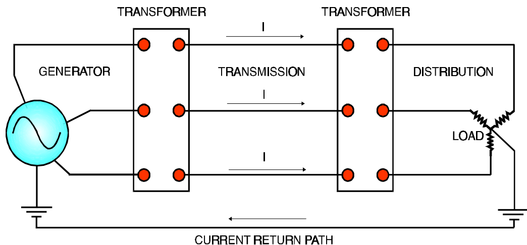
Figure 2-29 Power System Current Flow
