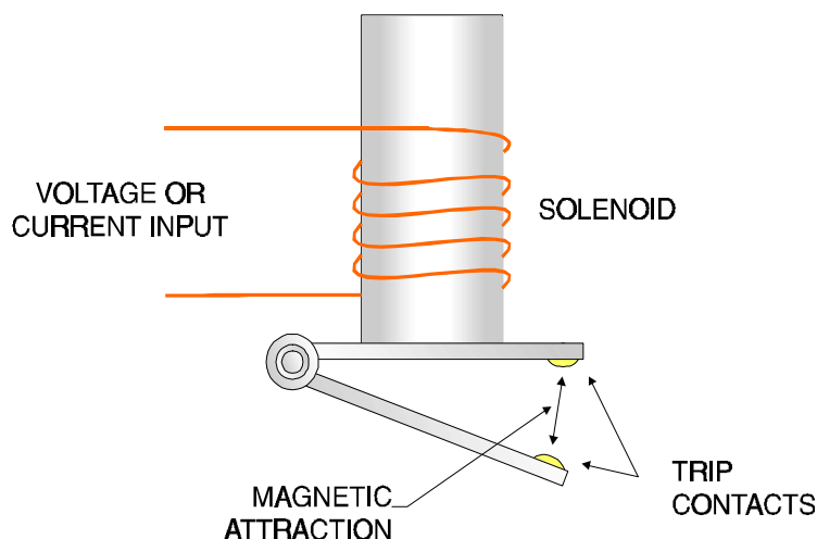
Figure 2-34 Magnetic Attraction Relay Element
