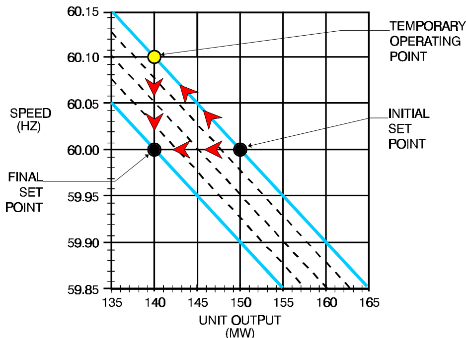
Figure 4-16 Changing the Set-Point to 140 MW @ 60 HZ
