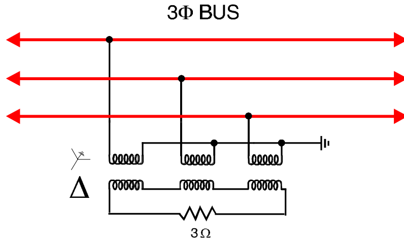
Figure 9-32 Resistor in a Delta Connected Secondary
