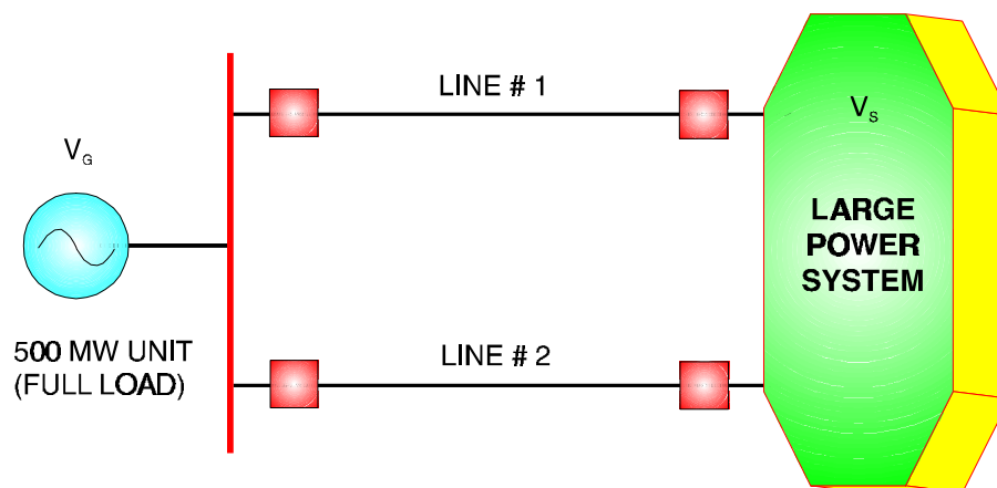
Figure 8-8 Loss of a Line to Start an Oscillation
