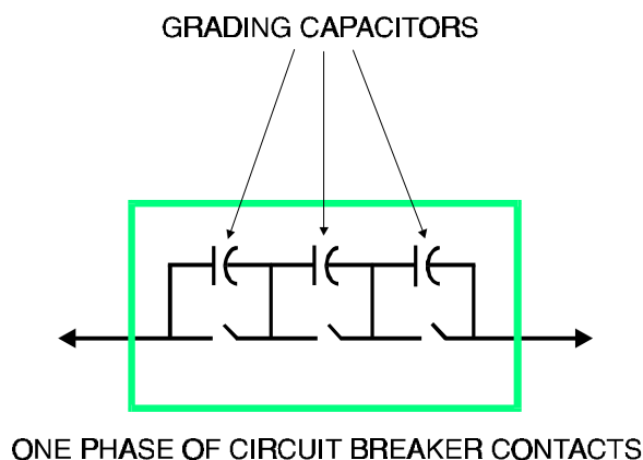
Figure 9-29 Multi-Break Circuit Breaker Contacts
