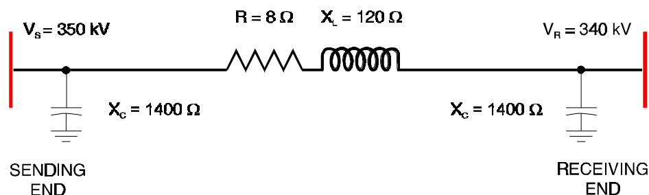
Figure 3-20 System for Illustrating Use of Power-Circle Diagram
