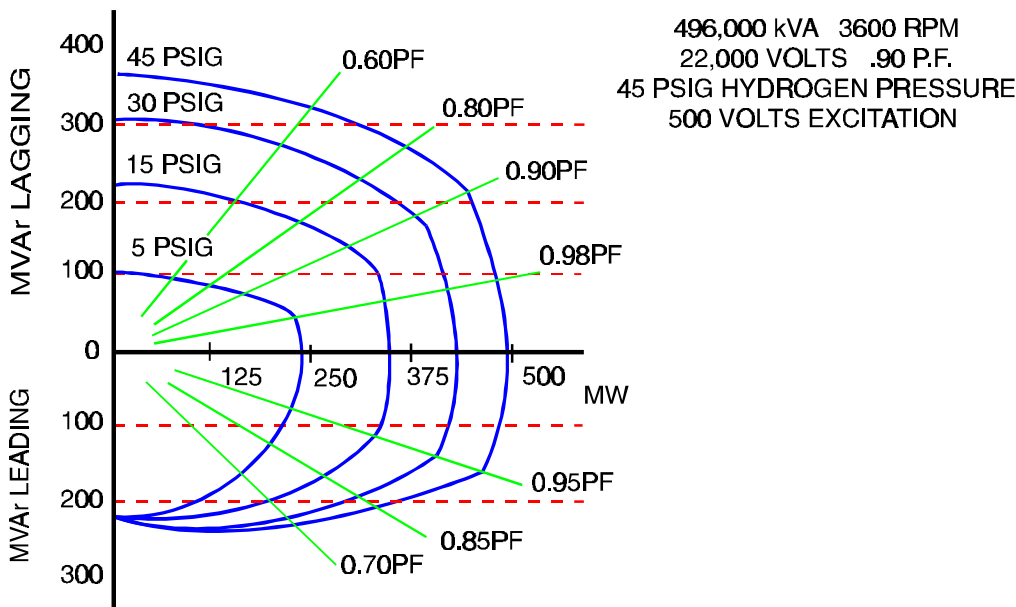
Figure 5-41 Actual Thermal Unit Reactive Capability Curve
