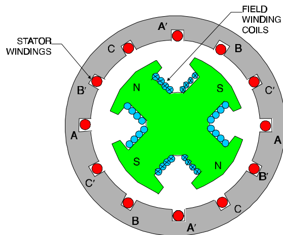
Figure 2-56 Four Pole Rotor
