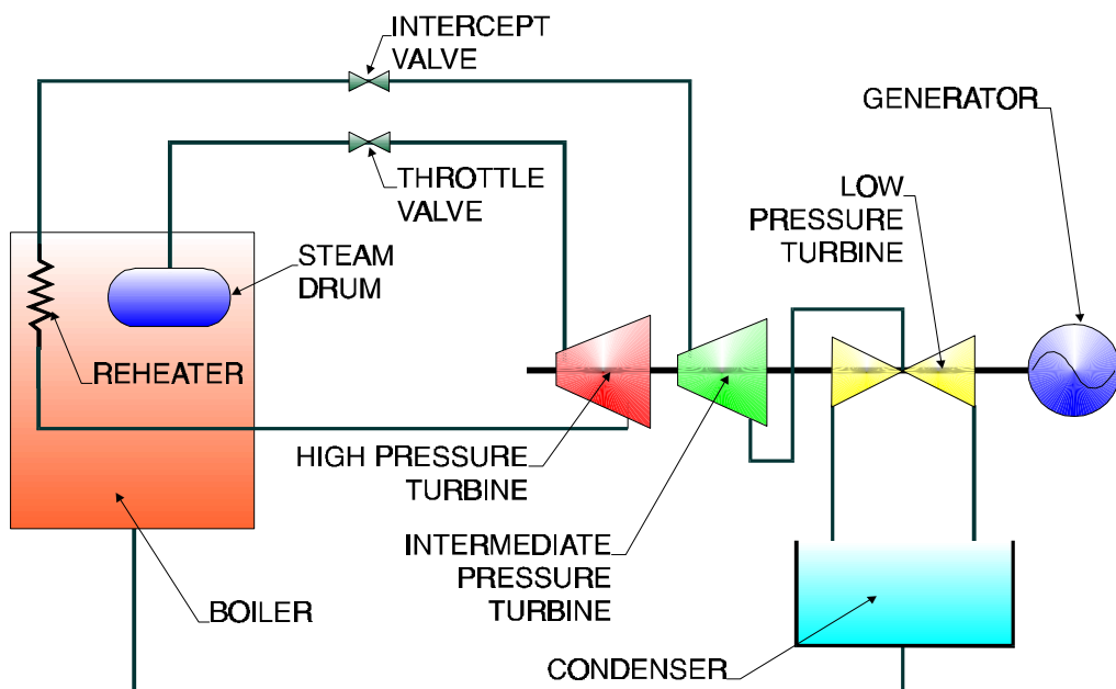
Figure 7-18 Fast Valving in Steam Units
