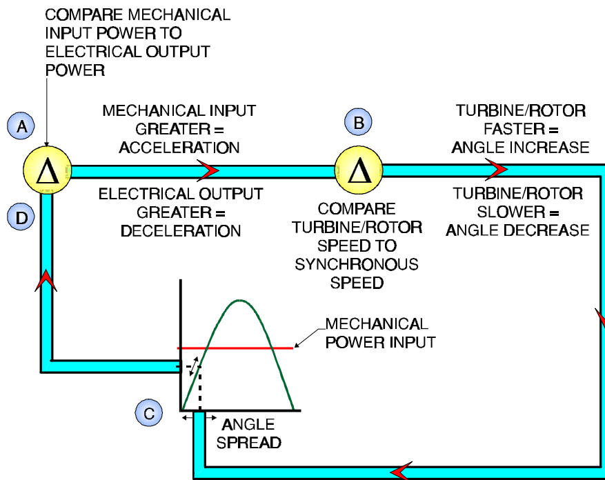
Figure 8-9 Feedback Loop for Power, Speed & Angle
