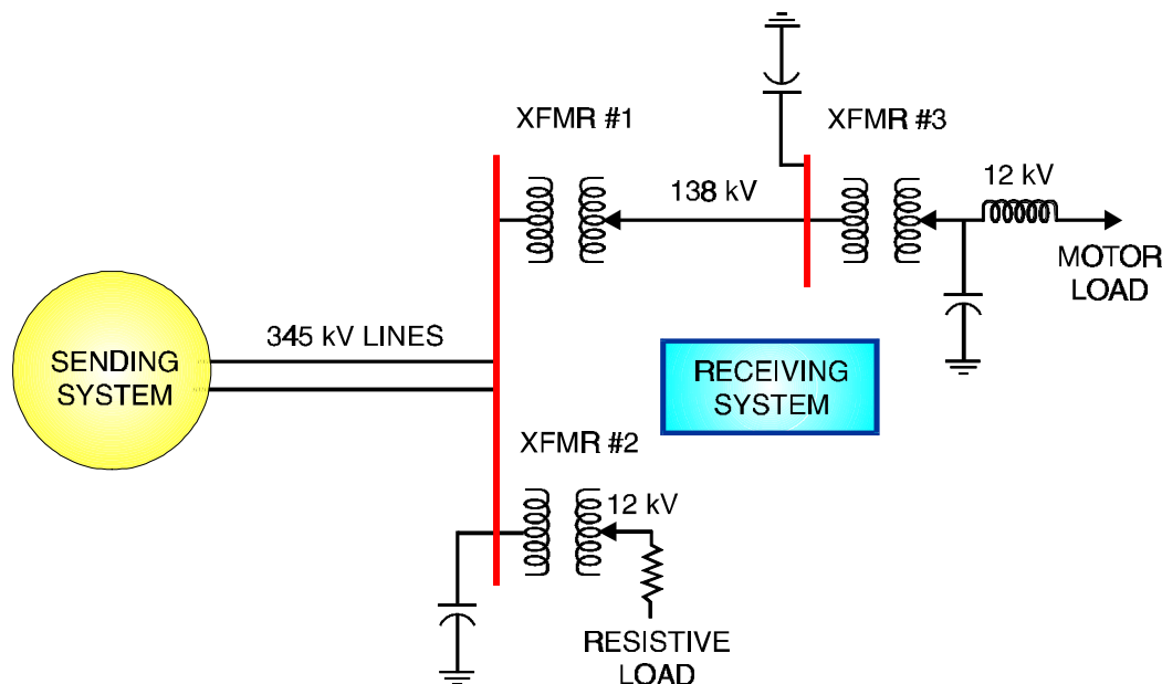
Figure 6-6 A Radial Power System
