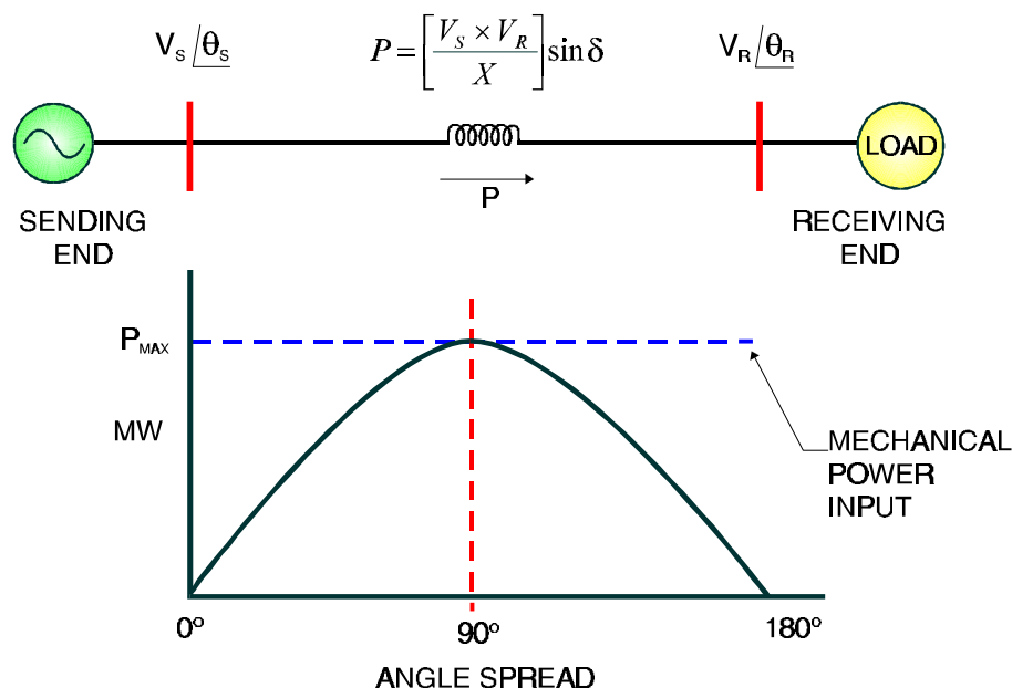
Figure 7-6 The Power-Angle Curve
