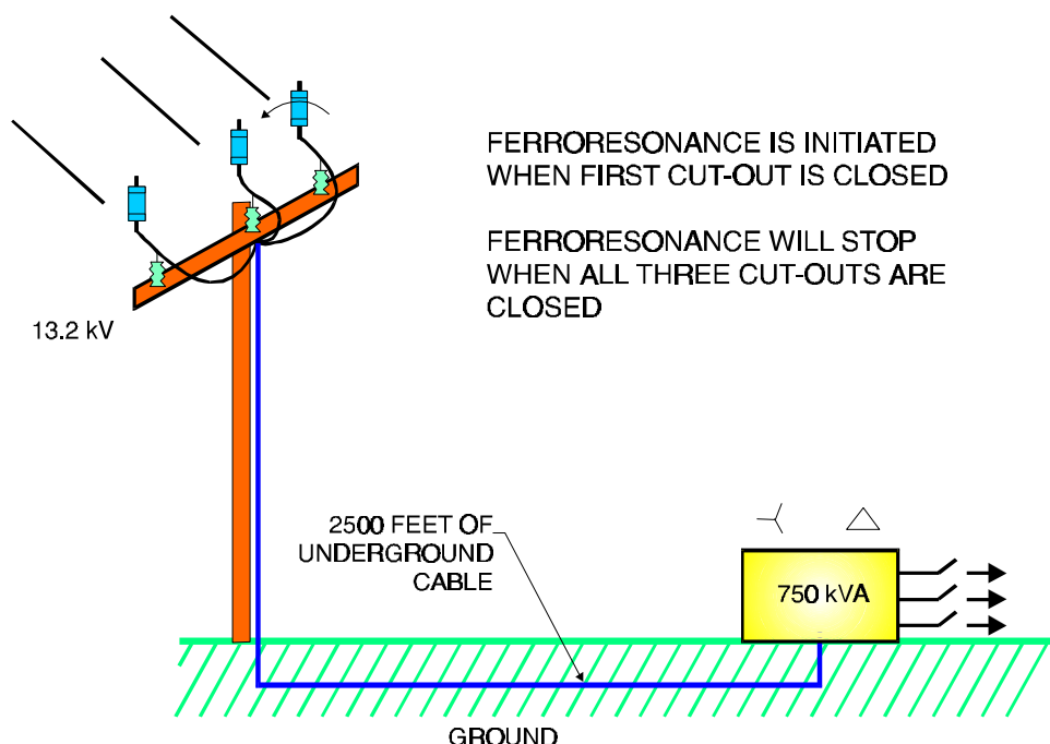
Figure 9-22 Distribution System Ferroresonance
