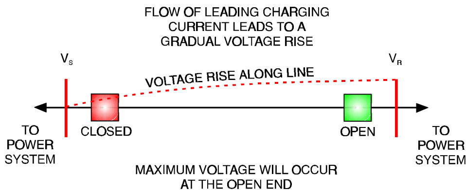
Figure 5-14 Voltage Profile Due to Ferranti Effect
