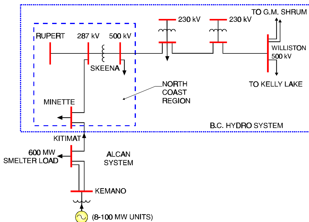
Figure 6-21 North Coast System One-Line Diagram
