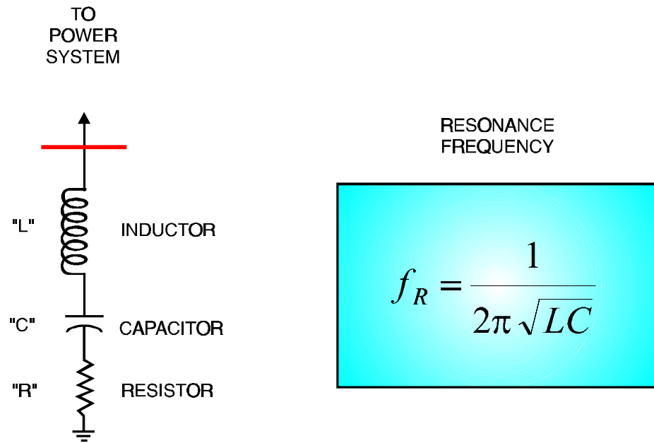
Figure 9-8 Harmonic Filter
