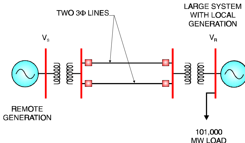
Figure 7-12 Power System for Transient Stability & Instability
