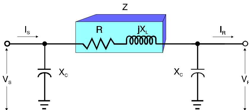
Figure 3-8 Transmission Line PI Model
