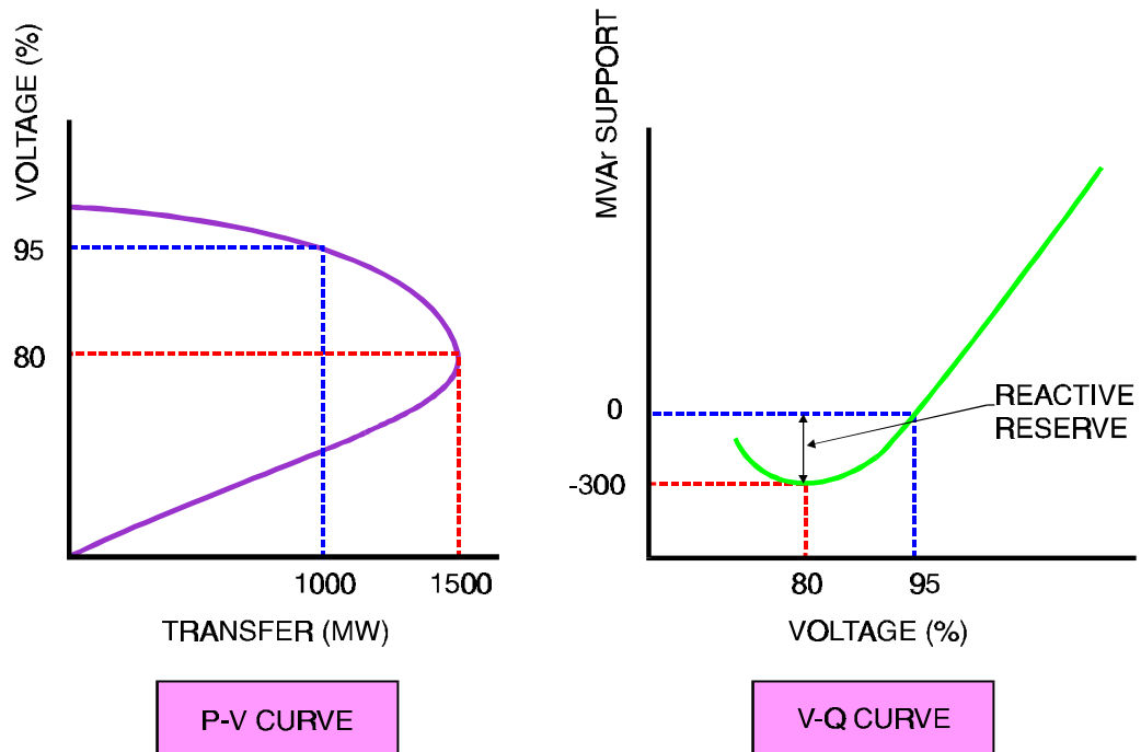
Figure 6-19 P-V & V-Q Curves
