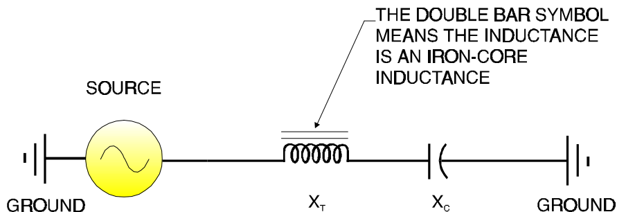
Figure 9-23 Series Resonance Circuit
