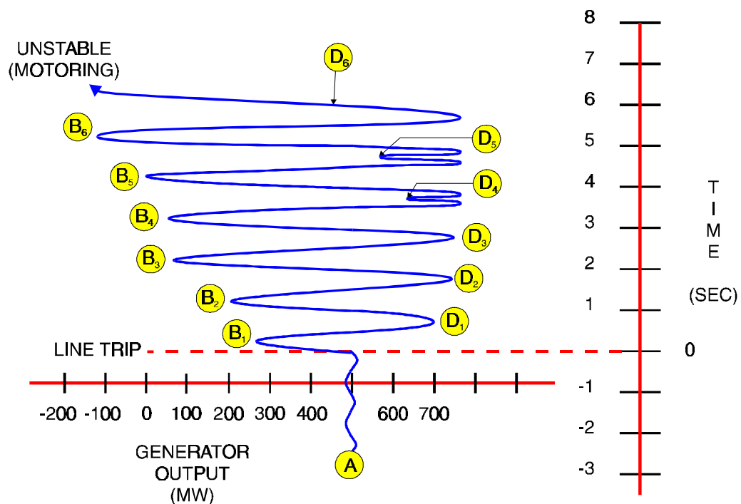
Figure 7-25 Strip Chart Illustration of Oscillatory Instability
