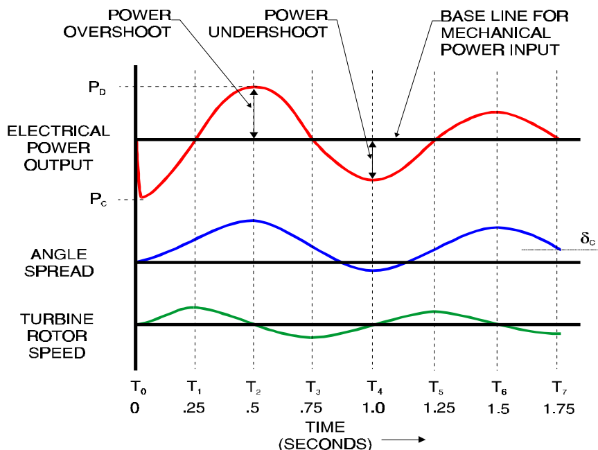
Figure 8-10 Plots of Power Output, Angle Spread & Rotor Speed
