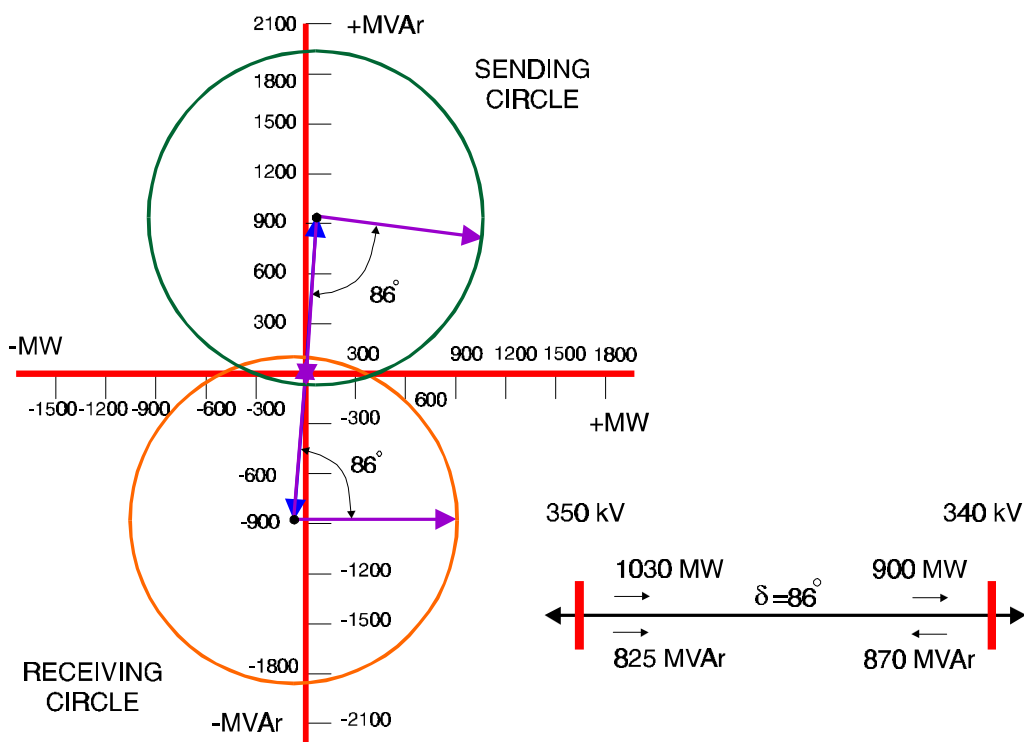
Figure 3-23 Power-Circle Diagram with a \delta of 86^\circ
