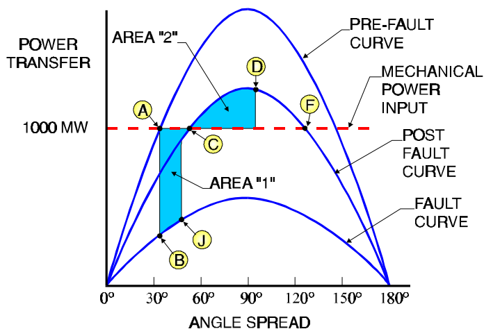
Figure 7-16 Transient Stability and a Fault
