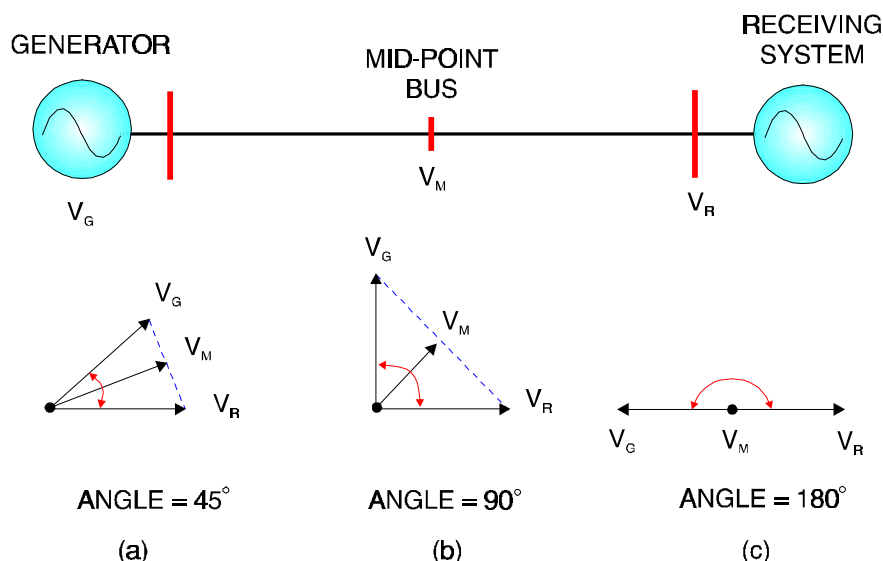
Figure 7-3 Out-of-Step from a Voltage Perspective
