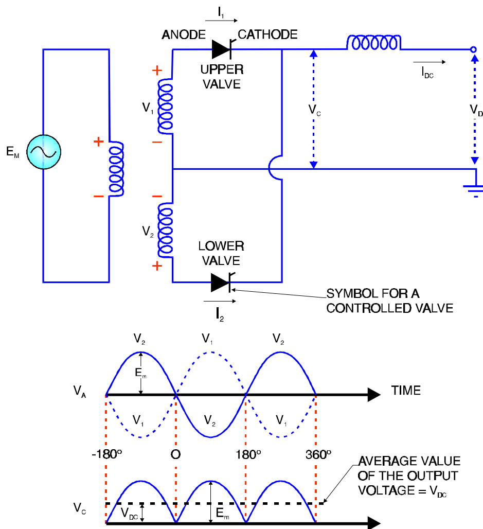
Figure 10-19 Two-Pulse Operation without Gate Control
