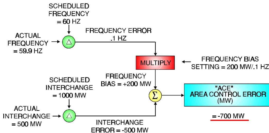
Figure 4-36 ACE for an Internal Generation Loss
