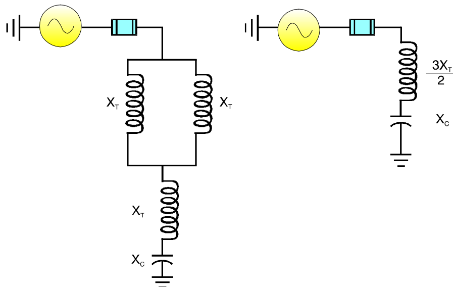
Figure 9-26 Circuit After Phases "B" & "C" Are Closed
