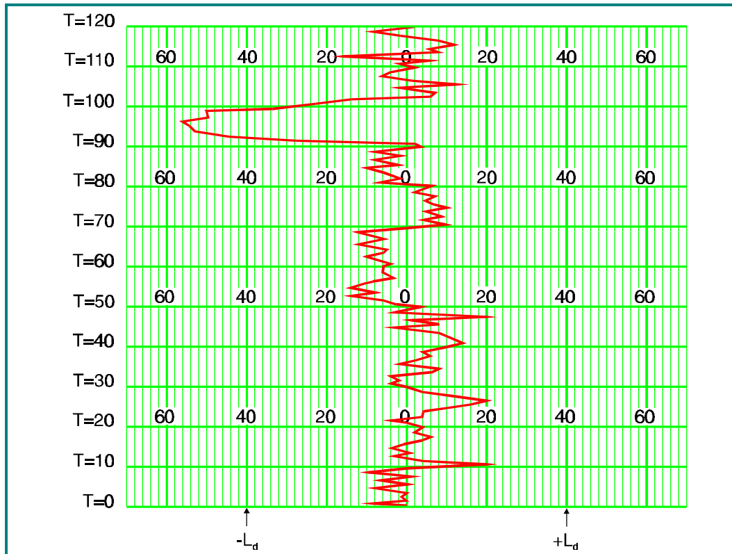
Figure 4-43 Violation of A1 and A2 Criteria
