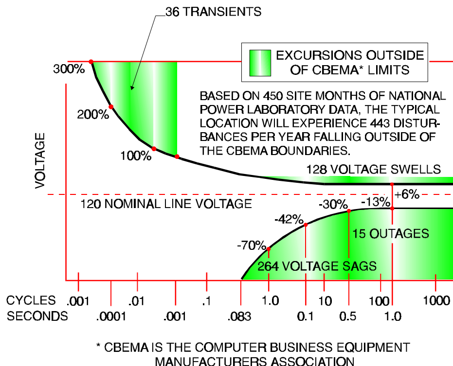
Figure 5-30 Computer Equipment Voltage Limits
