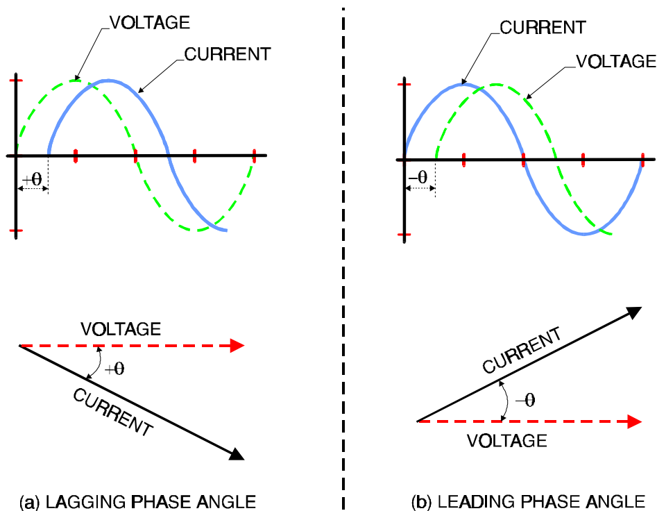
Figure 3-2 Concept of Phase Angle ( \theta )
