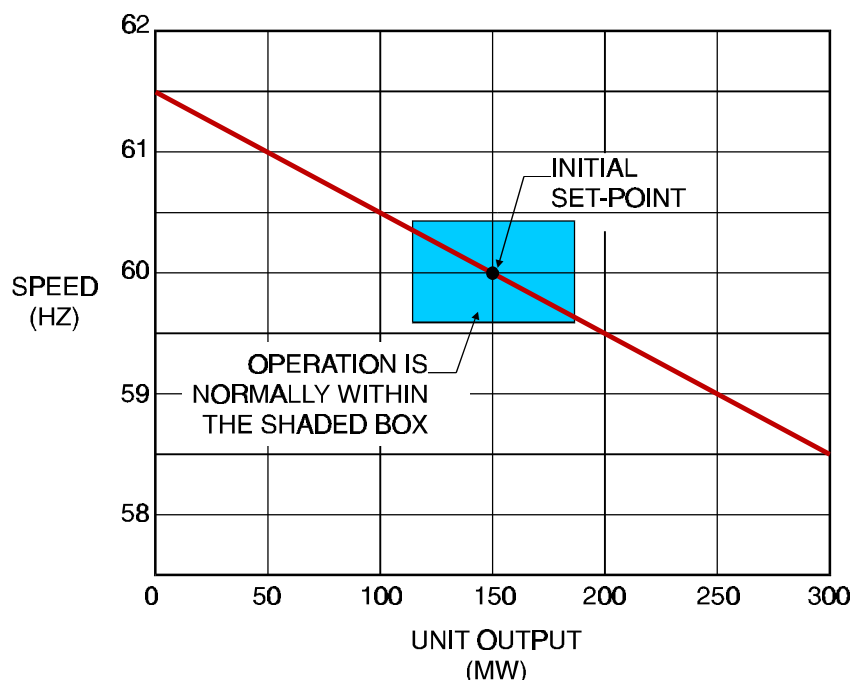
Figure 4-13 Governor Characteristic Curve with 5% Droop
