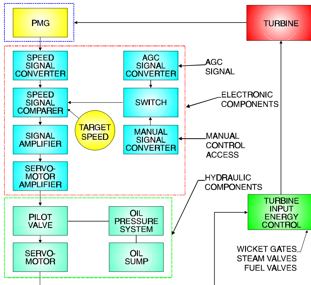
Figure 4-11 Electro-Hydraulic Governor Block Diagram
