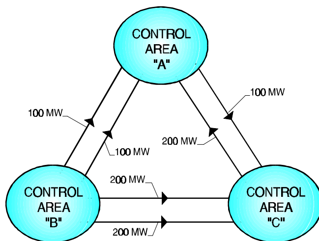
Figure 4-30 Control Area Interchange
