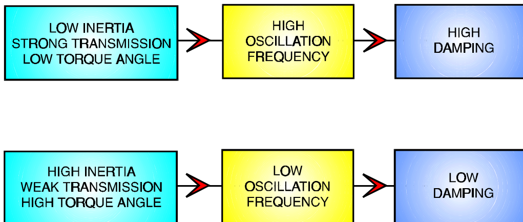
Figure 8-12 High & Low Frequency Oscillations
