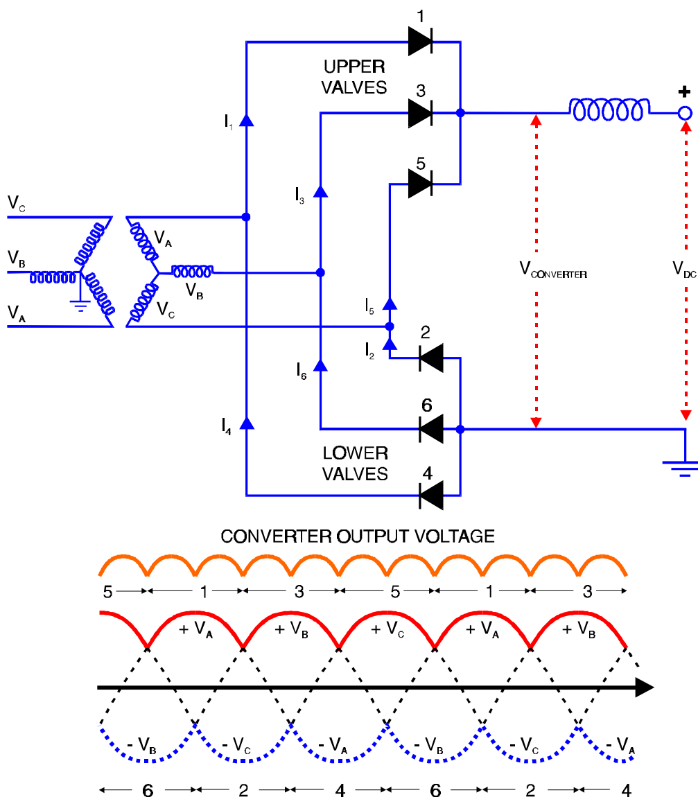
Figure 10-18 Six-Pulse Converter Operation without Gate Control
