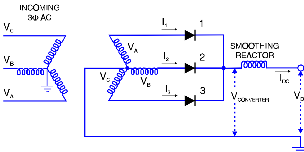
Figure 10-9 Three-Phase One-Way Converter
