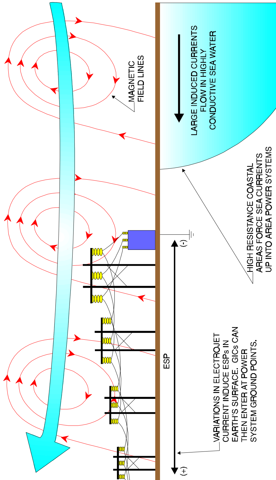
Figure 9-40 Summary of GIC Creation and Entry to Power System
