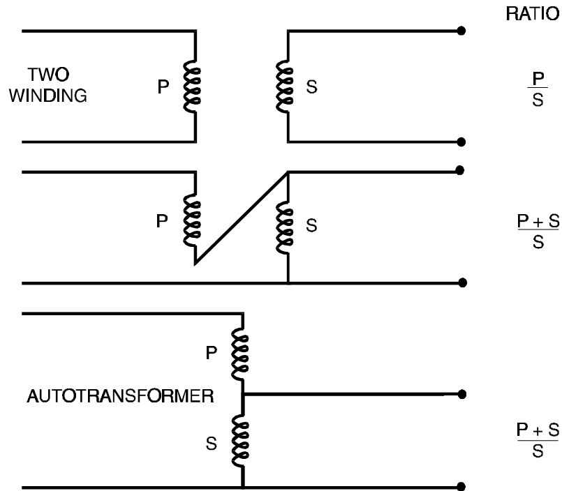
Figure 2-69 Autotransformer Evolution
