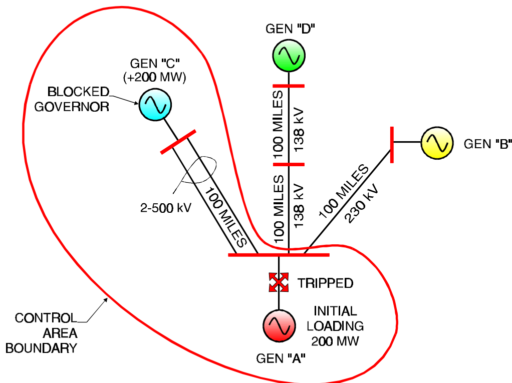
Figure 4-58 Stage #4 - The AGC Stage
