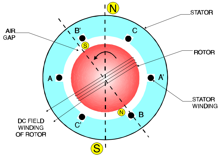
Figure 2-55 Two Pole Rotor
