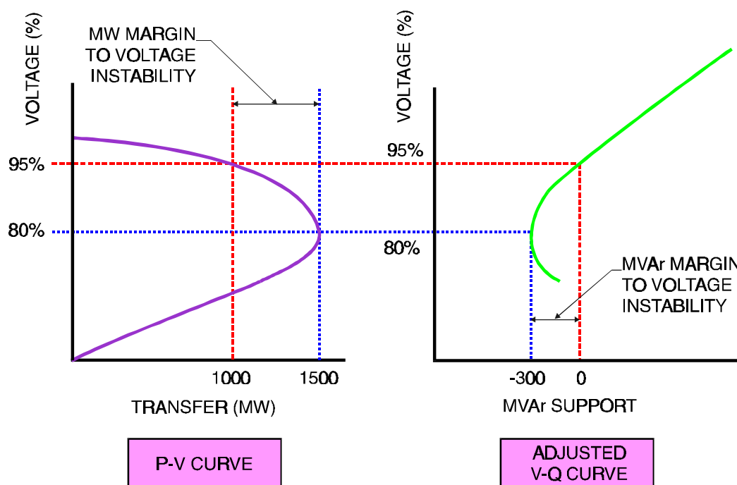
Figure 6-20 Margins to Voltage Instability
