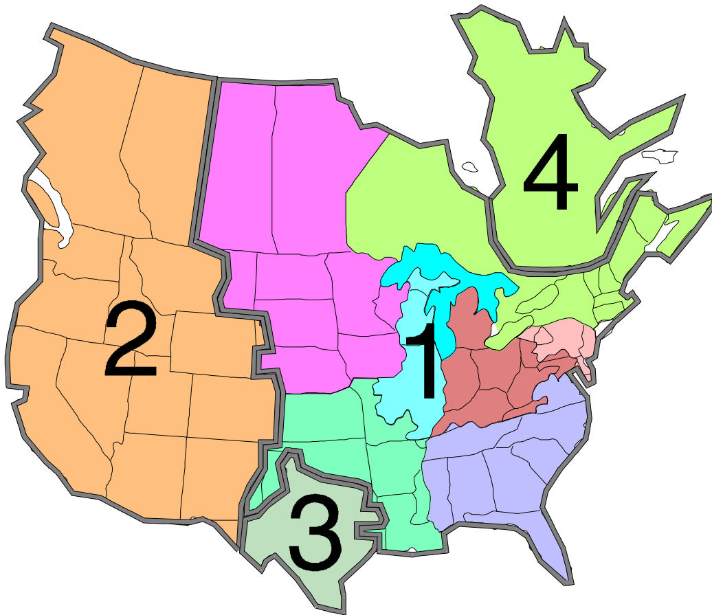
Figure 2-77 The Four Major Interconnections
