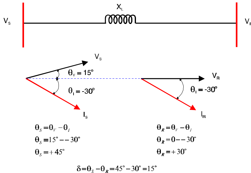
Figure 3-4 Determining Approximate Power Angle from Phase Angles
