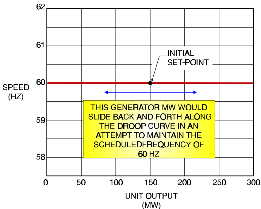
Figure 4-12 Isochronous Governor Characteristic Curve
