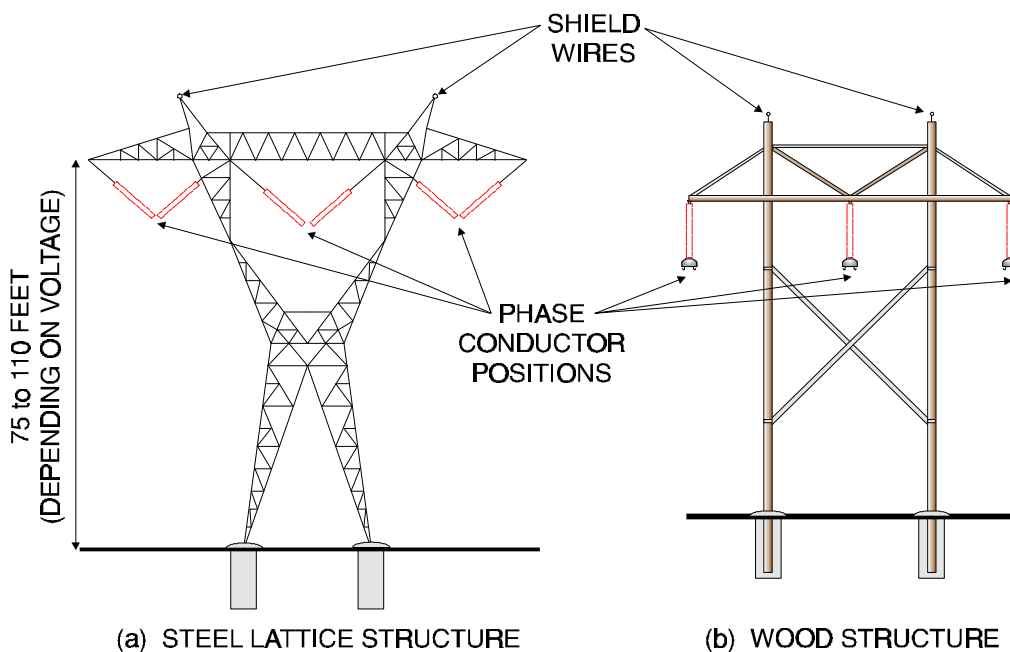
Figure 2-71 Transmission Line Structures
