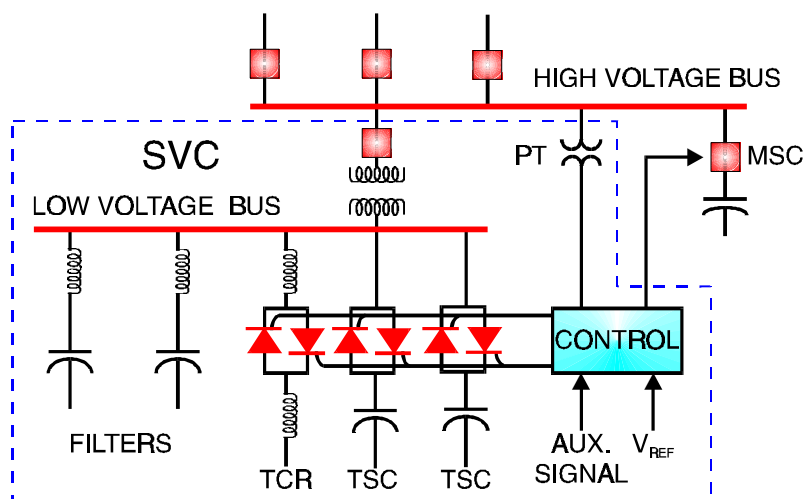
Figure 5-45 Static Var Systems (SVS)
