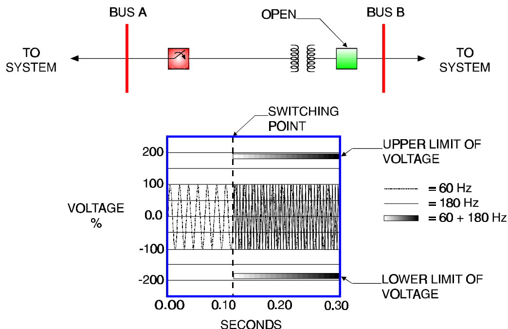
Figure 5-20 Energizing a Line-Transformer Combination
