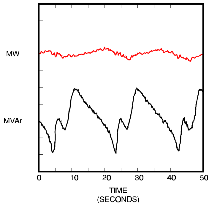
Figure 8-24 Generator Out-of-Step Oscillations
