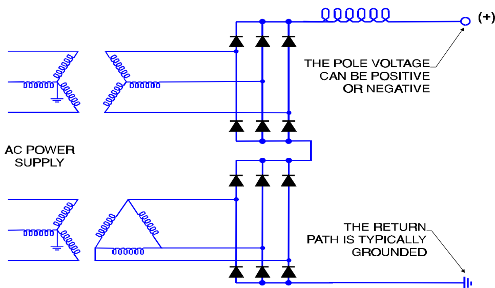
Figure 10-13 Twelve-Pulse Converter
