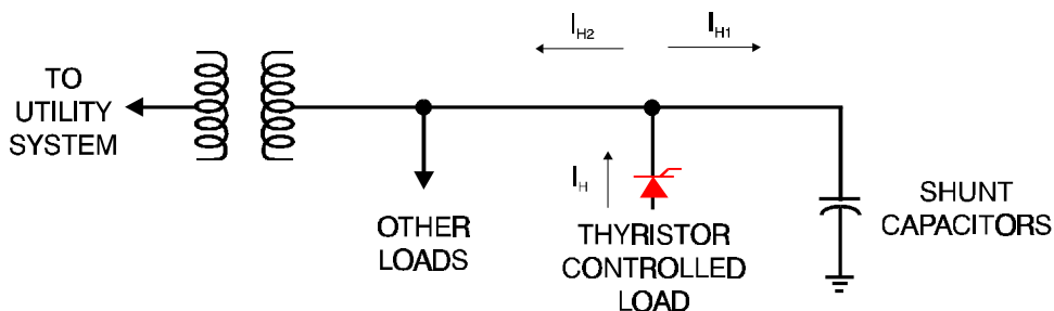
Figure 9-6 Flow of Harmonic Current
