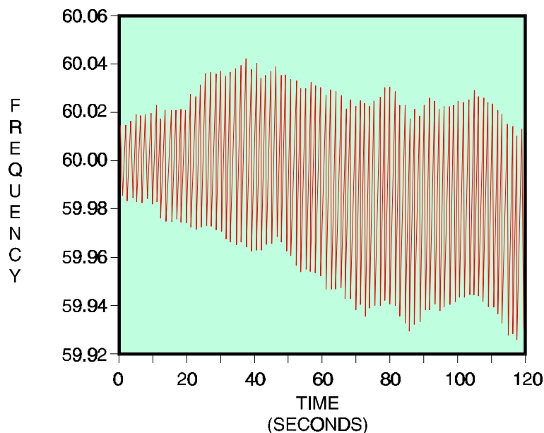
Figure 8-22 Oscillations Caused by Misoperating HVDC Controls
