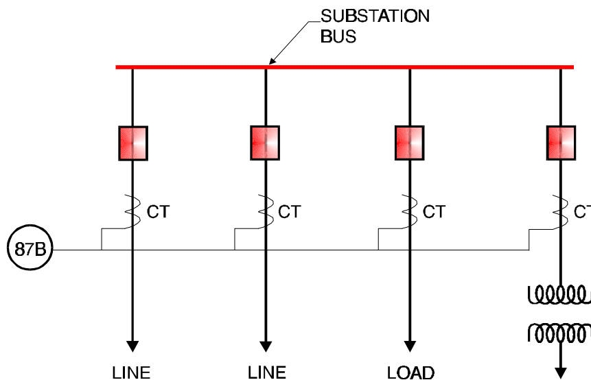
Figure 2-45 One-line with Bus Differential
