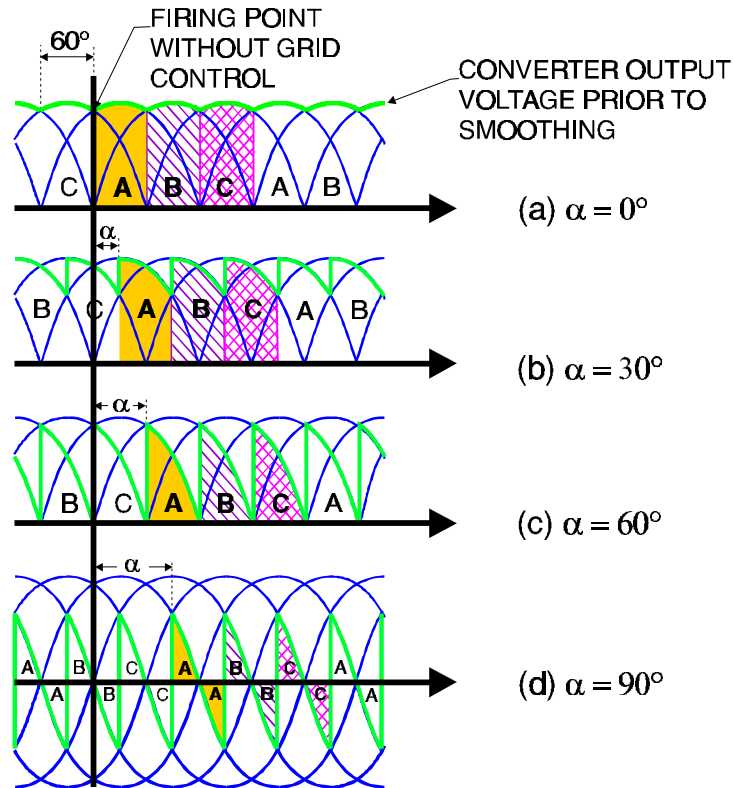
Figure 10-21 Six-Pulse Converter Ignition Delay Angles of 0° - 90°
