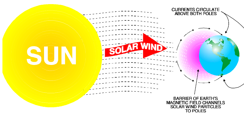
Figure 9-34 Solar Wind and Earth Currents
