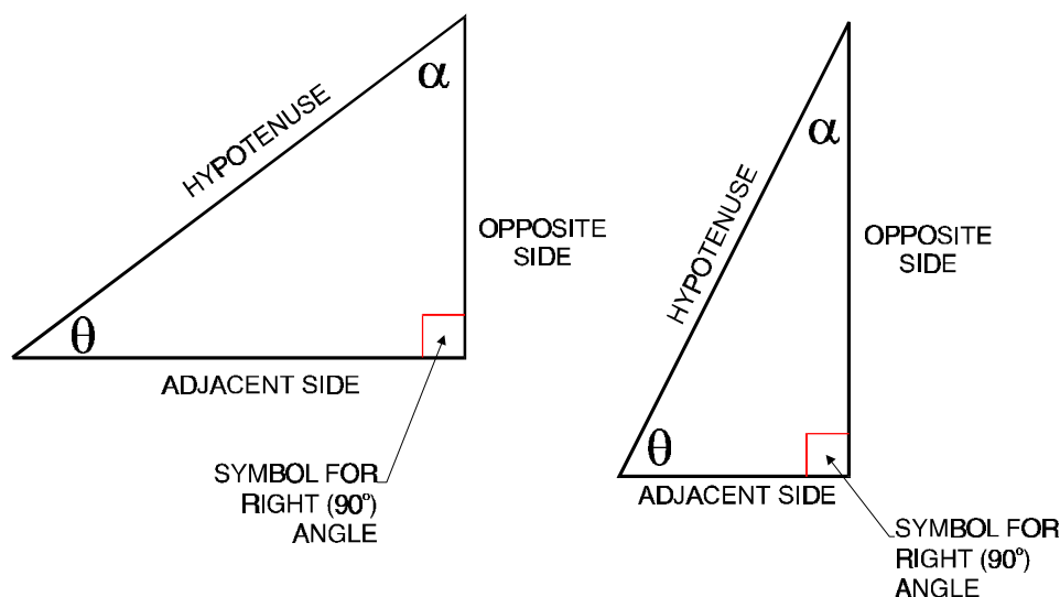
Figure 2-1 Right Triangles
