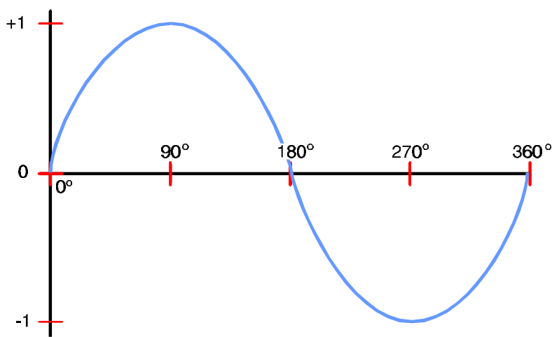
Figure 2-2 Sine Function
