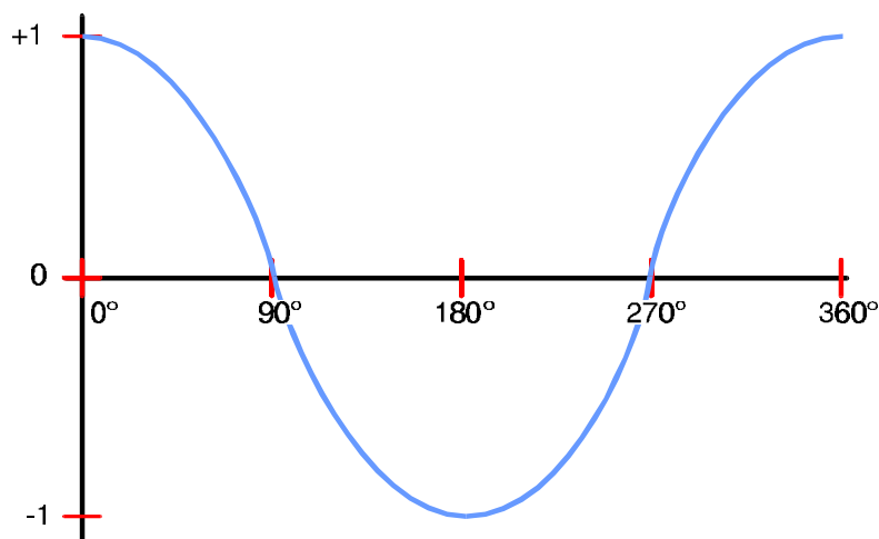
Figure 2-4 Cosine Function
