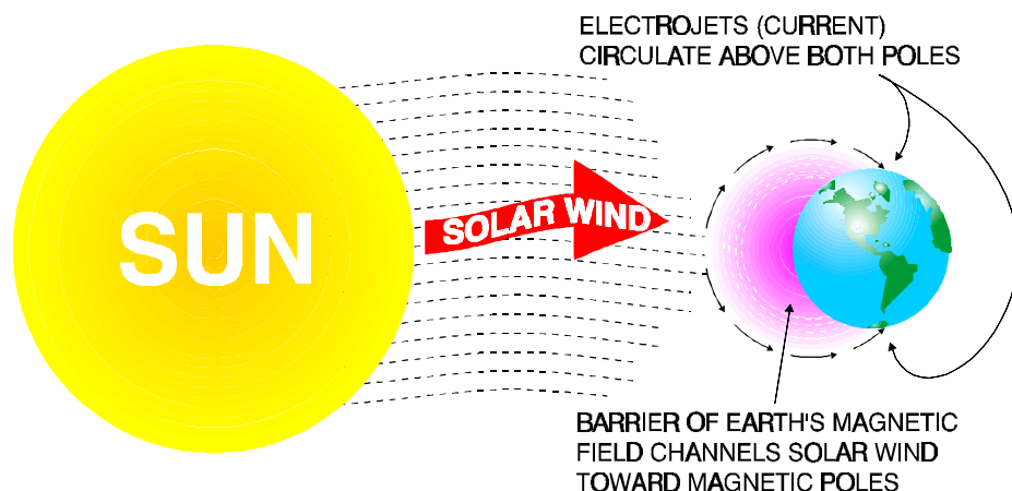
Figure 1-6 Geomagnetic Disturbances (GMDs)
