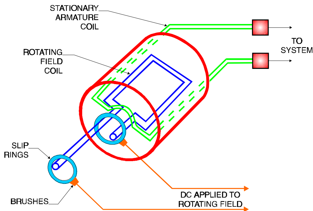
Figure 2-54 Single Phase AC Power Generator
