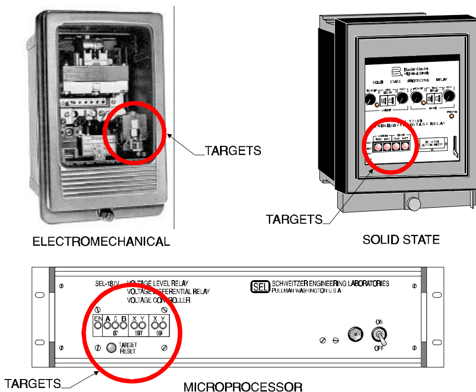
Figure 2-36 Electromechanical, Solid State & Microprocessor Relays
