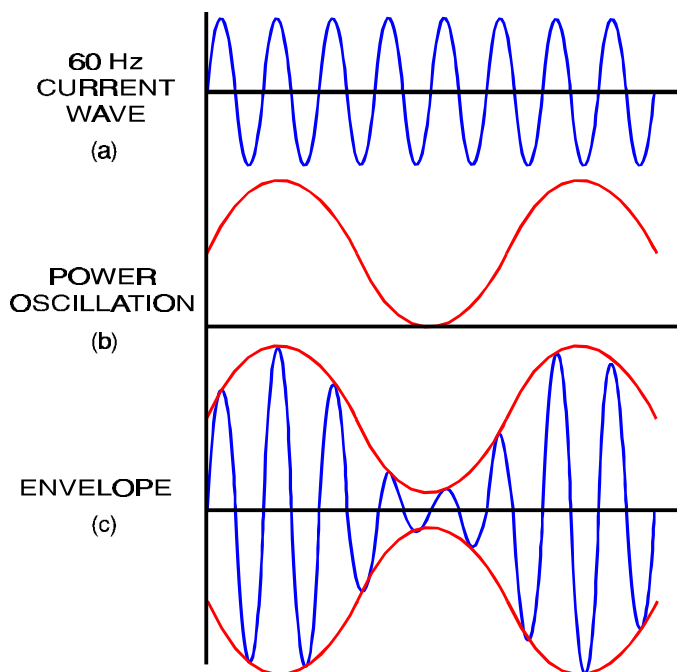
Figure 8-4 Current Oscillation Envelope
