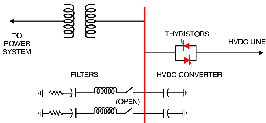
Figure 9-15 HVDC Converter Simplified One-Line
