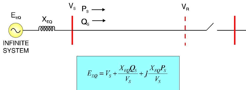
Figure 5-17 Source End Voltage Rise
