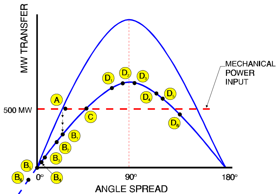
Figure 7-24 Power-Angle Curve for Oscillatory Instability
