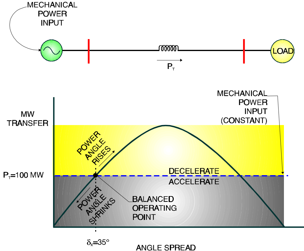
Figure 7-7 Accelerating and Decelerating on a Power-Angle Curve
