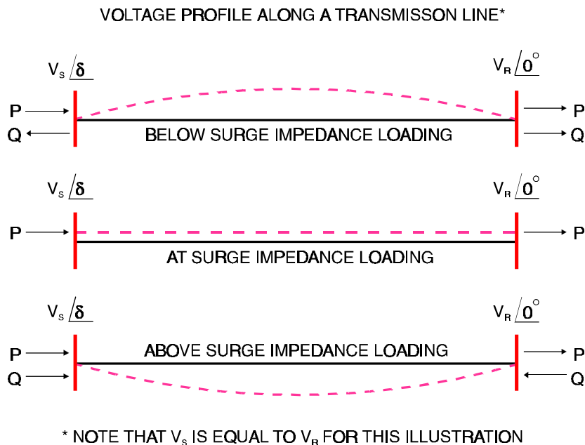
Figure 5-8 Illustration of Surge Impedance Loading
