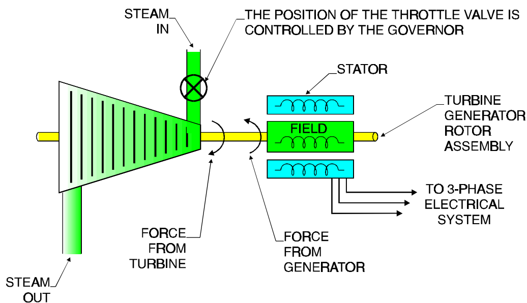
Figure 4-9 Simple System to Illustrate Governor Control
