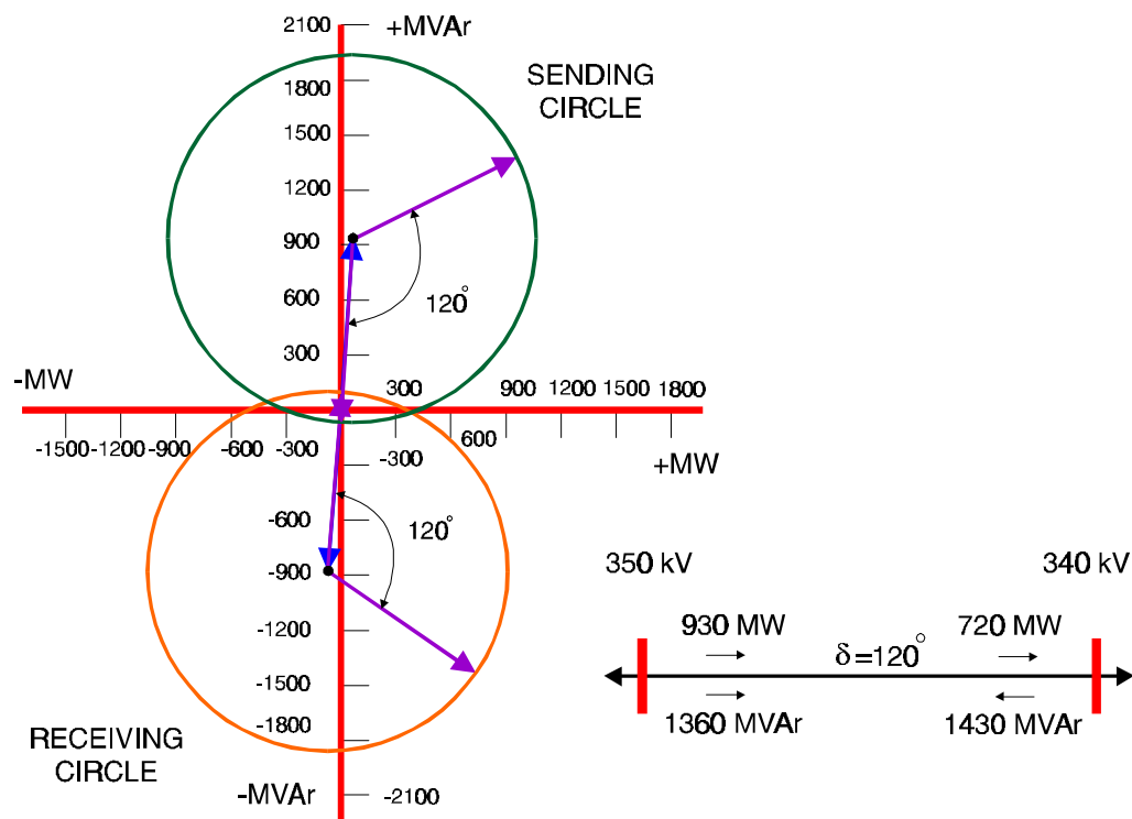
Figure 3-24 Power-Circle Diagram with a \delta of 120^\circ
