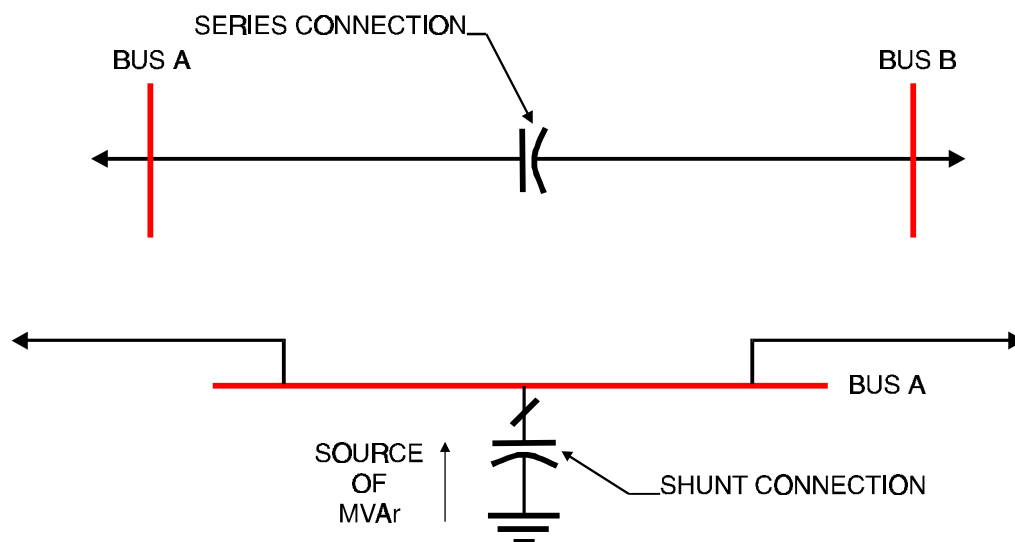
Figure 5-31 Shunt and Series Capacitors
