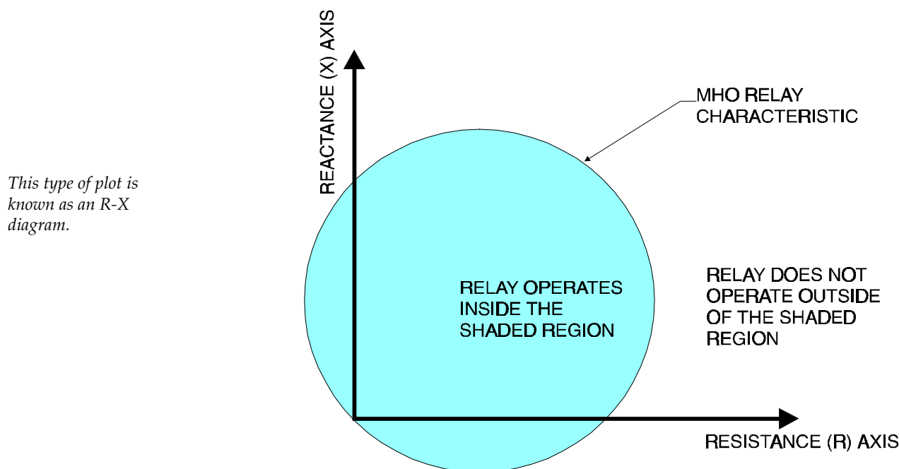
Figure 2-47 MHO Characteristic on an R-X Diagram
