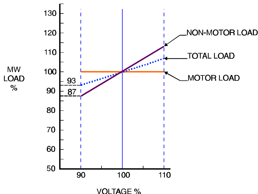
Figure 5-22 Effect of Voltage on Load Magnitude
