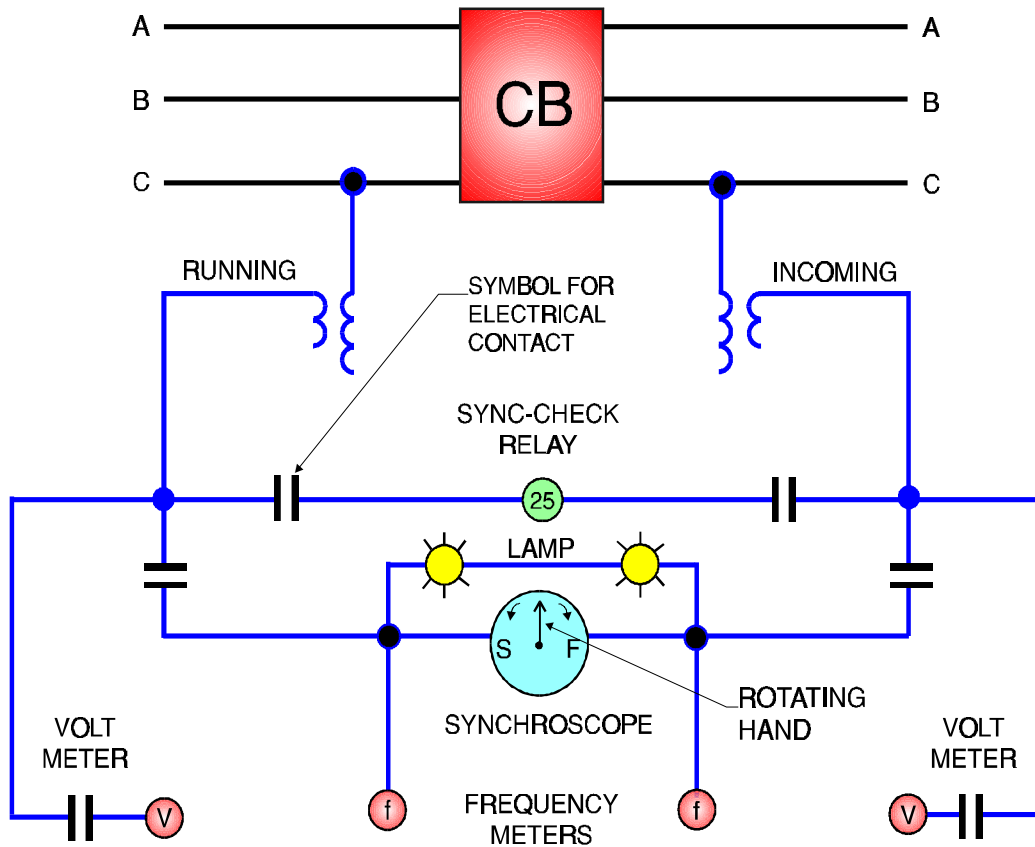
Figure 3-6 Synchrosopes & Power Angles
