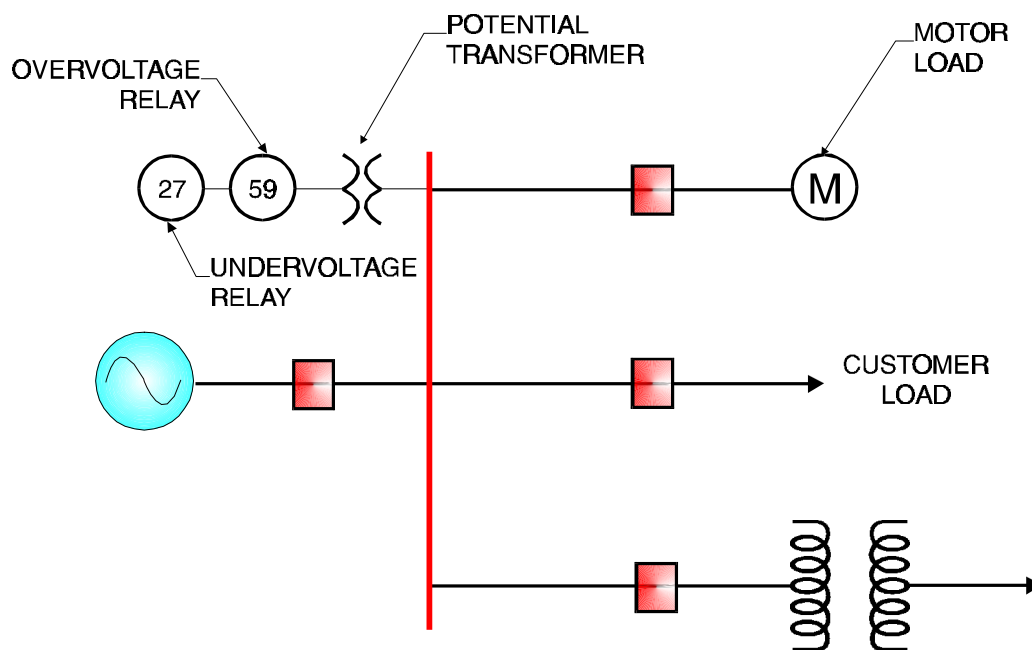
Figure 2-41 Voltage Relays on a Single-Line Diagram
