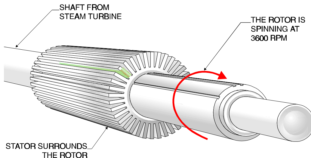
Figure 4-8 Inertia of a Steam Generator Rotor
