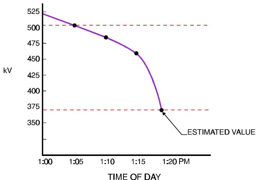
Figure 6-13 Tokyo Electric's Sin-Fuji 500 kV Substation Voltage
