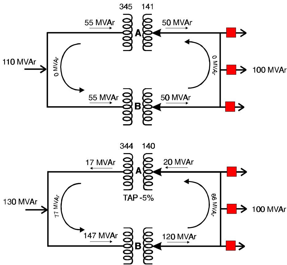
Figure 5-38 Circulating Reactive Power
