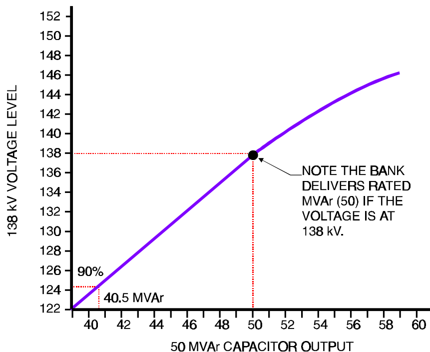
Figure 5-12 138kV Shunt Capacitor Bank Output
