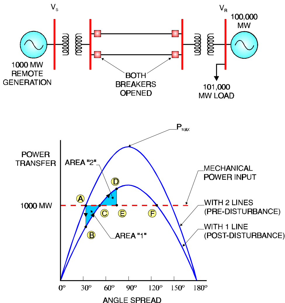
Figure 7-13 Power-Angle Curves for 1000 MW Generator Loading
