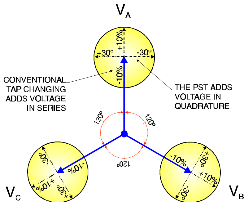
Figure 10-28 Phasor Diagram for Regulating Transformers
