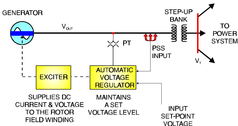
Figure 8-18 Generator Excitation System Block Diagram
