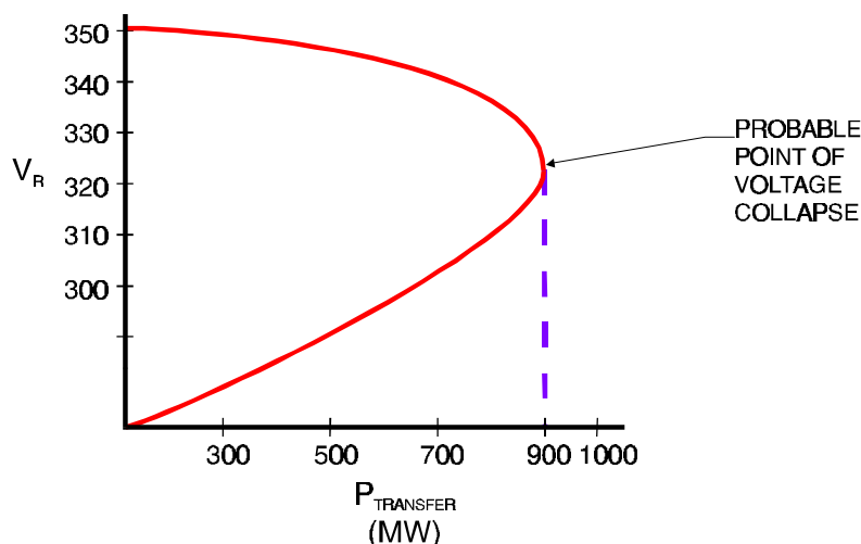
Figure 5-9 P-V Curve
