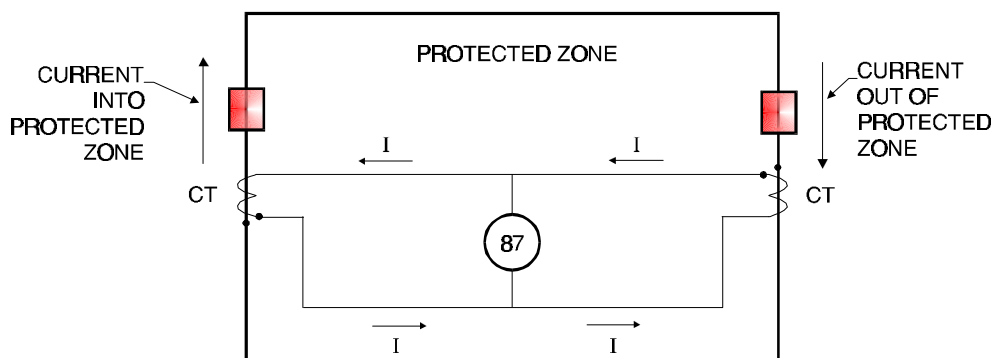
Figure 2-43 Normal Conditions for Differential Relay
