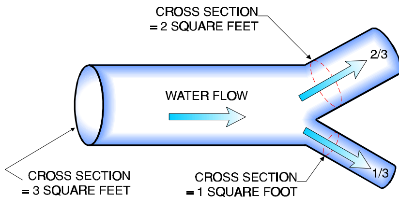
Figure 2-8 Resistance
