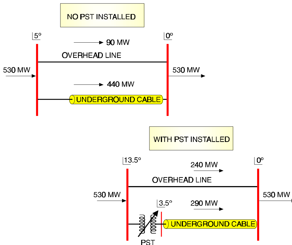
Figure 10-25 Use of a PST
