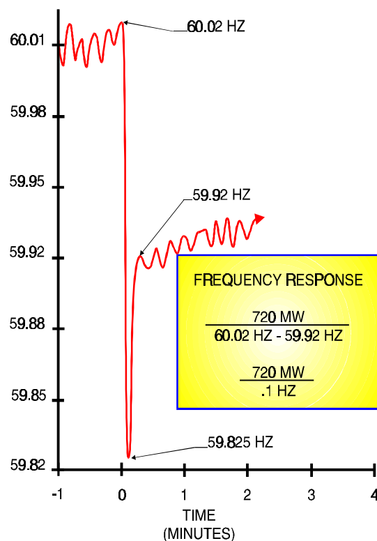
Figure 4-28 ERCOT Interconnection
