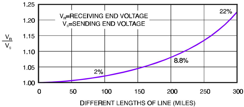
Figure 5-16 Ferranti Voltage Rise for Different Length Lines
