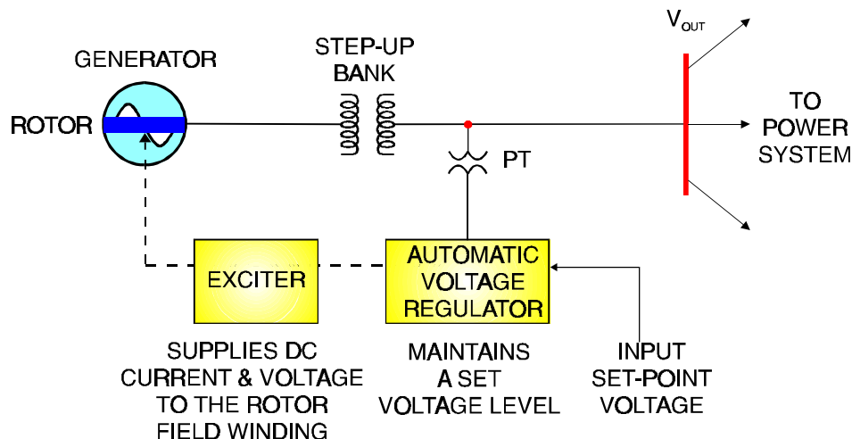
Figure 5-39 Block Diagram of a Generator Excitation System
