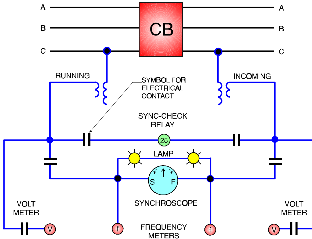
Figure 2-51 Synchronizing System for a Substation Breaker
