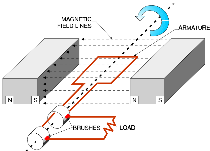
Figure 2-52 Rotating Armature - Stationary Field
