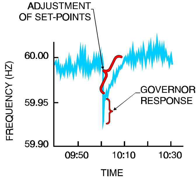
Figure 4-21 Frequency Trace
