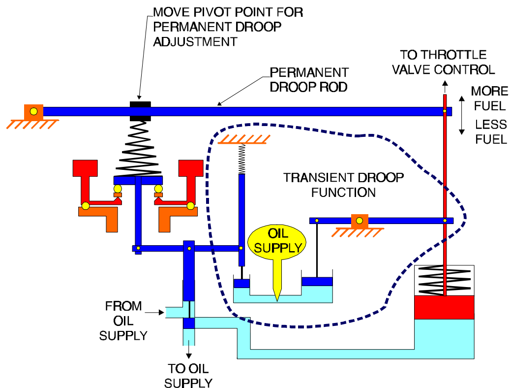
Figure 4-14 Droop in a Centrifugal Ballhead Governor
