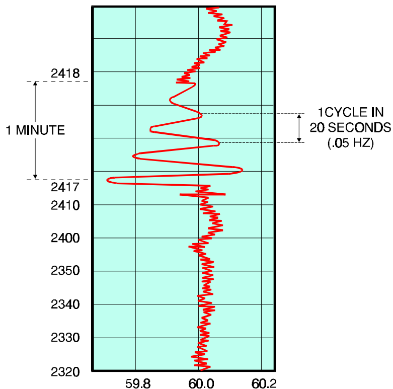
Figure 8-21 Oscillations Due to Disabling Transient Droop
