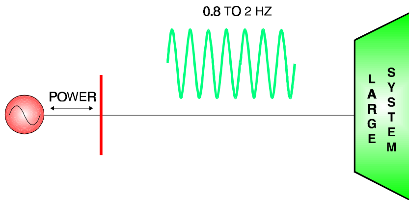
Figure 8-15 Local Mode of Oscillation
