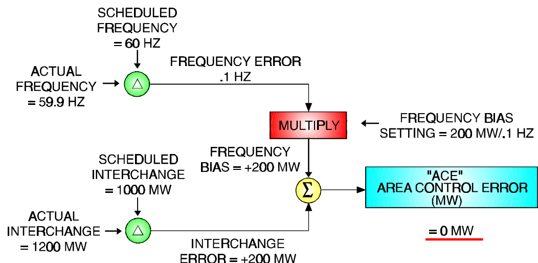
Figure 4-35 ACE for an External Generation Loss
