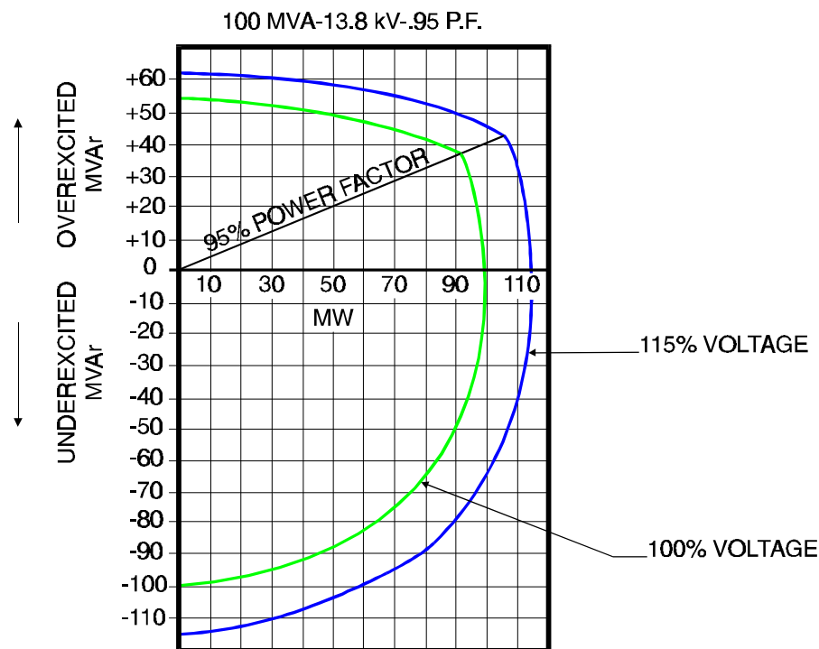
Figure 5-42 Actual Hydro Unit Reactive Capability Curve
