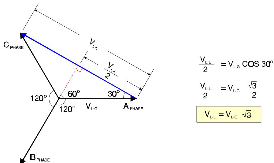
Figure 2-28 Line-to-Line & Line-to-Ground Voltages
