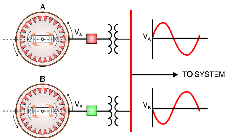
Figure 7-2 Out-of-Step-Generator Closing
