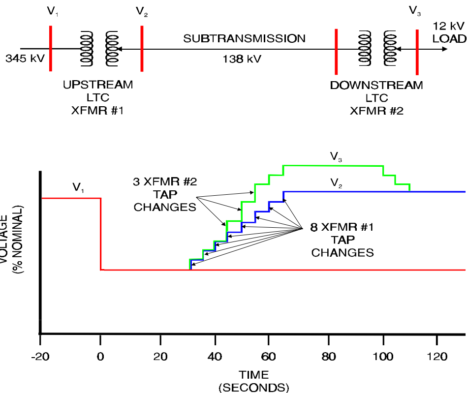
Figure 6-12 Tap Changers and Load Overshoot 1
