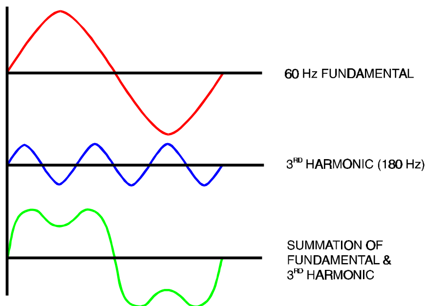
Figure 9-3 Summation of Fundamental with Harmonic
