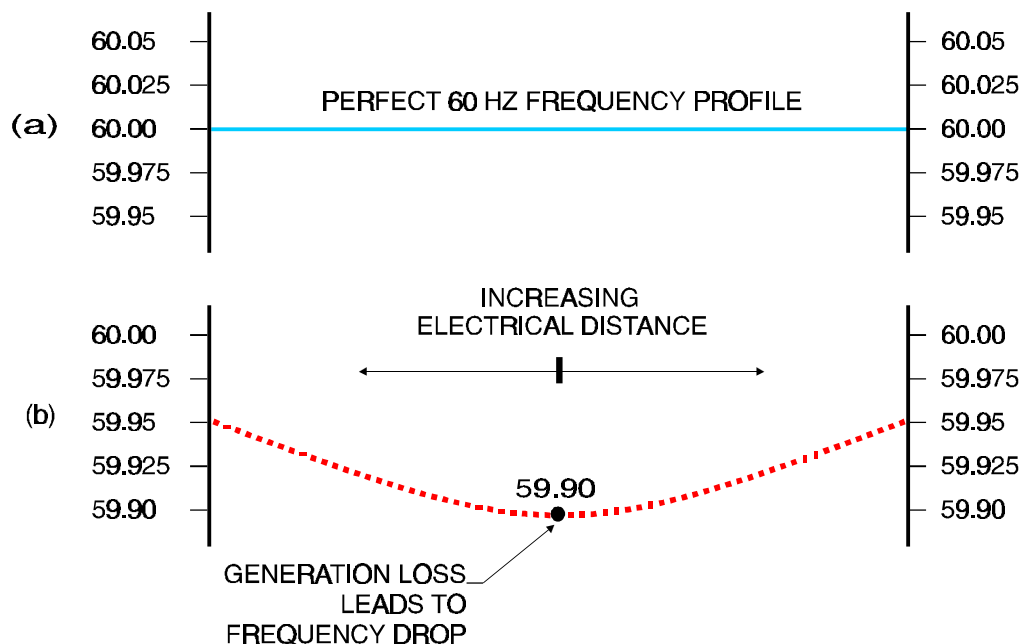
Figure 4-52 Distance and Frequency Undershoots
