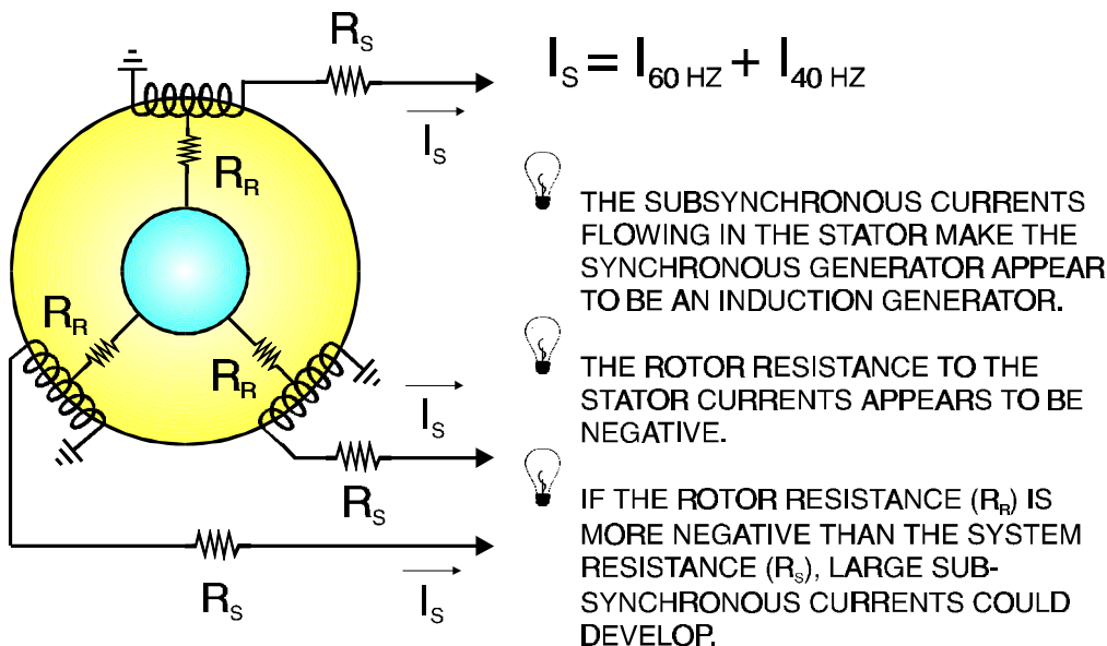
Figure 9-20 SSR Scenario III - Induction Generator Effect
