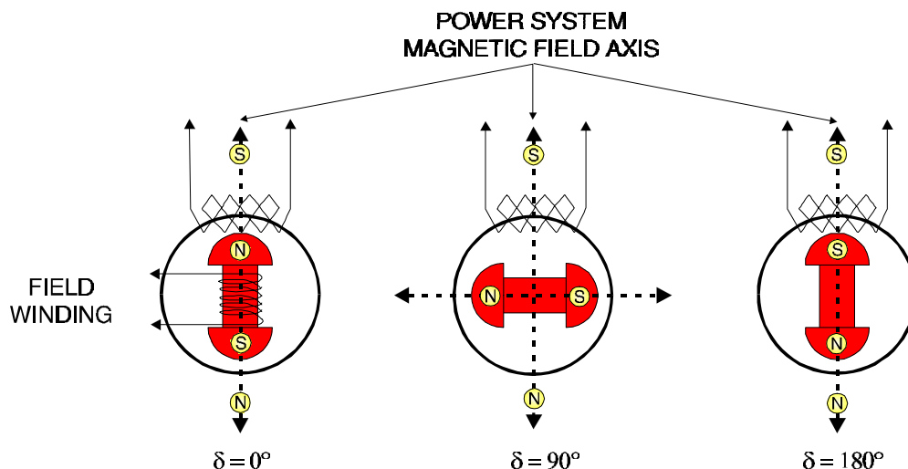
Figure 8-23 Increasing Angle Spread
