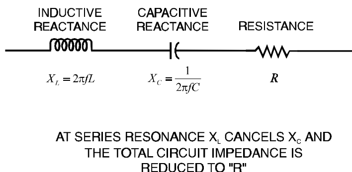
Figure 9-10 Series Resonance
