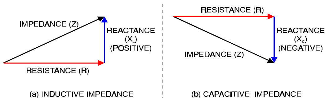
Figure 2-24 The Impedance Triangle
