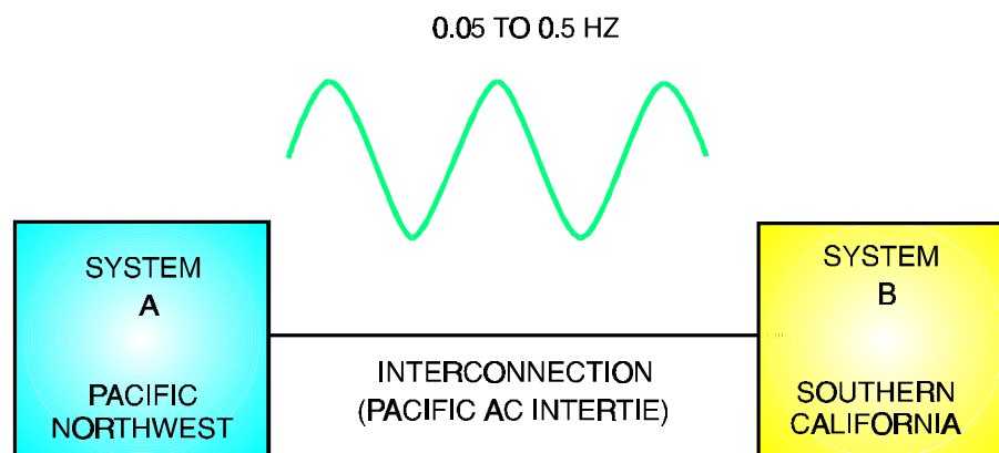
Figure 8-13 Inter-Area Mode of Oscillation
