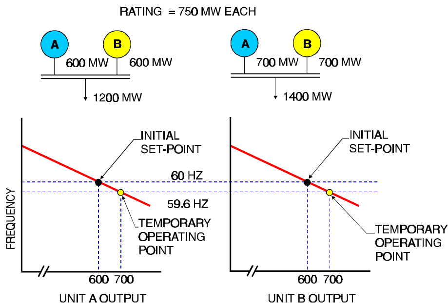
Figure 4-23 Load Sharing - Same Unit Ratings - Same Droop
