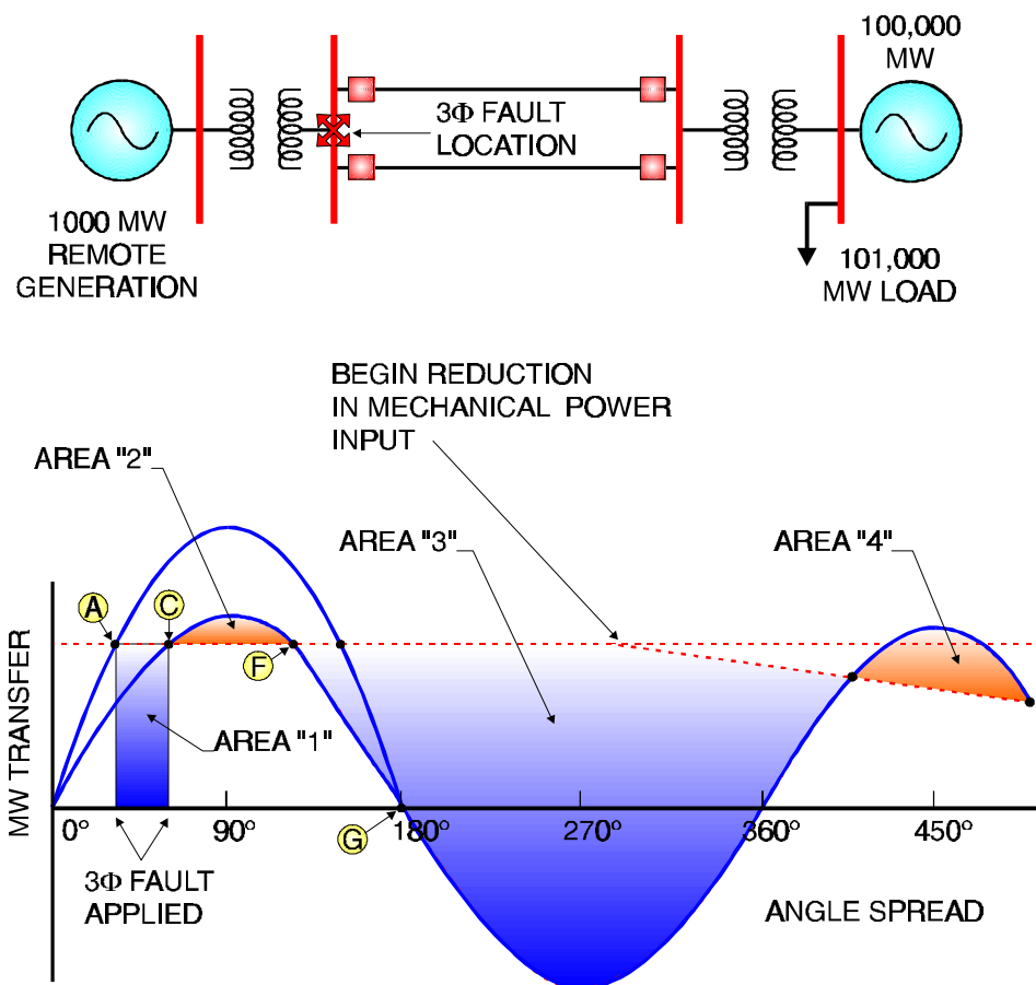
Figure 7-17 Extended Power-Angle Curve
