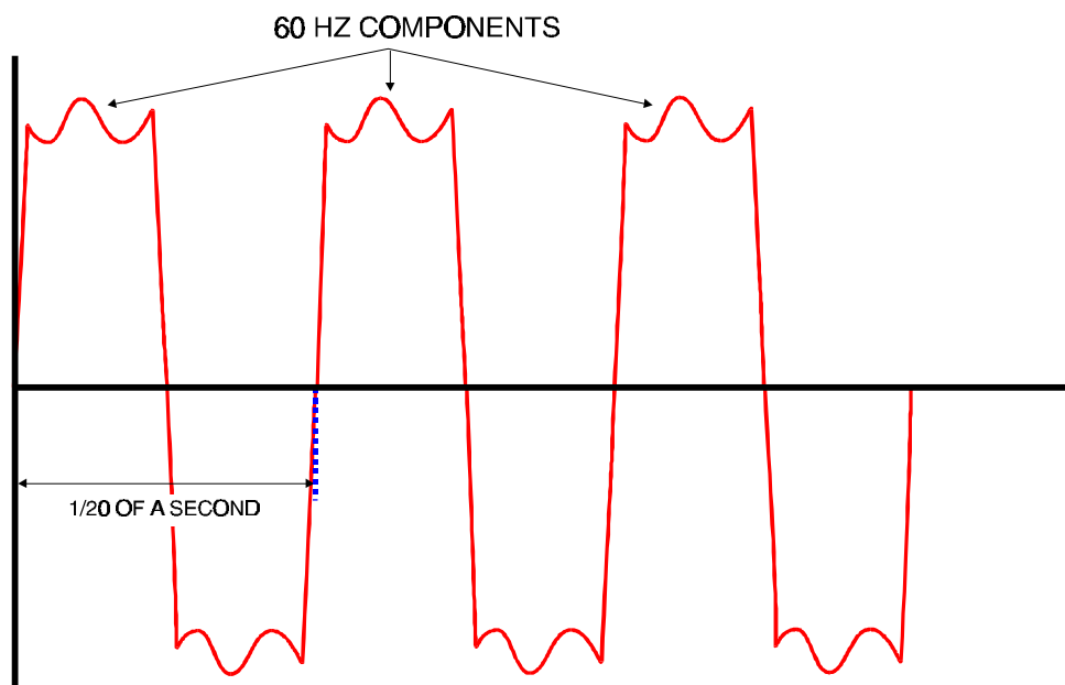
Figure 9-31 Ferroresonance Voltage Waveform
