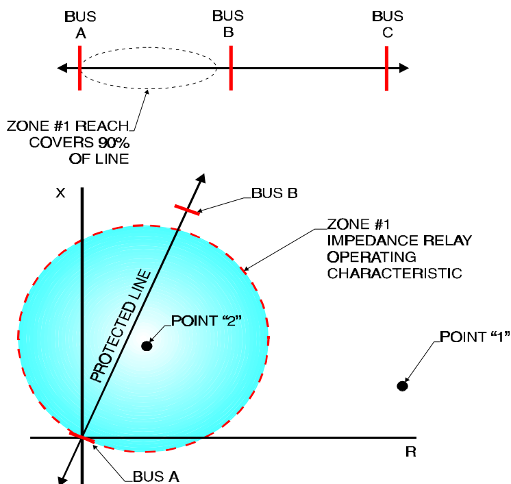
Figure 7-26 R-X Diagram for an Impedance Relay
