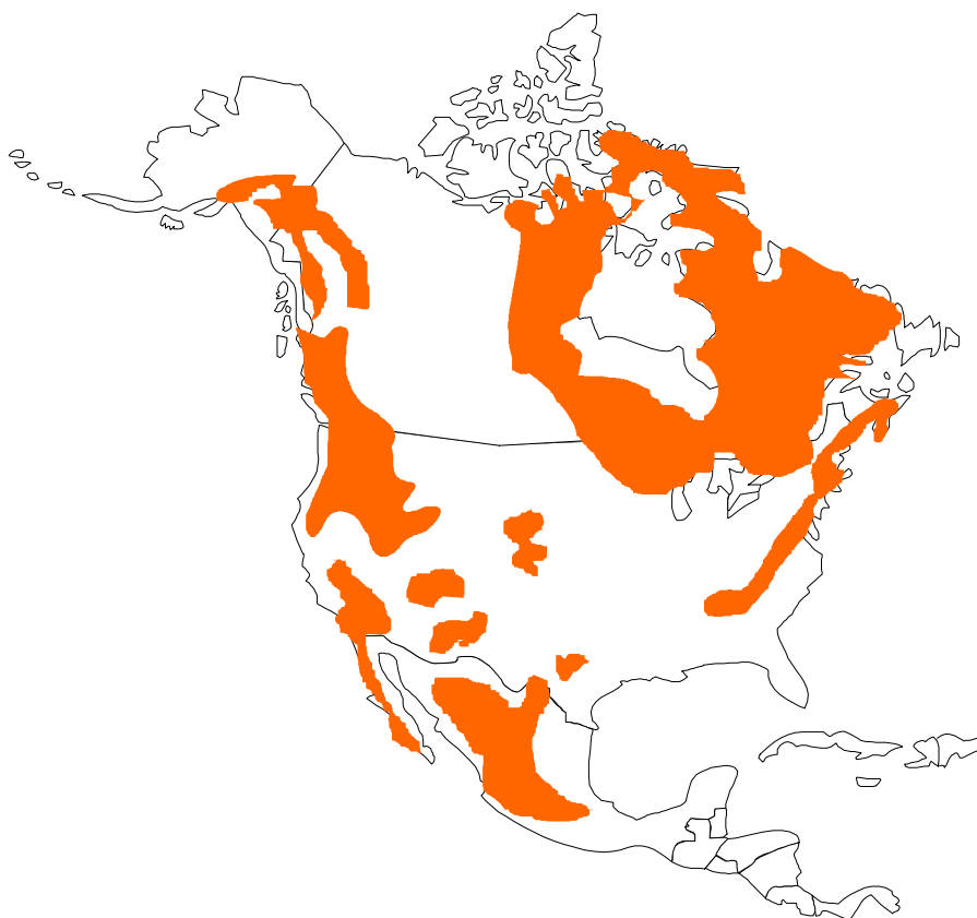
Figure 9-37 Igneous Rock Locations in North America
