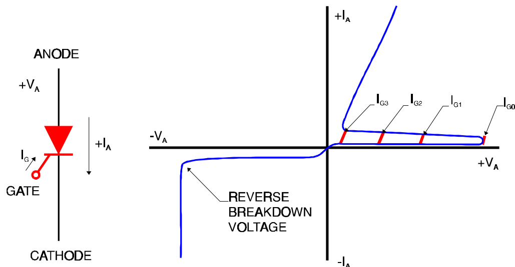
Figure 2-76 Thyristor Symbol & Operation
