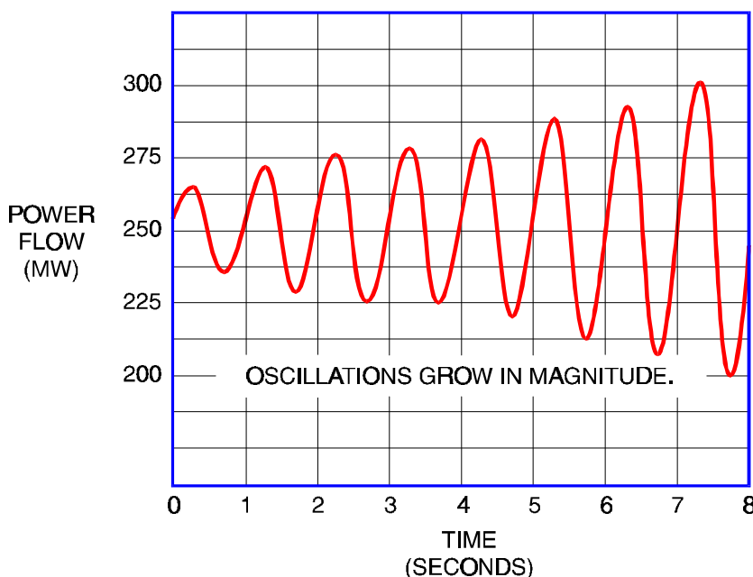
Figure 8-7 Negatively Damped Power Oscillations
