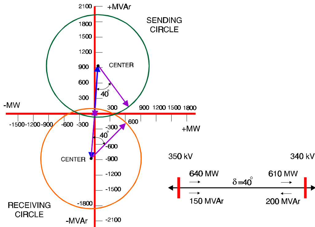
Figure 3-22 Power-Circle Diagram with a \delta of 40^\circ
