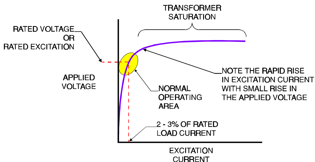
Figure 5-28 Transformer Saturation Curve
