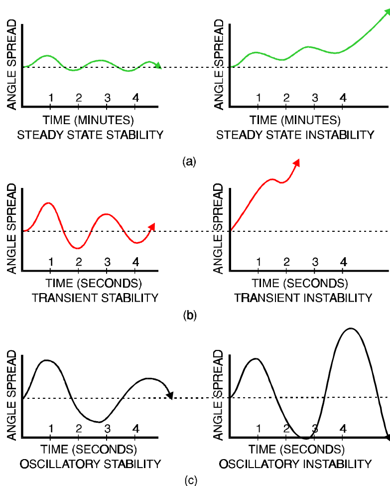
Figure 1-3 Types of Stability / Instability
