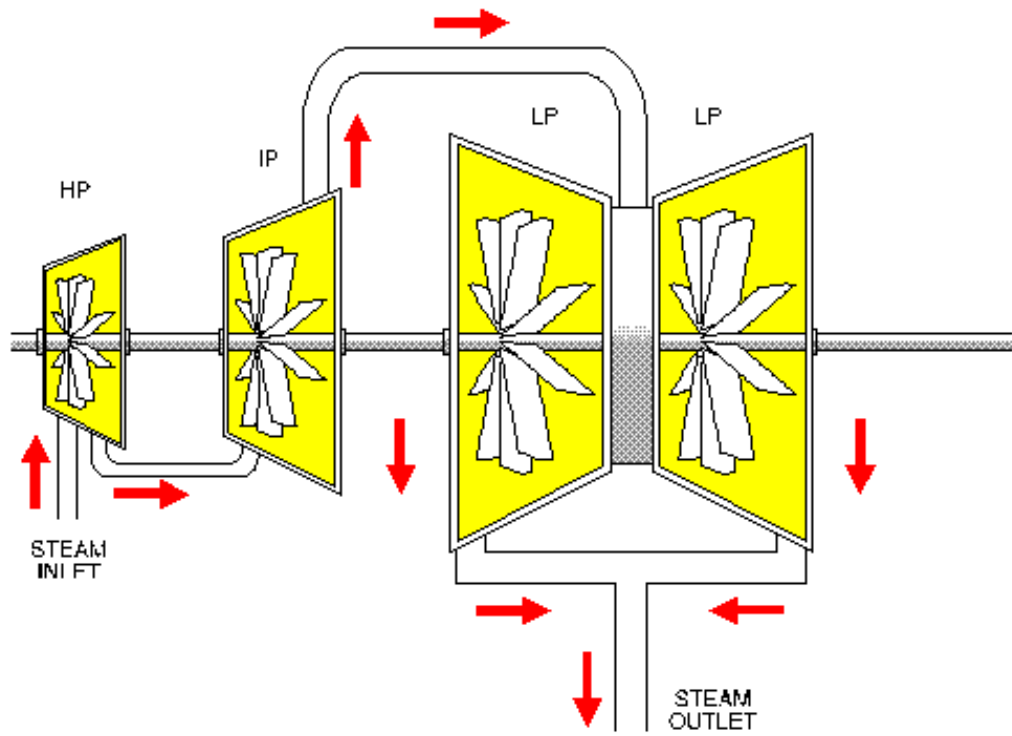
Figure 2-62 Steam Turbine Stages
