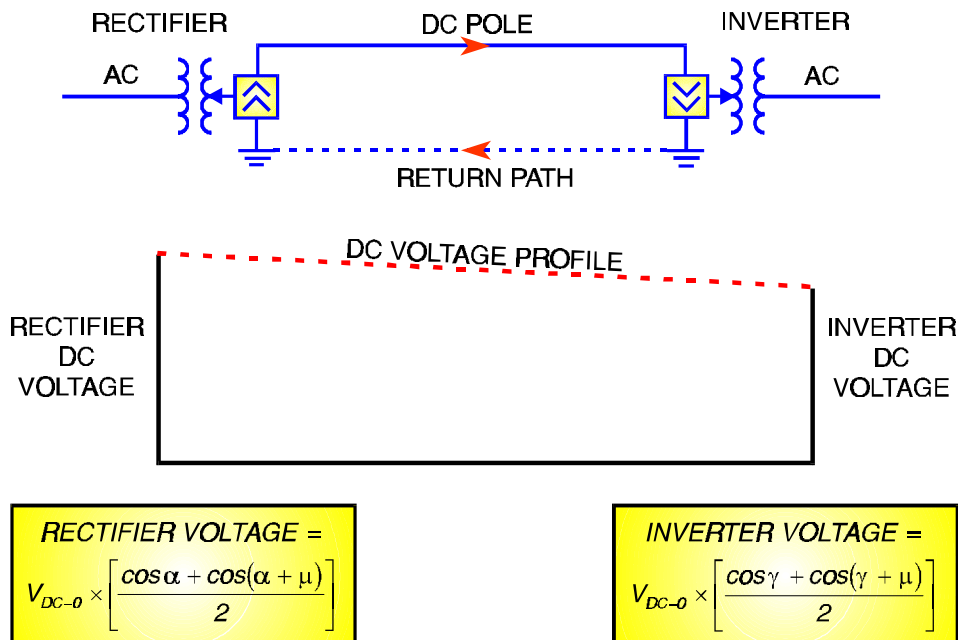
Figure 10-24 HVDC Power Flow Control
