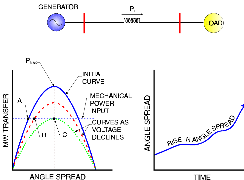
Figure 7-11 Manual Excitation and Steady State Instability
