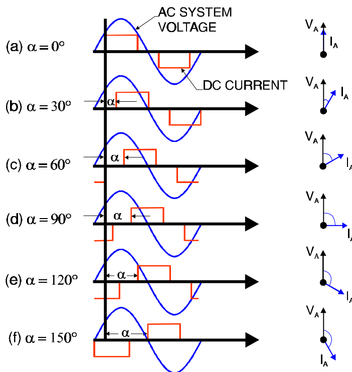
Figure 10-23 Phase Displacement in an HVDC Converter
