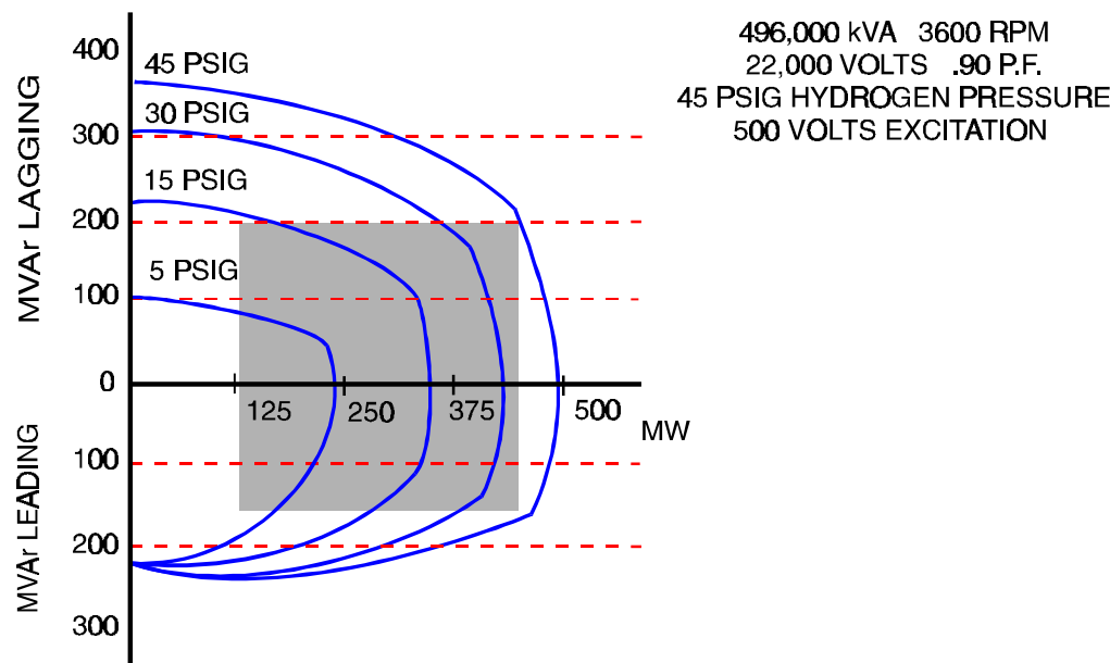
Figure 5-43 Reactive Production Limitations
