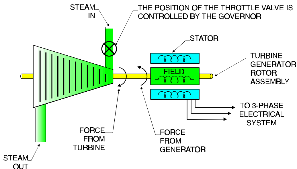
Figure 1-2 Simple System to Illustrate Governor Control
