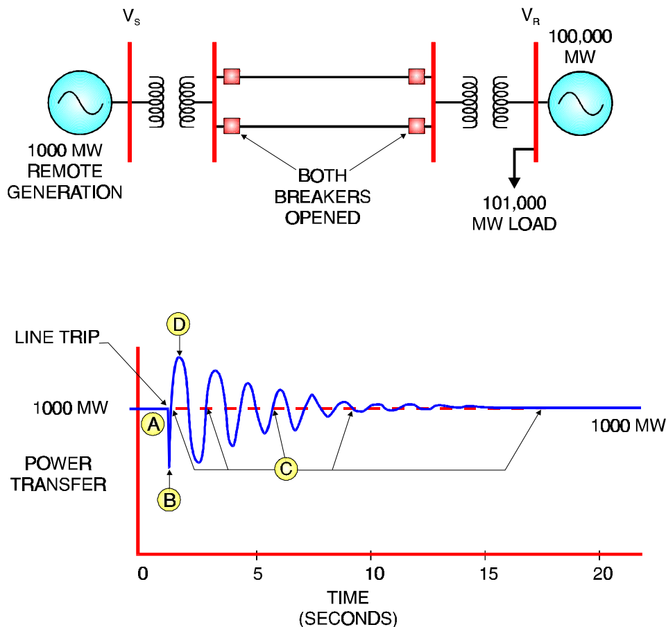
Figure 7-14 Strip Chart Equivalent of Figure 7-13
