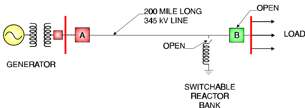
Figure 5-18 Self Excitation of a Generator
