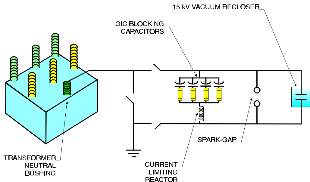
Figure 9-44 Connection Diagram for Neutral Blocking Capacitor
