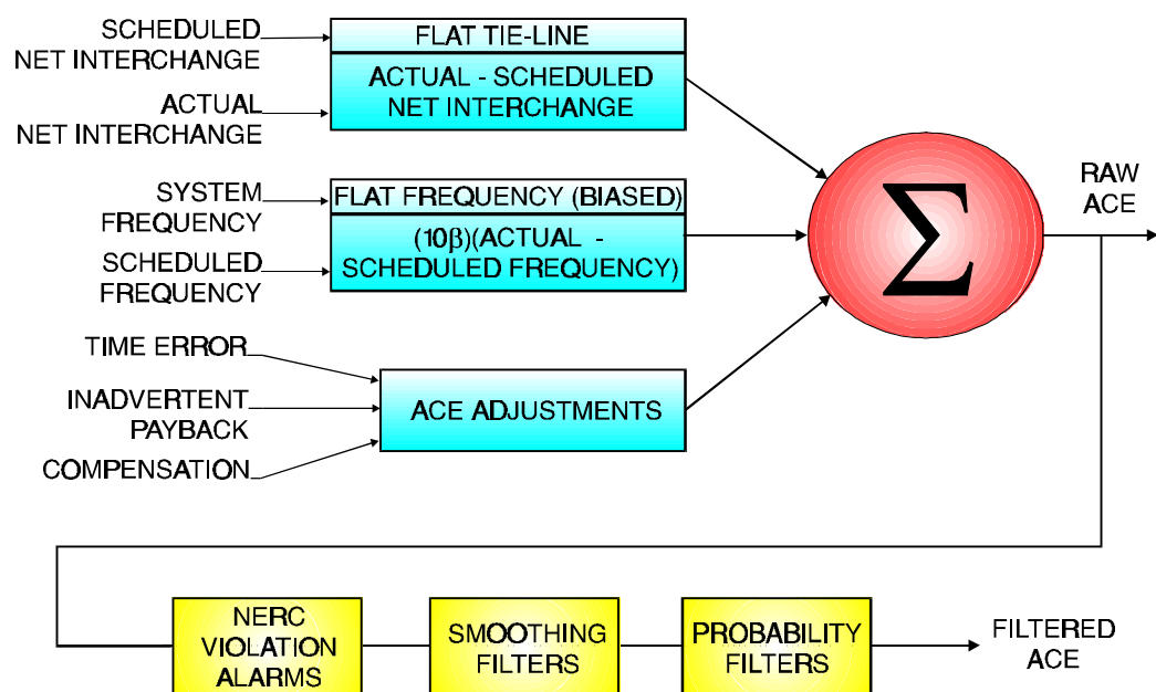
Figure 4-37 A Simple Model of a Control Area AGC System
