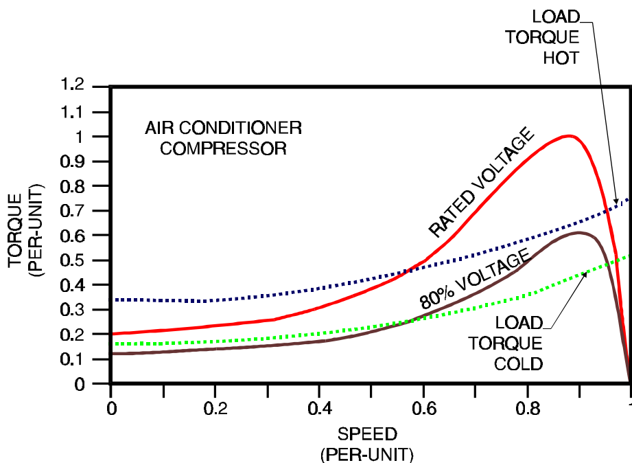
Figure 6-25 Air-Conditioner Compressor Load Torque/Speed Curve
