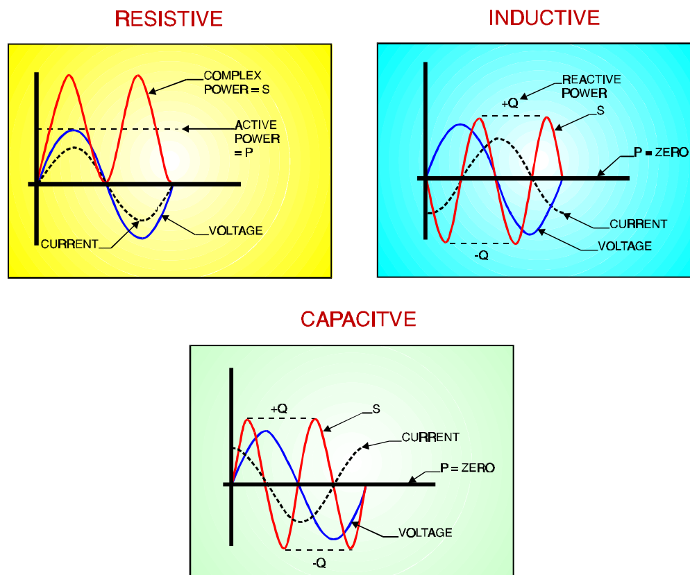
Figure 5-2 Reactive Power Storage
