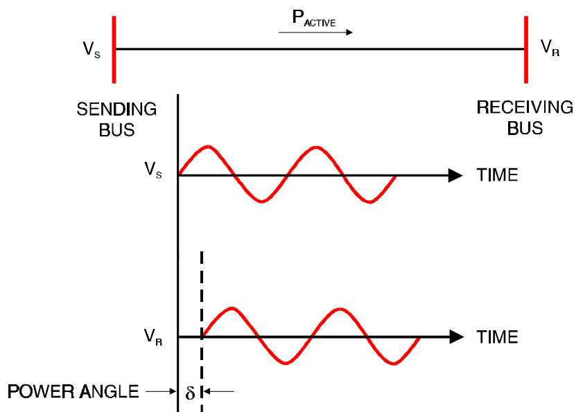
Figure 3-3 Measurement of the Power Angle ( \delta )
