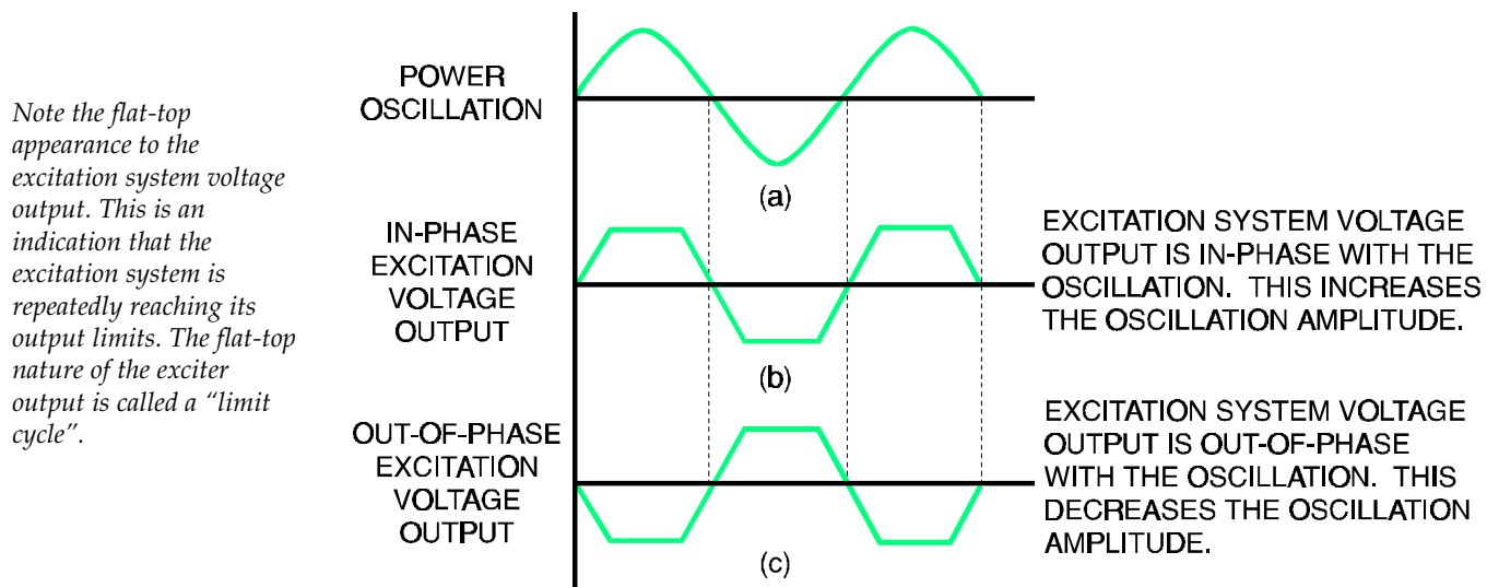
Figure 8-19 Exciter Output Effect on Oscillations
