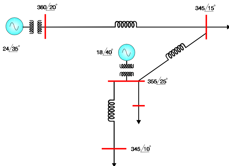
Figure 7-1 Stability: Voltage and Angle
