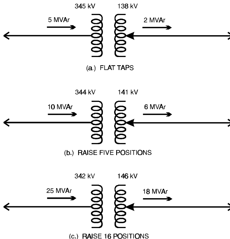
Figure 5-37 Tap Change and Reactive Power
