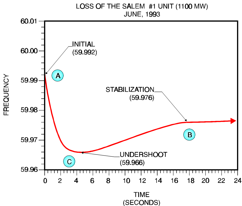
Figure 4-50 Eastern Interconnection Expanded Frequency Plot
