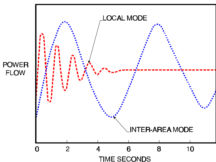
Figure 8-17 Comparison of Local and Inter-Area Mode Oscillations
