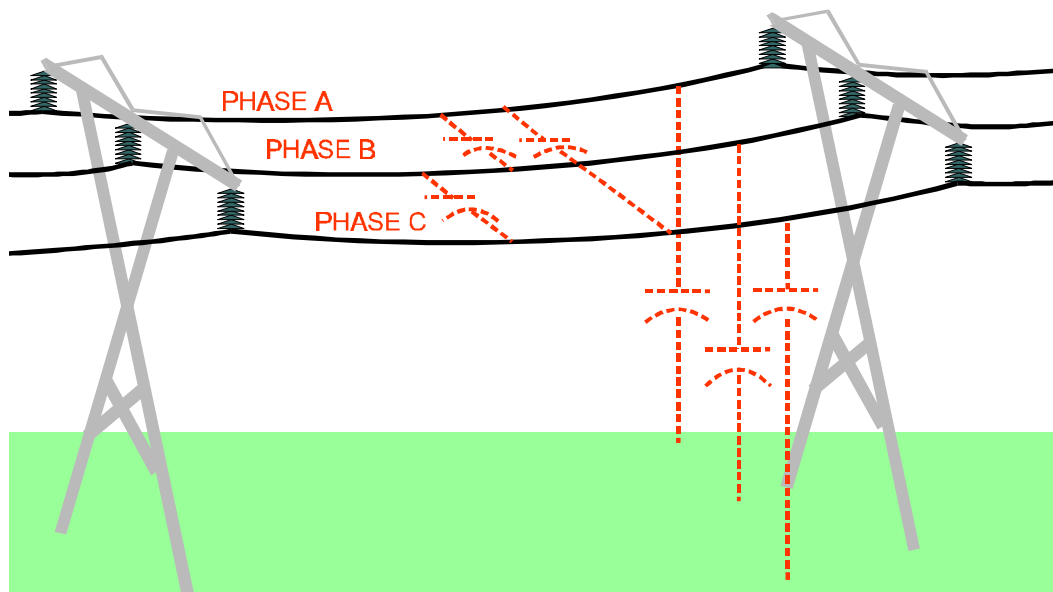
Figure 2-74 Natural Capacitance of a Transmission Line
