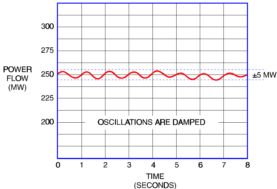
Figure 8-5 Normal (Positively) Damped Power Oscillations
