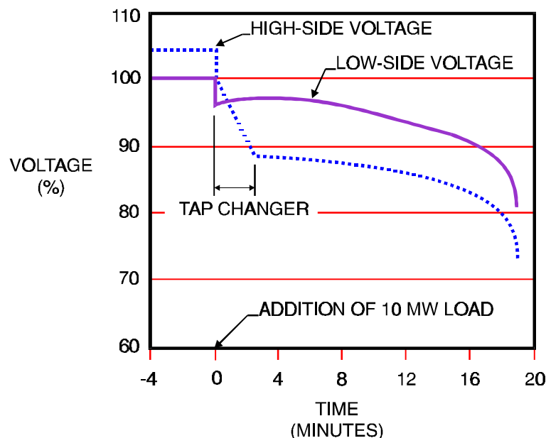
Figure 6-15 High and Low-Side Voltages After 10 MW Load is Added
