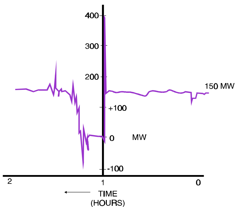
Figure 6-22 Kitimat-Minette Line Flow
