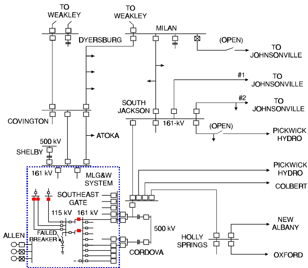
Figure 6-26 TVA and MLG&W Power Systems
