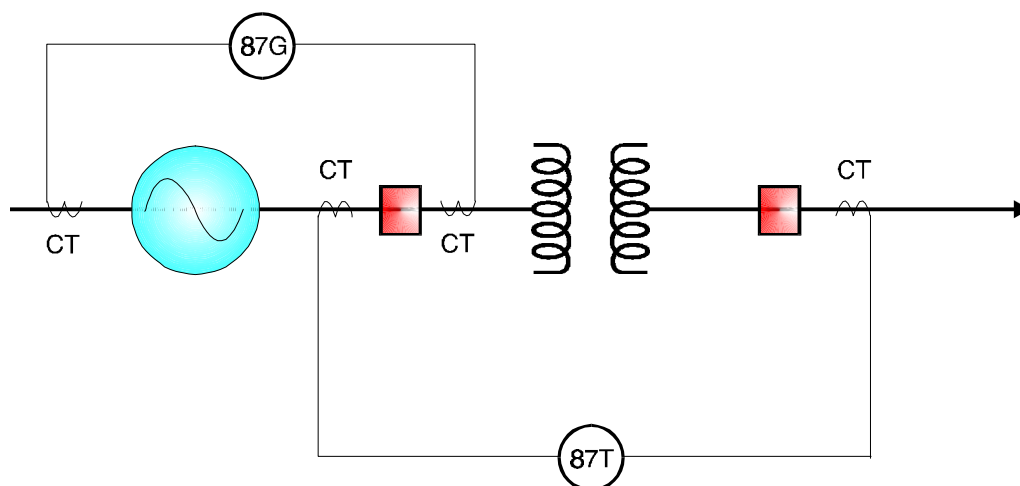
Figure 2-46 Single-line Diagram with Differentials
