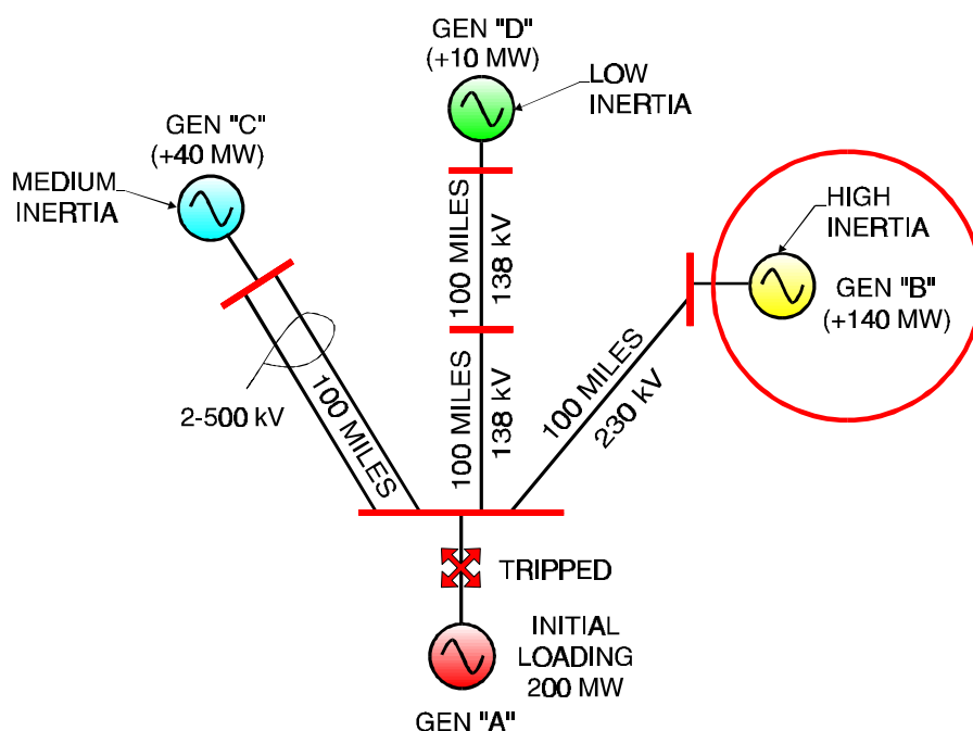
Figure 4-56 Stage #2 - The Inertial Stage
