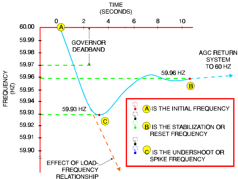
Figure 4-48 Expanded Plot of a Simulated Frequency Disturbance
