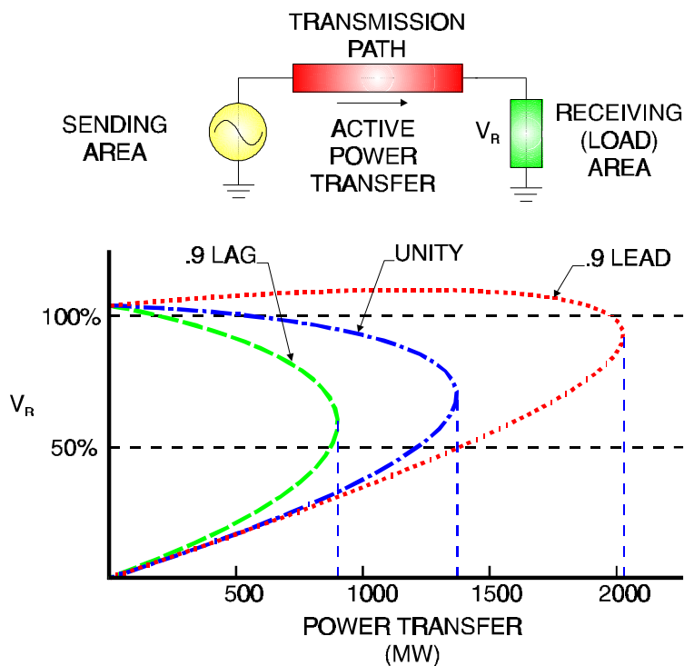
Figure 6-9 Shunt Capacitor Effect on P-V Curves
