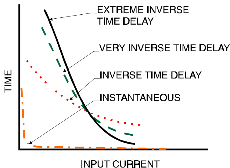
Figure 2-42 Overcurrent Relay - Time Characteristic Curves
