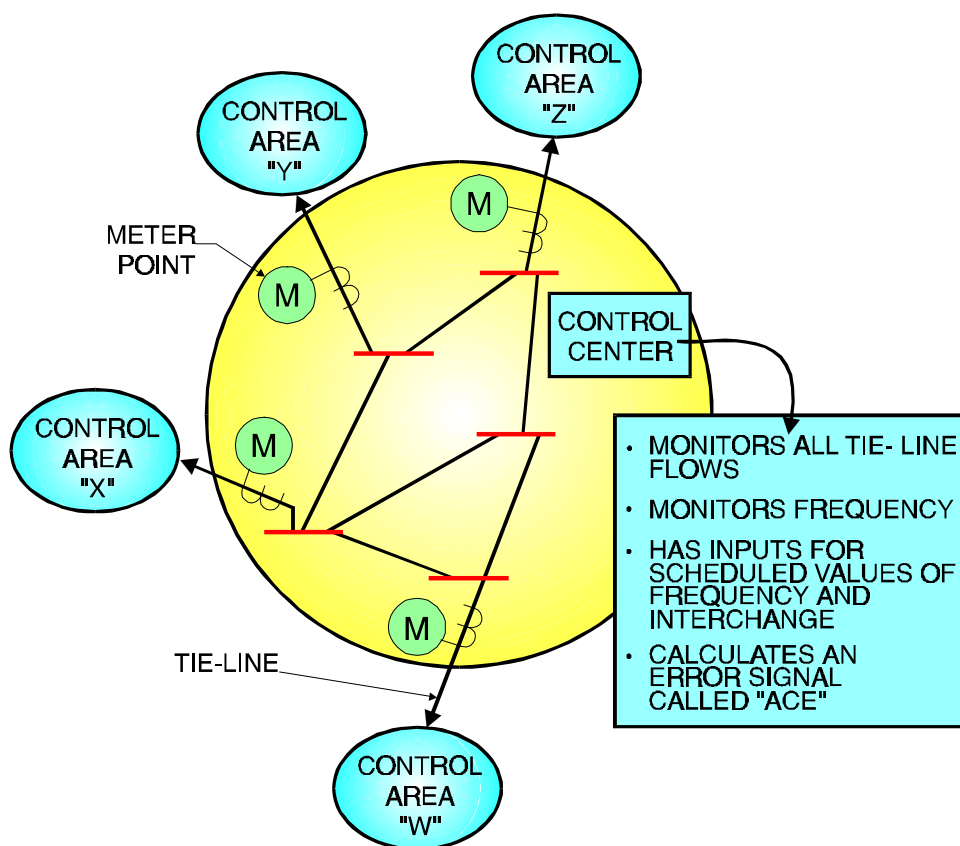
Figure 4-29 Definition of a Control Area
