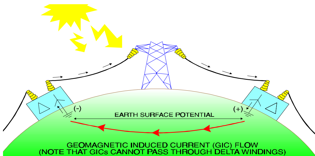
Figure 9-38 Flow of GIC
