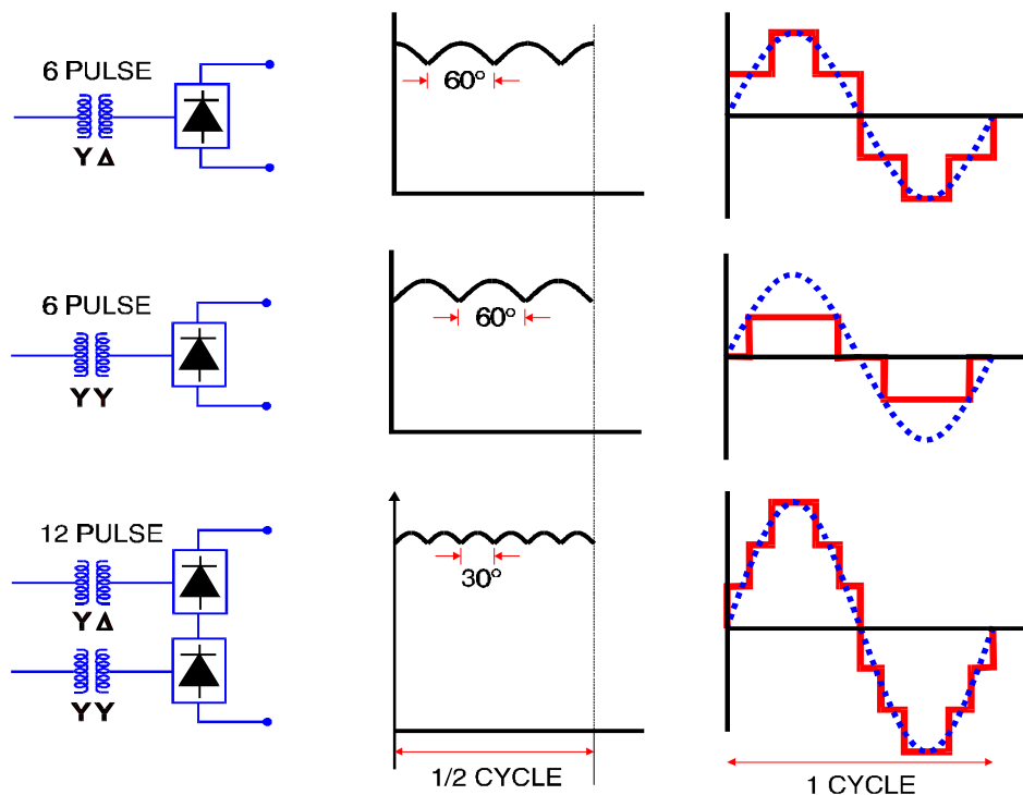
Figure 10-15 Benefits of Multi-Pulse Operation
