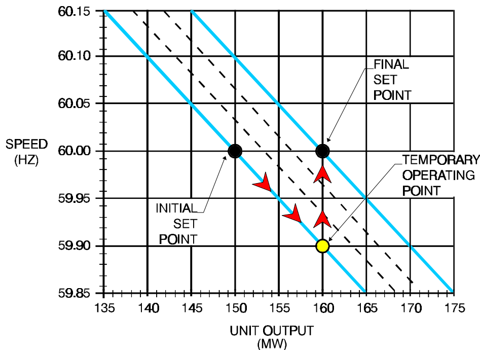
Figure 4-18 Changing the Set-Point to 160 MW @ 60 HZ
