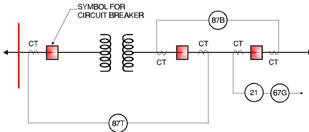
Figure 2-39 Single-Line Diagram Using IEEE Device Numbers
