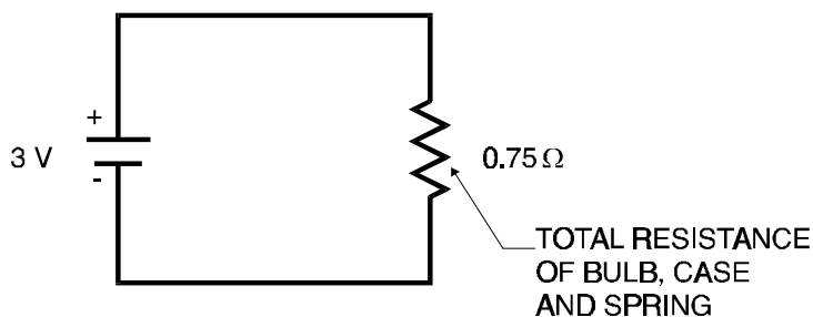
SIMPLIFIED FLASHLIGHT CIRCUIT
