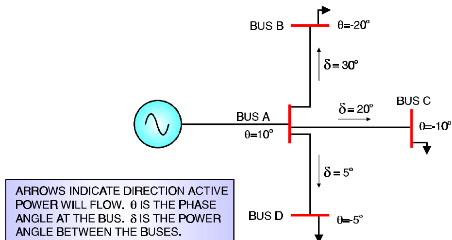
Figure 3-5 Power System Phase & Power Angles
