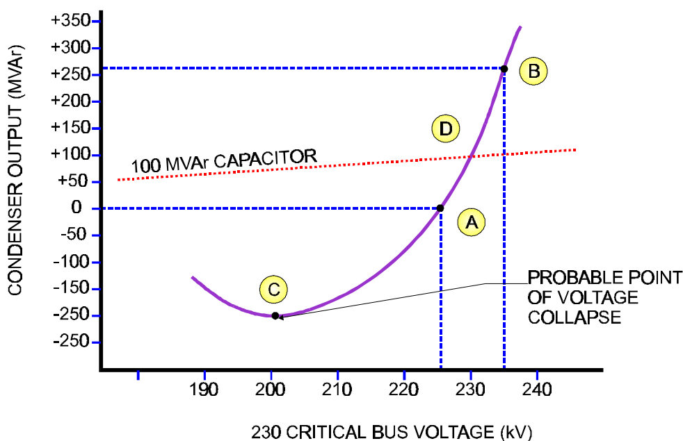
Figure 6-18 The V-Q Curve
