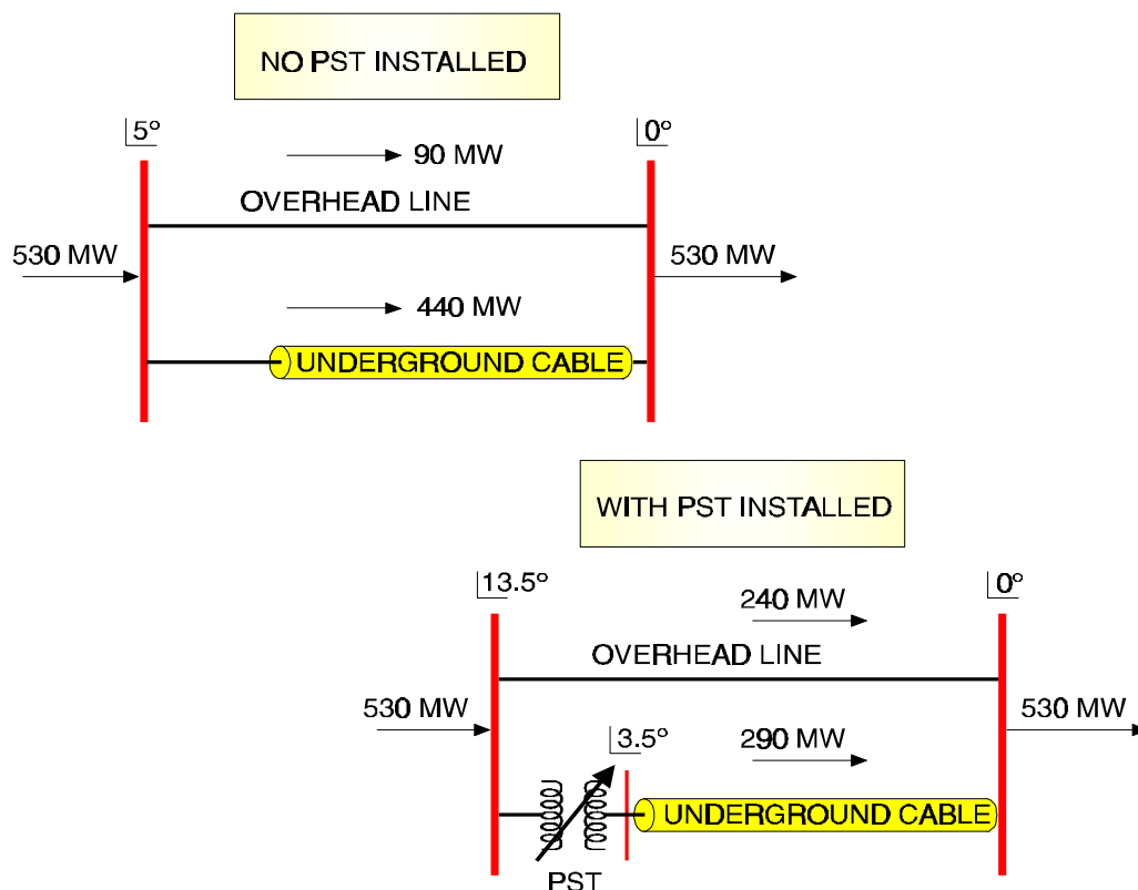
Figure 3-15 Use of Phase Shifting Transformer
