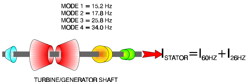
Figure 9-18 SSR Scenario I - Torsional Interaction
