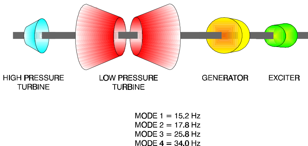
Figure 9-17 Turbine/Generator Shaft Modes
