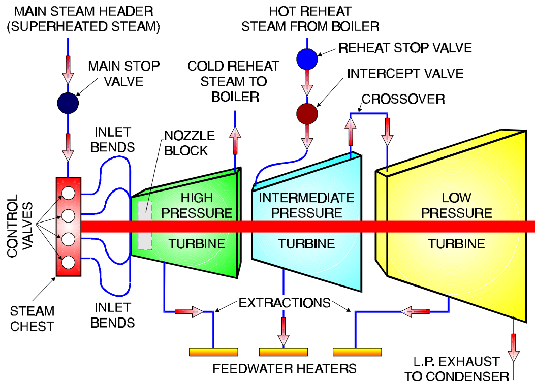
Figure 2-63 Turbine Components
