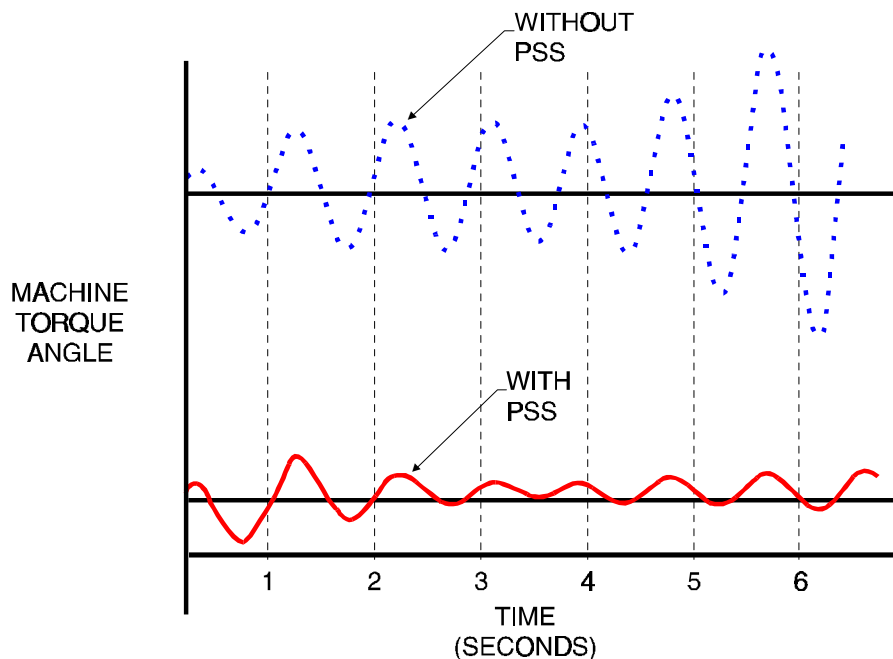
Figure 8-20 Power Oscillations With and Without PSS In-Service
