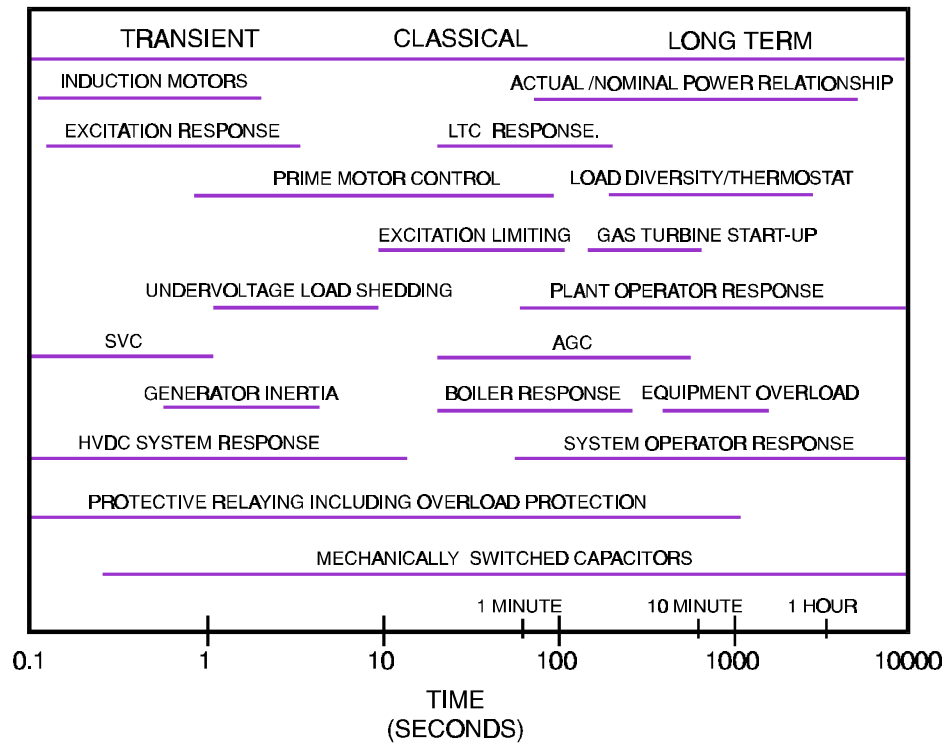
Figure 6-29 Time Frames for Voltage Collapse
