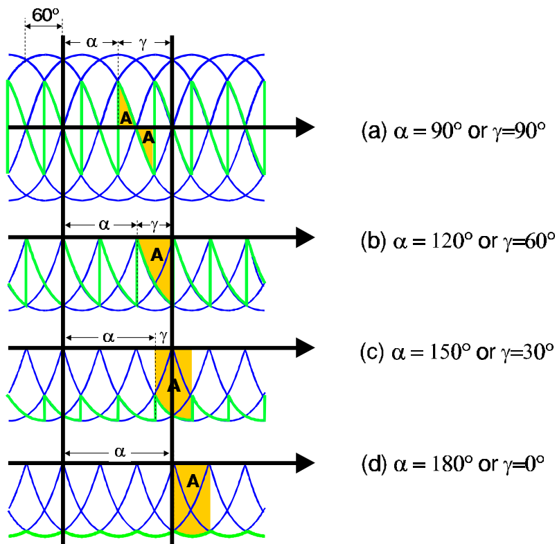
Figure 10-22 Six-Pulse Converter Ignition Delay Angles of 90^\circ - 180^\circ
