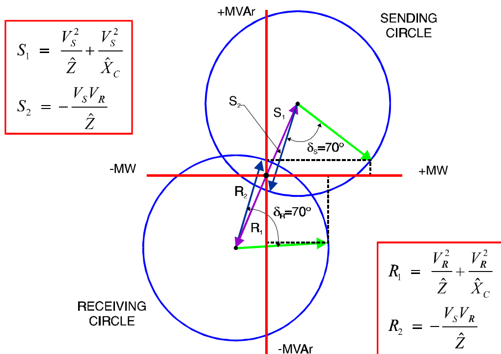
Figure 3-19 Sending & Receiving Ends Plots
