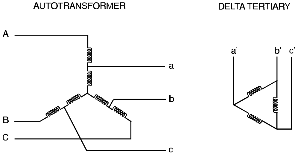
Figure 9-7 Autotransformer with Delta Tertiary
