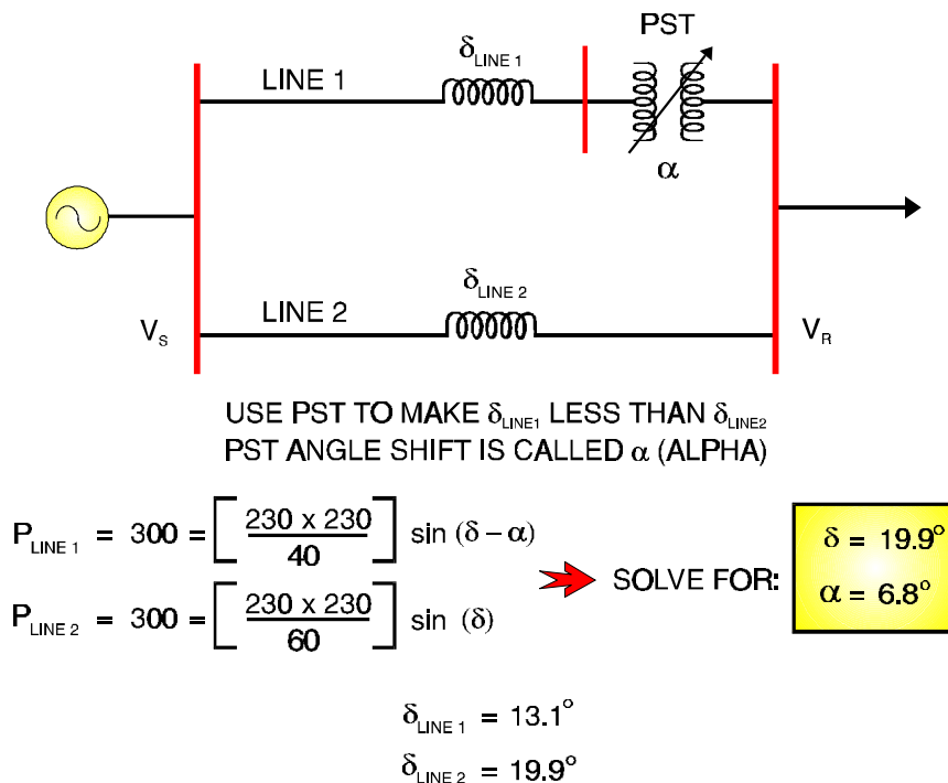
Figure 10-30 PST Operation - Part II
