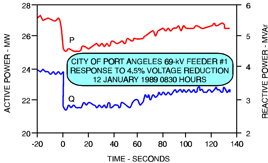
Figure 5-23 Effect on Time on Load Magnitude
