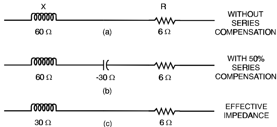
Figure 9-12 Use of Series Capacitors
