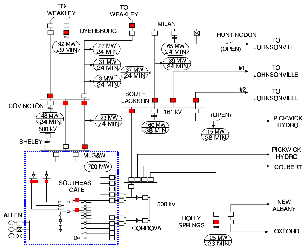
Figure 6-27 Post Disturbance System Conditions
