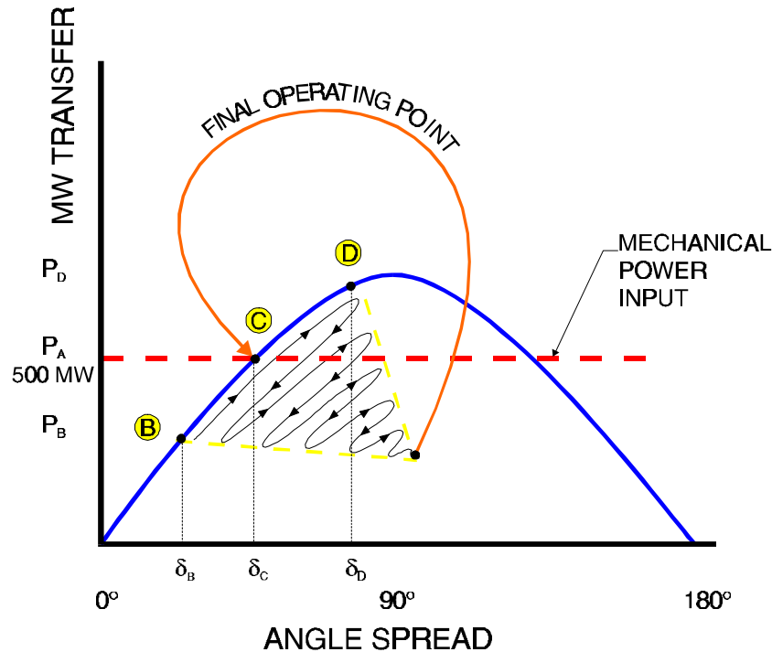
Figure 7-22 Illustrating Oscillations on a Power-Angle Curve
