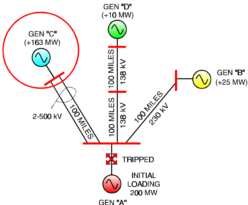
Figure 4-55 Stage #1 - The Electromagnetic Energy Stage
