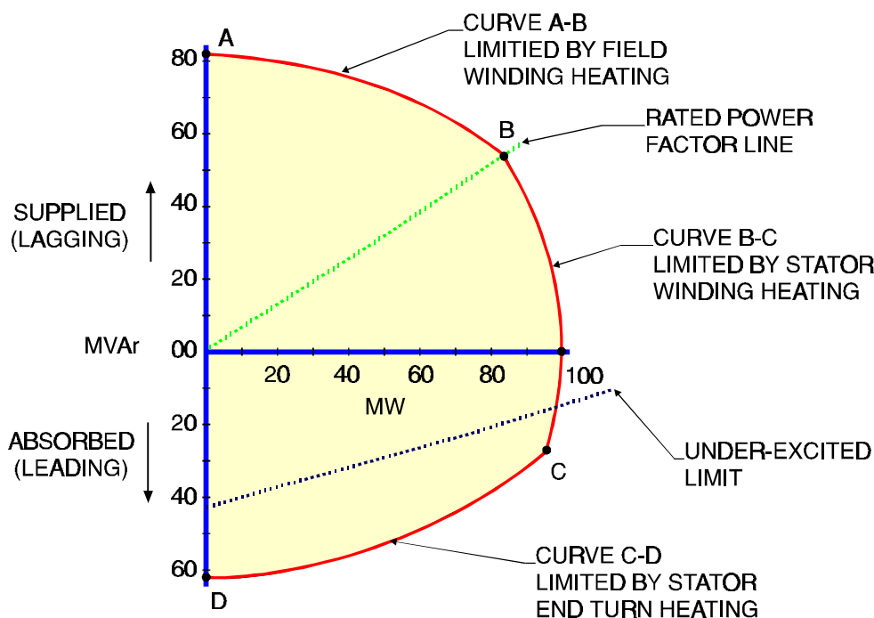
Figure 5-40 Reactive Capability Curve
