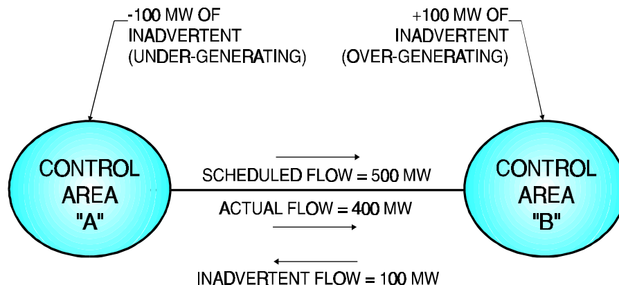
Figure 4-31 Inadvertent Interchange
