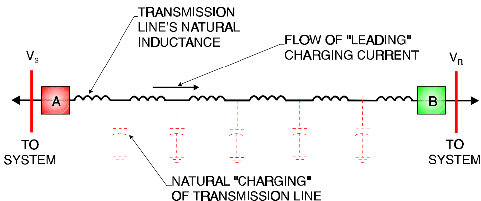
Figure 5-13 Charging Current Flowing into an Open-Ended Line
