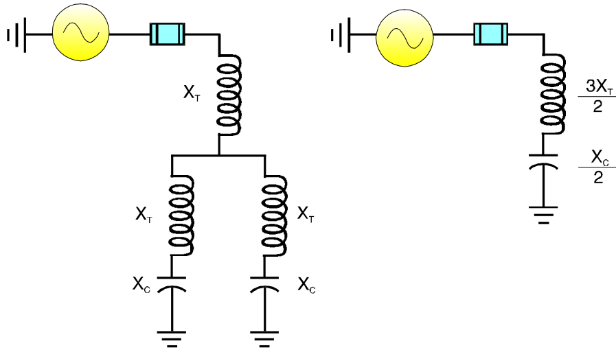
Figure 9-25 Circuit Phase "C" is Closed
