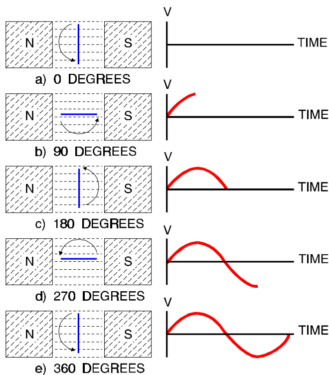
Figure 2-53 Armature Rotation & Voltage
