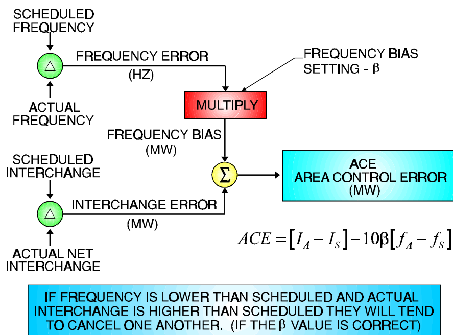
Figure 4-34 Tie-Line Bias Control ACE Calculation
