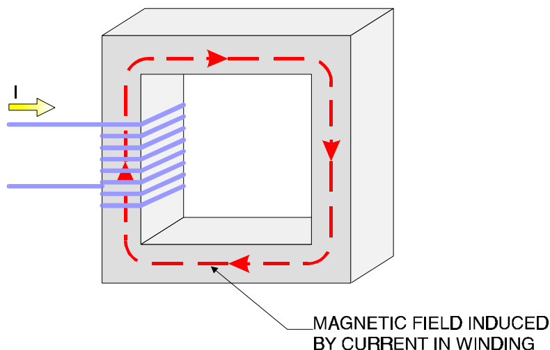
Figure 2-22 Magnetic Field in an Iron-Core
