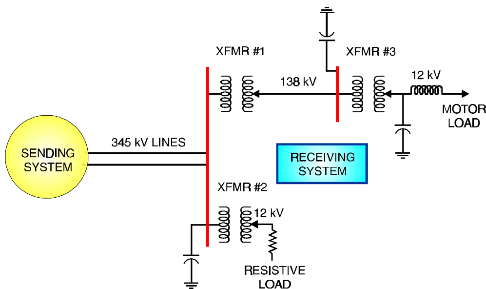
Figure 6-11 Radial Power System for Long Term Voltage Collapse
