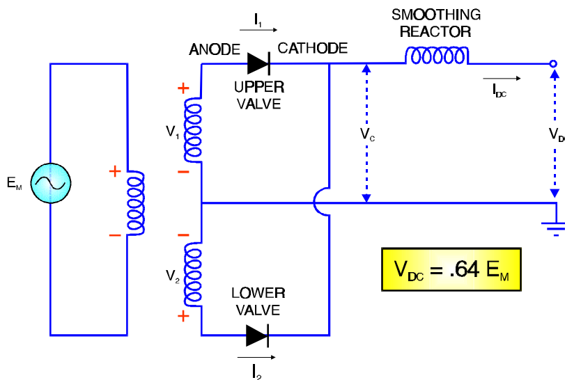
Figure 10-7 Single-Phase Converter
