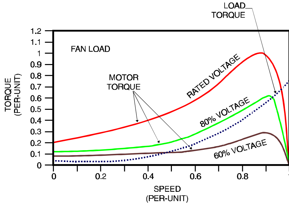
Figure 6-24 Fan Load Torque/Speed Curve
