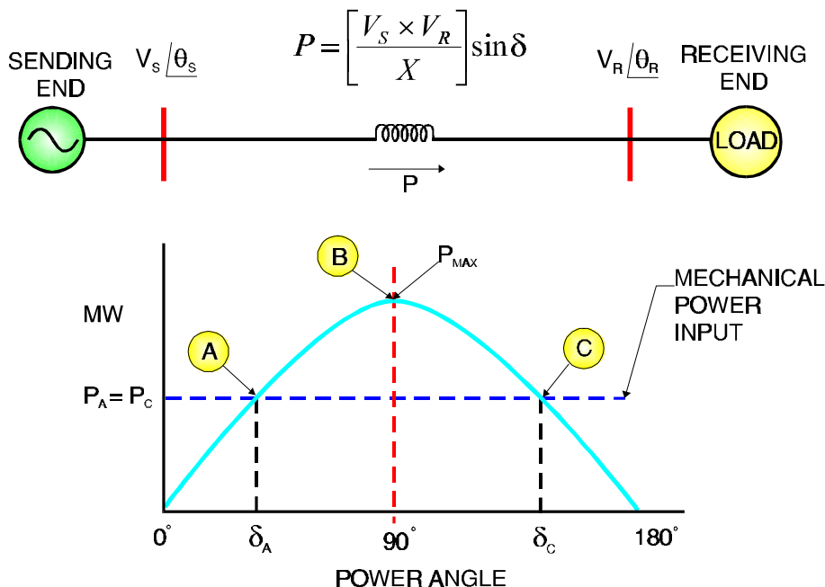
Figure 3-16 The Power-Angle Curve
