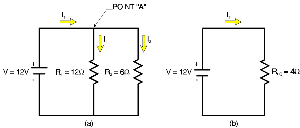
Figure 2-14 Resistors in Series & Parallel
