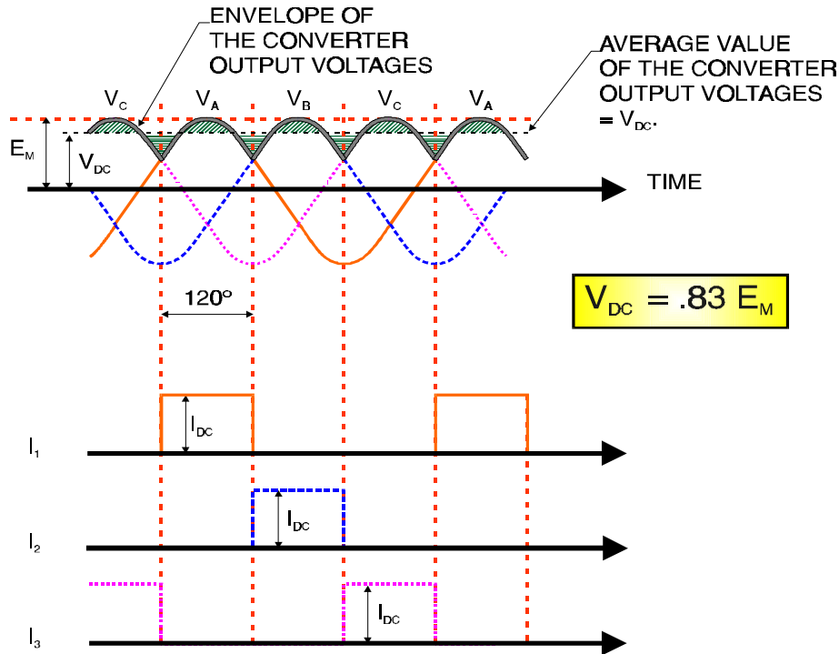
Figure 10-10 Waveforms for 3Φ One-Way Converter
