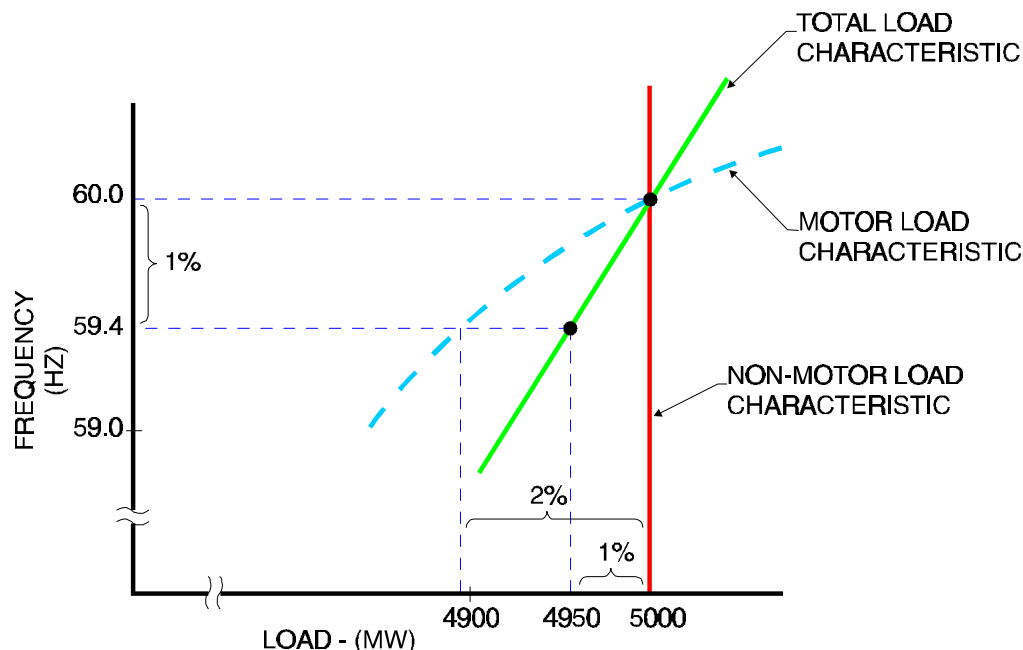
Figure 4-7 Relationship Between Load Magnitude & Frequency
