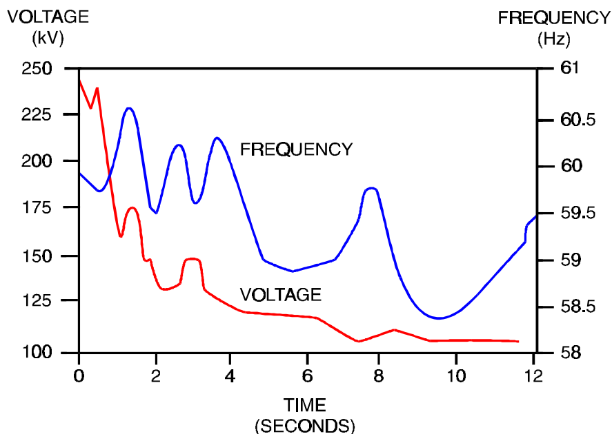
Figure 5-27 Voltage and Frequency Decay
