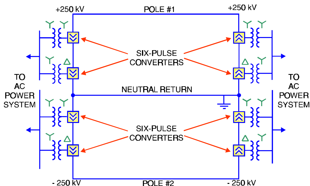
Figure 10-16 A Bipolar HVDC System
