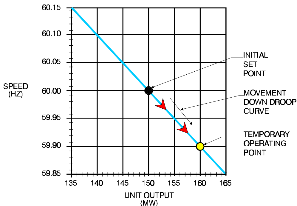
Figure 4-17 300 MW Unit with 5% Droop - Frequency Drop
