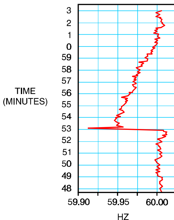
Figure 4-6 Abnormal Frequency Deviations
