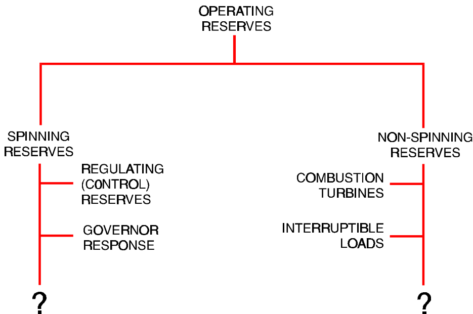
Figure 4-38 Operating Reserves
