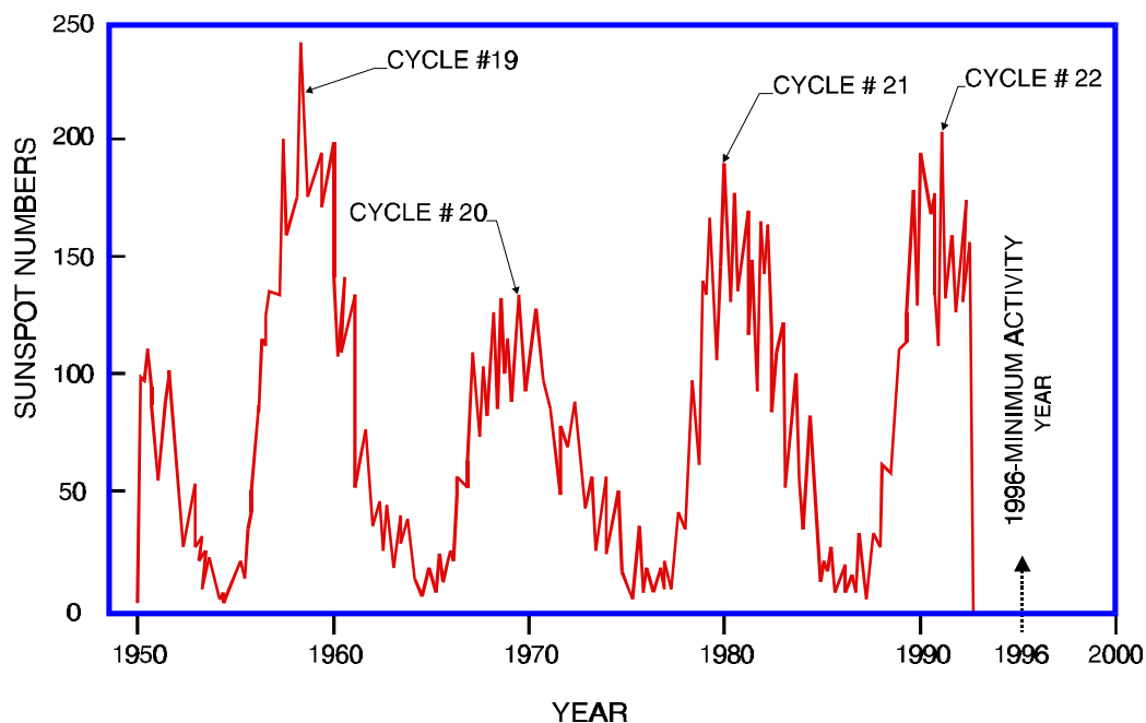
Figure 9-33 Monthly Sunspot Numbers 1950 - Present
