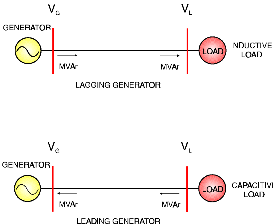
Figure 5-4 Direction of Reactive Power Flow
