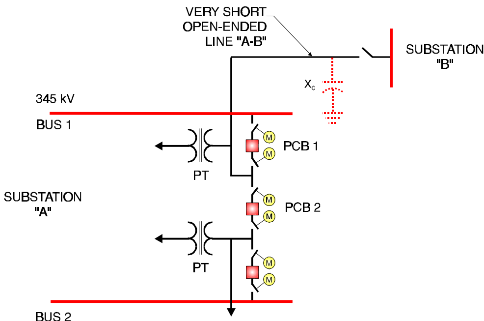
Figure 9-28 One-Line for Transmission System Ferroresonance
