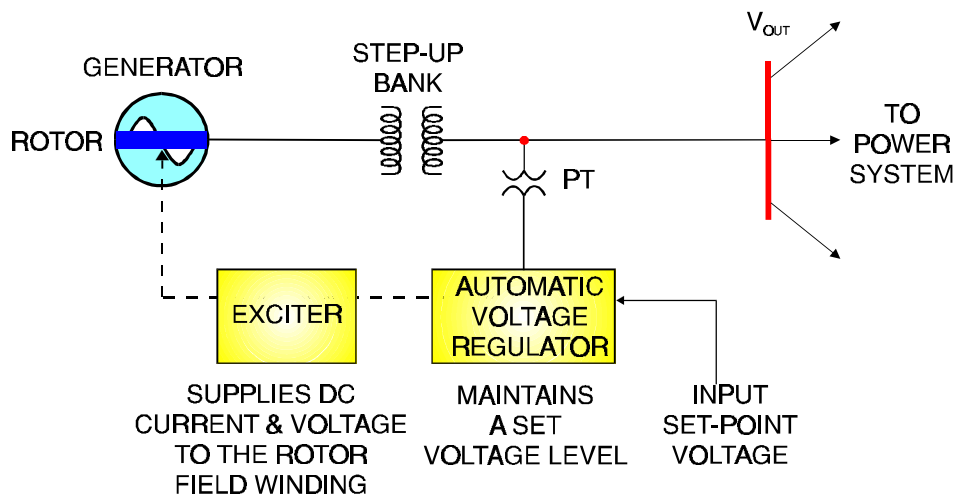
Figure 2-66 Block Diagram of a Generator Excitation System
