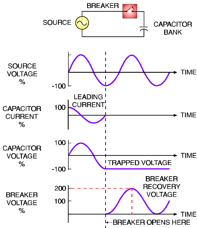
Figure 5-21 Capacitive Switching
